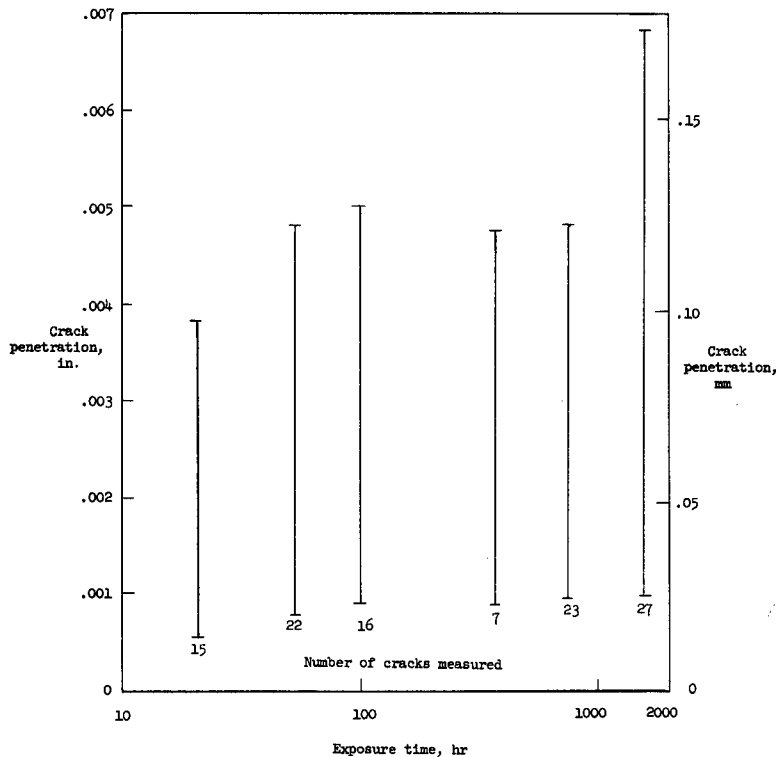
Figure 13.- Depth of crack penetration into residually stressed duplex-annealed Ti-8Al-1Mo-1V alloy sheet after various exposure times at 600° F (589° K) for the 0.25-inch-radius (0.6 cm) specimens.
