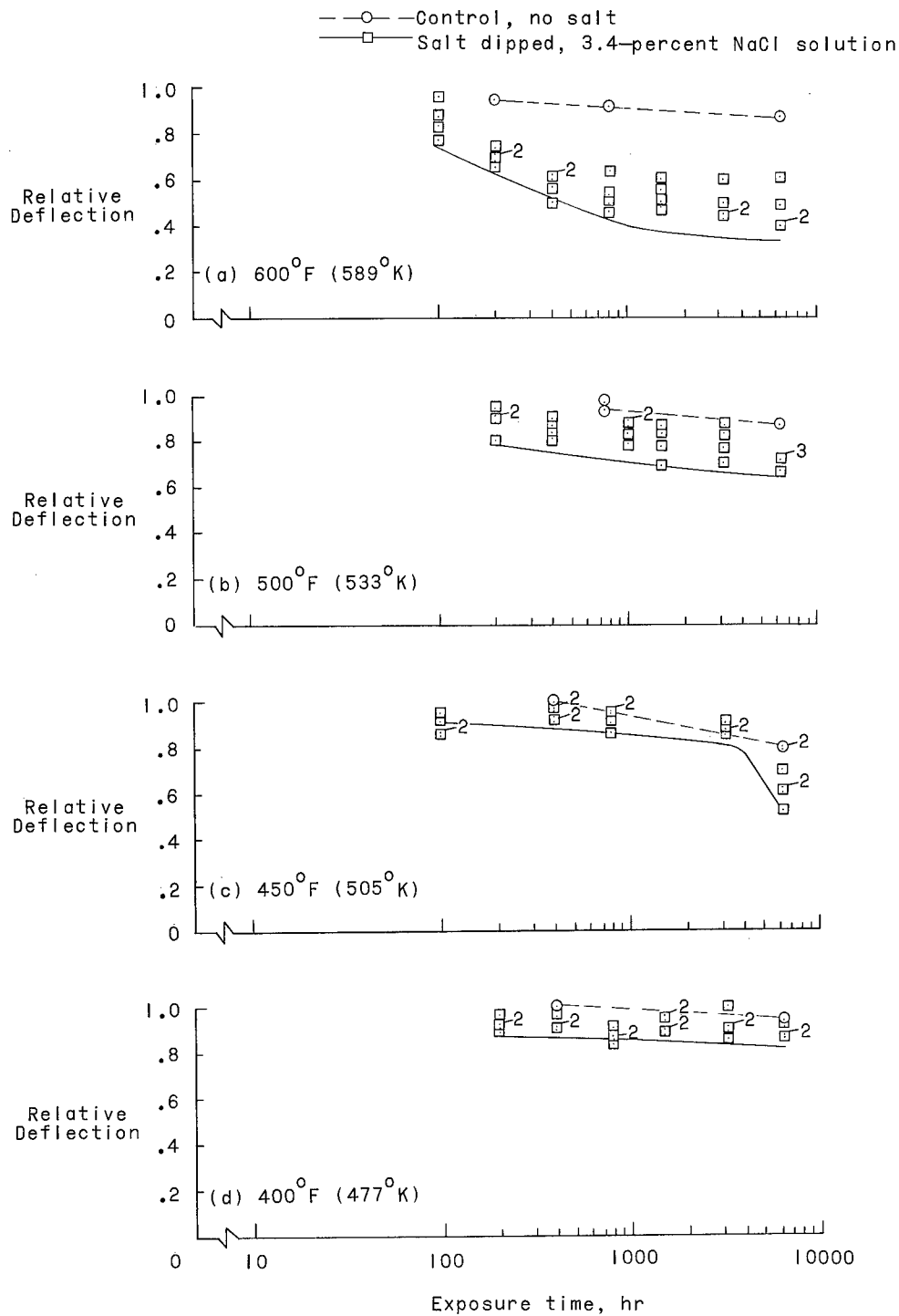
Figure 7.- Effect of various temperatures on salt stress corrosion of duplex-annealed Ti-8Al-1Mo-IV alloy sheet for 1.5-inch-radius (3.8 cm) specimens.
