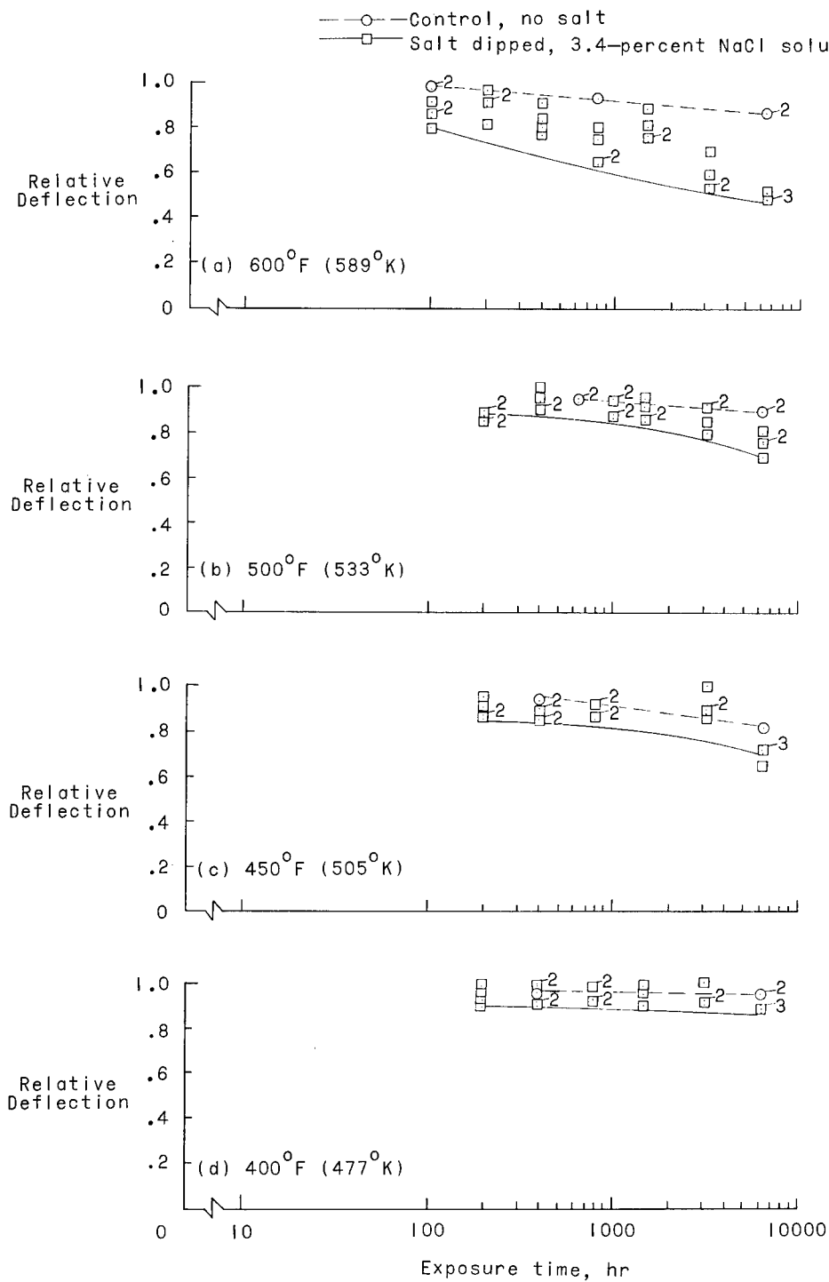
Figure 8.- Effect of various temperatures on salt stress corrosion of duplex-annealed Ti-8Al-1Mo-1V alloy sheet for 2.5-inch-radius (6.4 cm) specimens.
