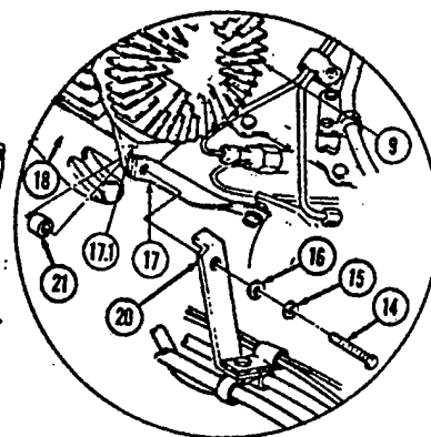
NEW CONFIGURATION
