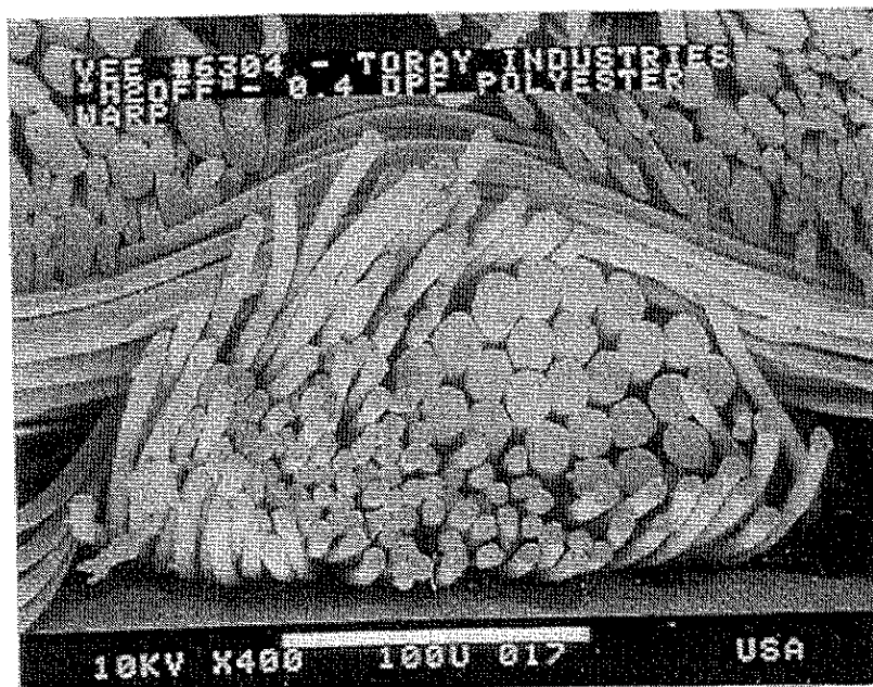
Figure 3. Toray Warp Yarn, Cross-Section
