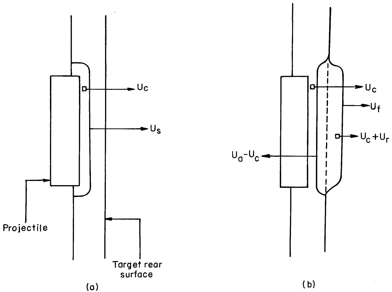
Figure 4.- Conditions produced in target with impact of projectile.
