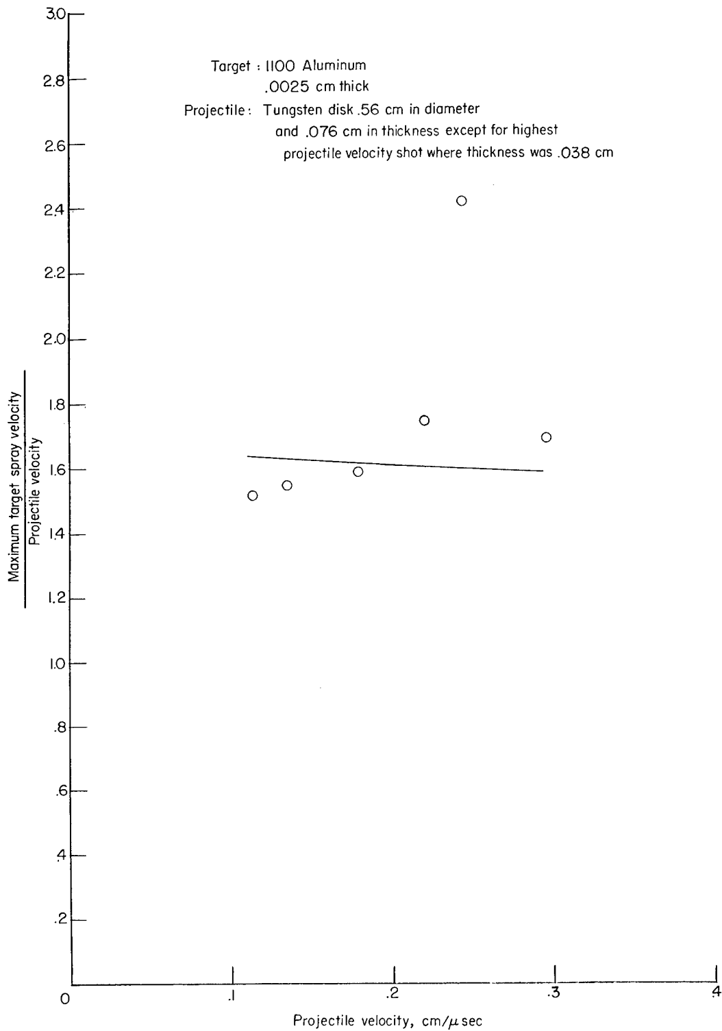
Figure 6.- Comparison of experimental and predicted ratio of maximum target-material spray velocity and projectile velocity with a 1100 aluminum target 0.0025 cm thick.
