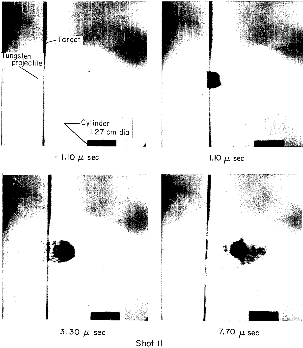
Figure 15.- A tungsten disk 0.56 cm in diameter and 0.076 cm thick impacting a 1100 H14 aluminum target 0.041 cm thick at 0.209 cm/ \mu sec. U_f/U_p = 1.59 .
