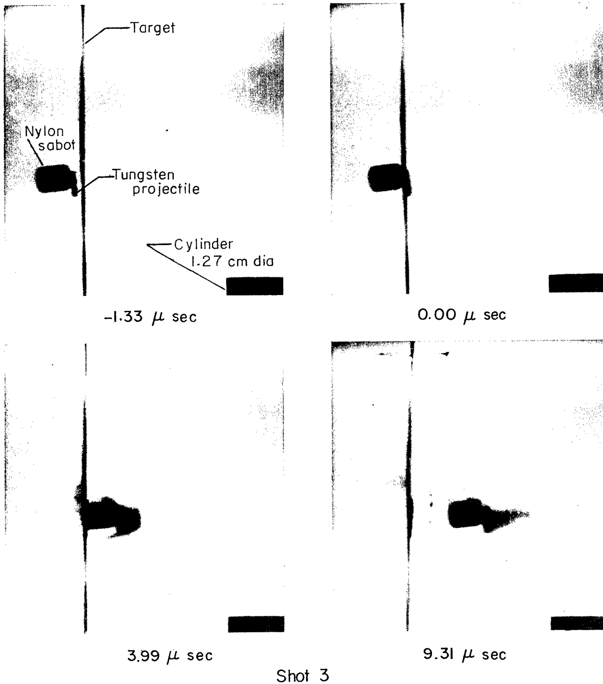
Figure 9.- A tungsten disk 0.56 cm in diameter and 0.076 cm thick impacting a 1100 aluminum target 0.0025 cm thick at 0.179 cm/ \mu\text{sec} . U_i/U_p = 1.59 .
