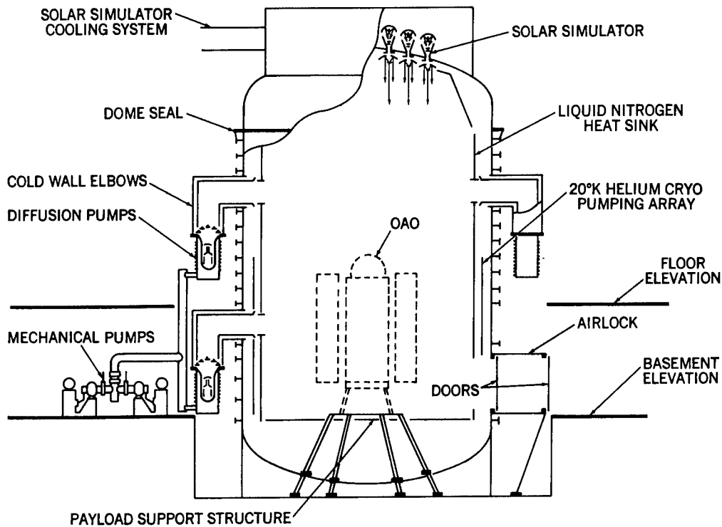
Figure 2—Cross-section of the simulator.
