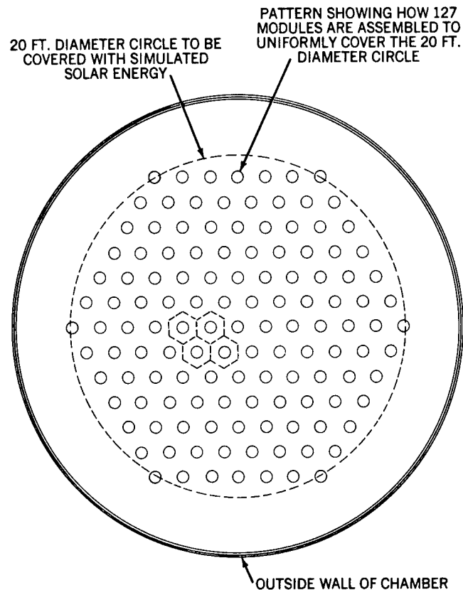
Figure 10—Solar module arrangement.
