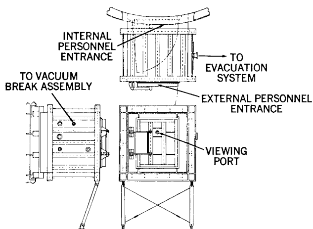
Figure 5—Details of the air lock.
