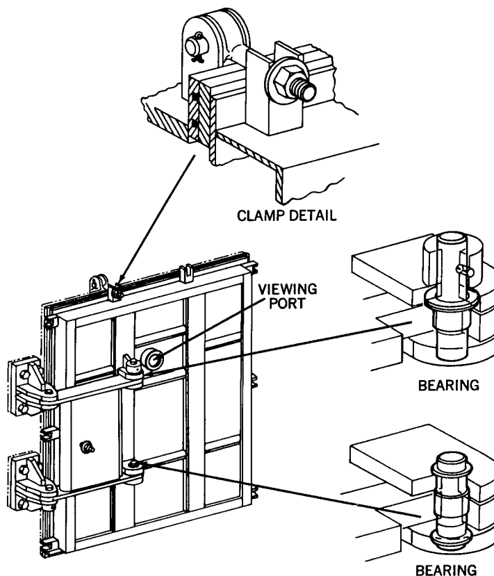
Figure 7—Air lock door.
