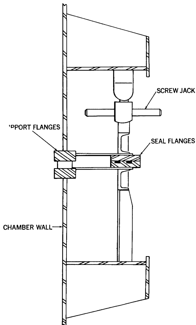
Figure 6—Head seal section.
