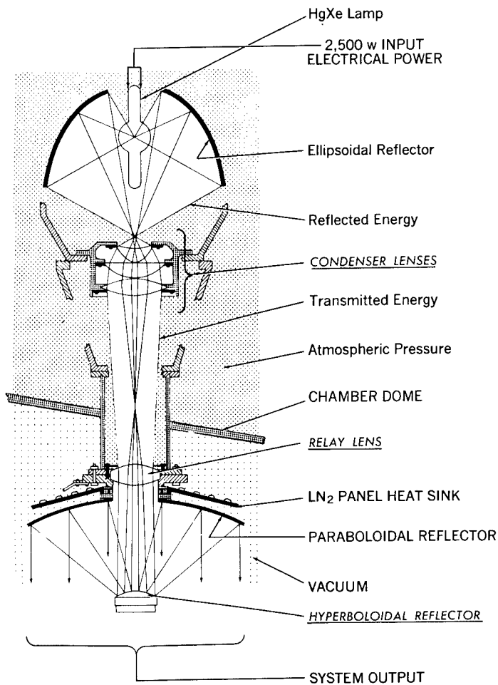
Figure 11—Solar Simulator Module Schematic.
