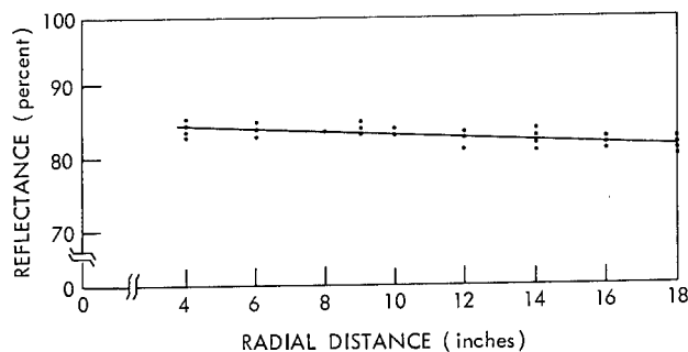
Figure 3 - Reflectance distribution at Lyman alpha.
