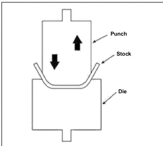
Figure 7. Bending Action
