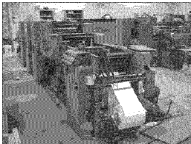
Figure 31. Roll-to-Roll Offset Printing Press
