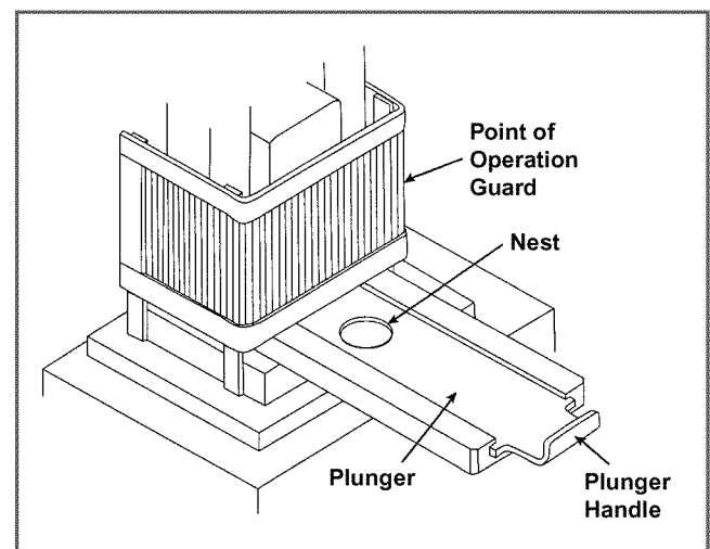
Figure 19. Power Press with Plunger Feed
