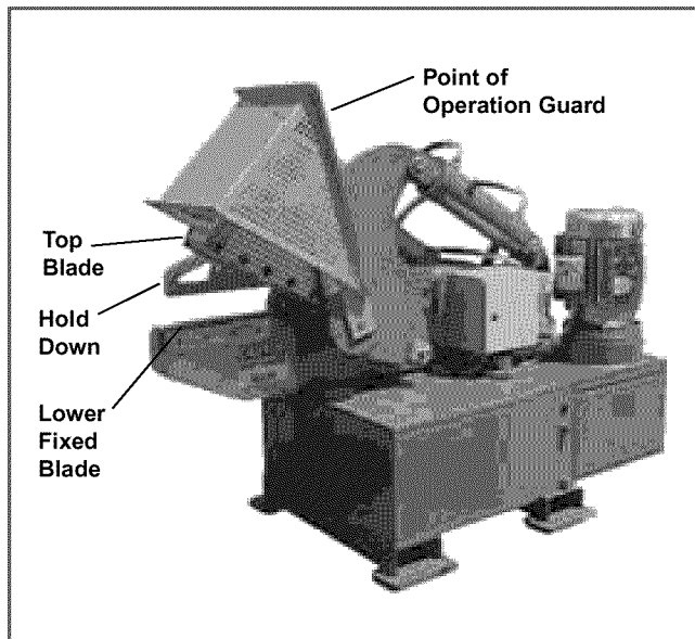
Figure 35. Hydraulic Alligator Shear
