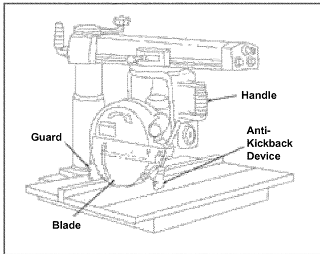
Figure 11. Self-Adjusting Guard on a Radial Saw
