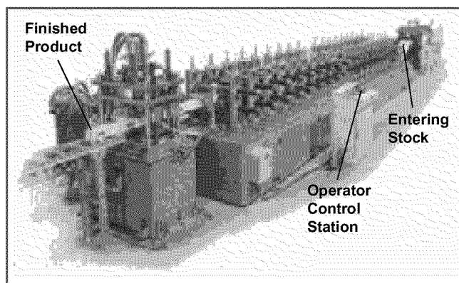
Figure 33. Roll-Forming Machine
