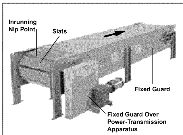
Figure 30. Slat Conveyor
