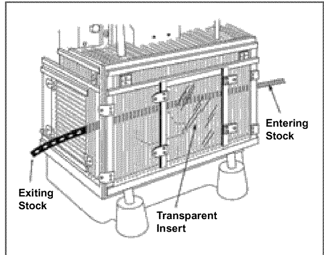
Figure 9. Fixed Guard on a Power Press
