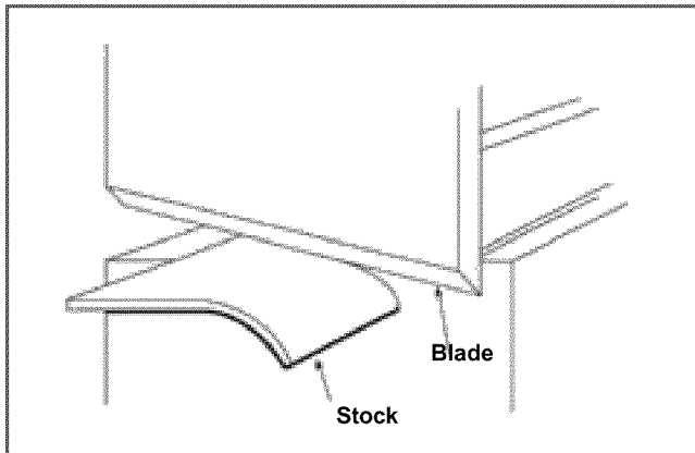
Figure 6. Shearing Action
