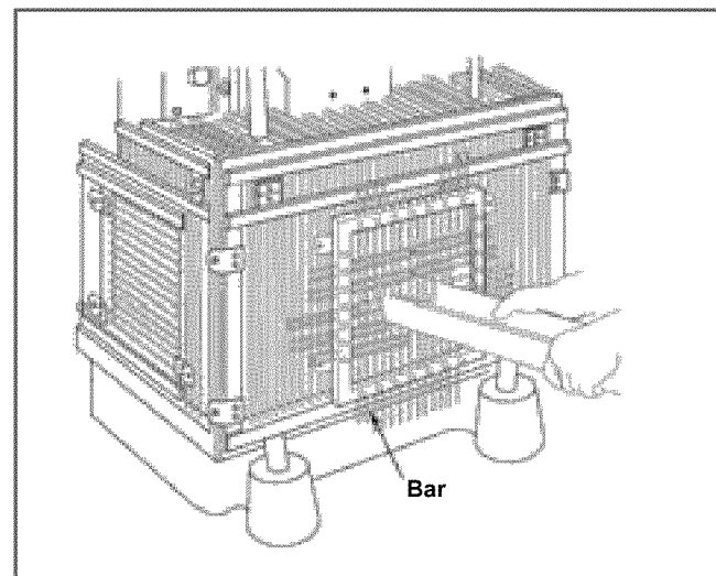
Figure 10. Power Press with Adjustable Barrier Guard
