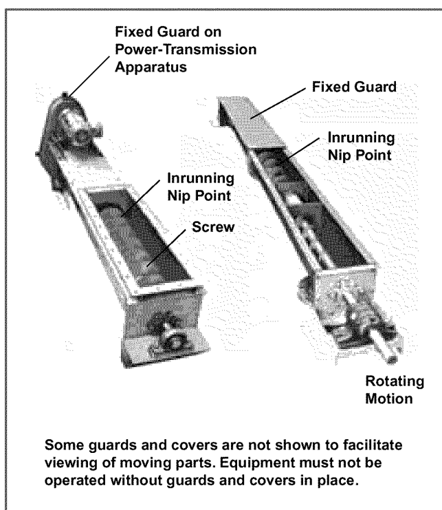
Figure 28. Screw Conveyor
