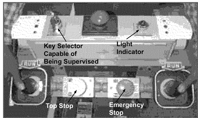
Figure 17. Two-Hand Control
