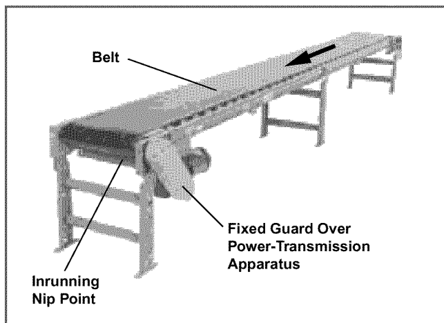
Figure 27. Belt Conveyor
