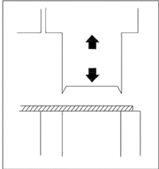
Figure 5. Punching Action
