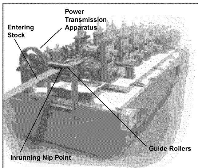
Figure 34. Infeed Area of a Roll-Forming Machine
