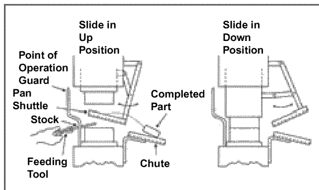
Figure 20. Shuttle Ejection Mechanism
