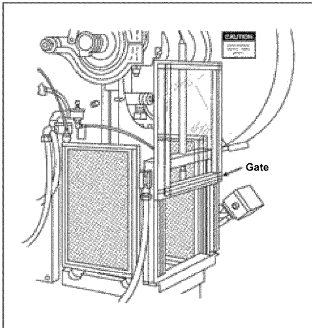
Figure 18. Power Press with Gate
