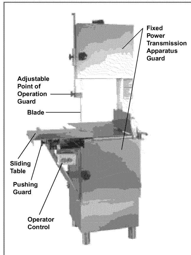
Figure 39. Stainless Steel Meat-Cutting Band Saw
