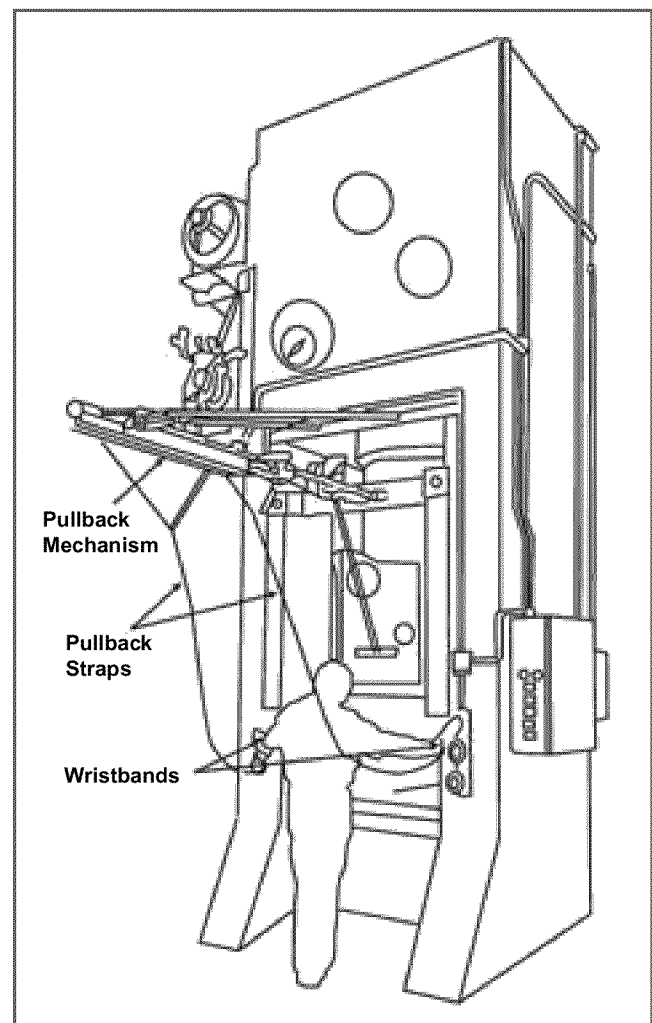
Figure 13. Pullback Device on a Power Press
