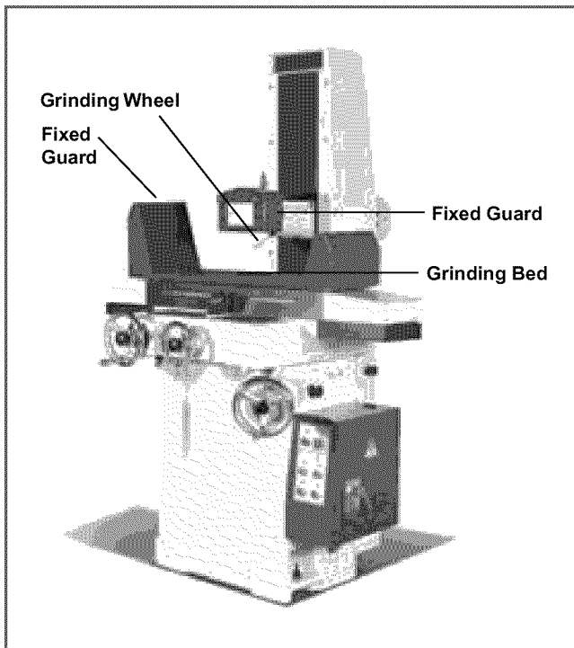
Figure 42. Horizontal Surface Grinder
