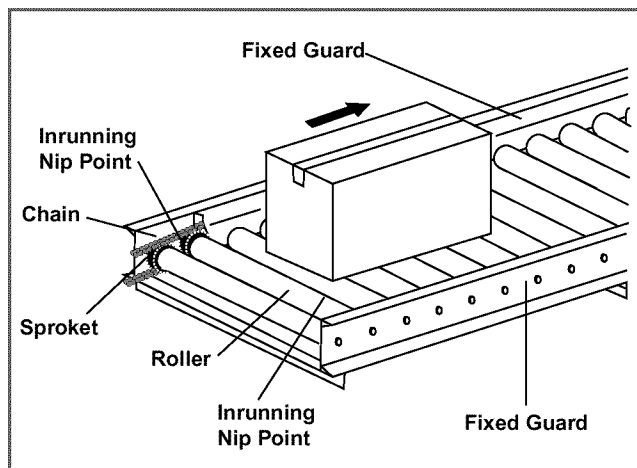
Figure 29. Chain Driven Live Roller Conveyor
