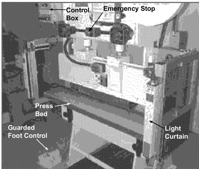
Figure 15. Presence Sensing Device on a Power Press
