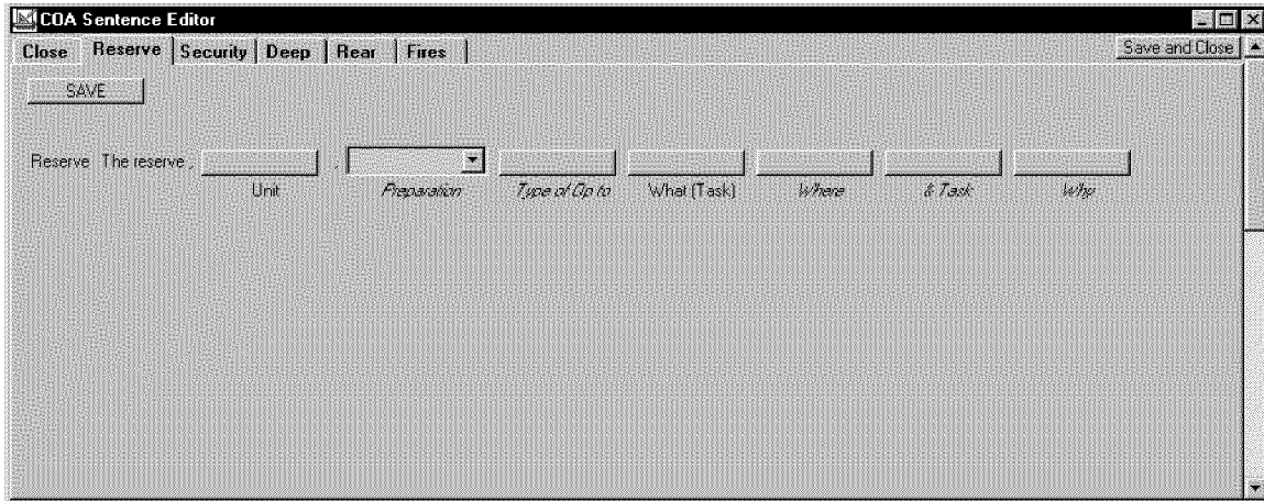
Figure 7.2. COA Statement window, showing template for Reserve statements.
