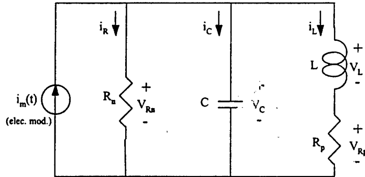
Figure V.2 Small signal circuit model of a single mode laser with electrical modulation.
