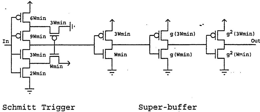
Figure III.14: Digital buffer.
