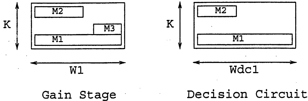
Figure III.21: Layout floorplan of receiver gain stage and decision circuit.
