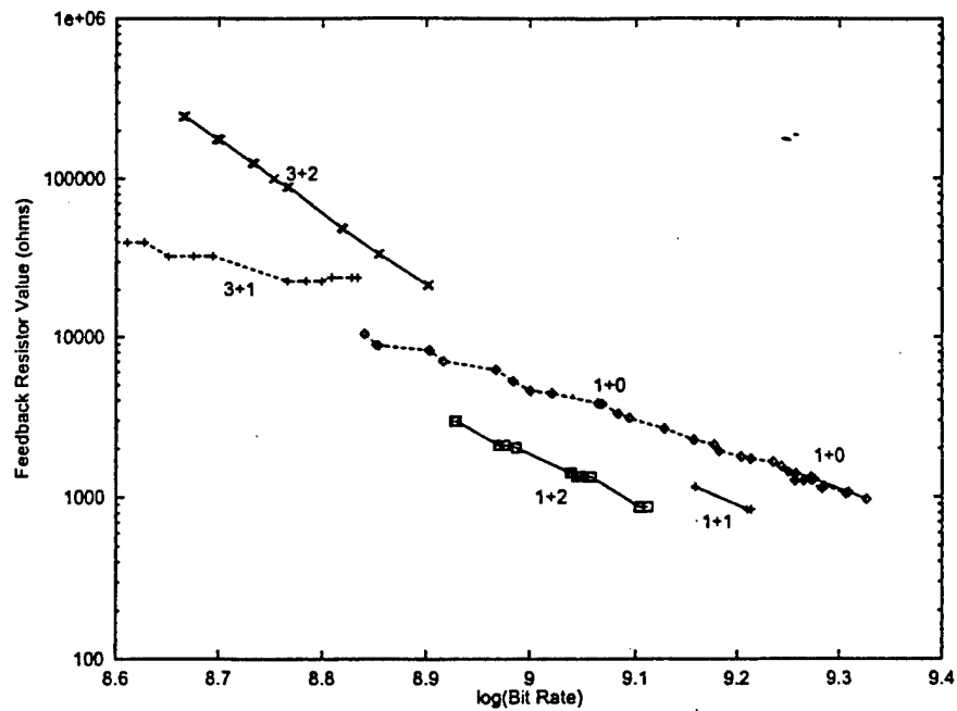
Figure III.42: Feedback resistor values for optimized receivers in 0.35\ \mu\text{m} CMOS. The solid line is for receivers optimized for minimum optical power, and the dashed line is for receivers optimized for total power.
