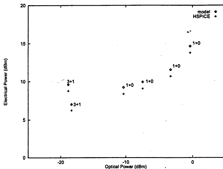
Figure III.48: Comparison of HSPICE results and model of electrical power dissipation versus optical power requirement, for receivers optimized for total power in 0.35 \mu\text{m} CMOS.
