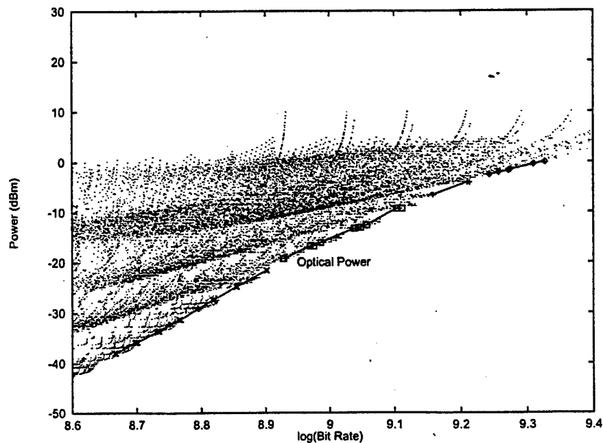
Figure III.38: Scatter plot of receiver performance, across the range of parameters, for L=0.35 \mu m CMOS. Optimum performance is at the right edge of the diagram.
