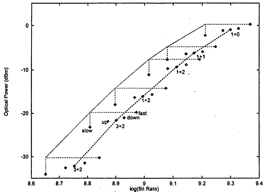
Figure III.34: Plot of optical power requirement versus bit-rate, showing performance at all four process corners, for receivers optimized for optical power in 0.35\ \mu\text{m} CMOS. Worst case optical power and bit-rate combination is also graphed.
