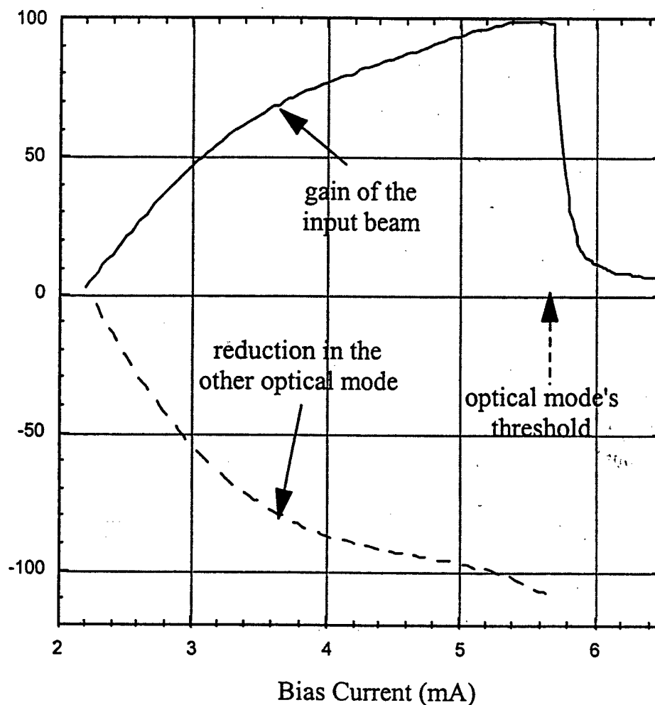
Figure V.10 Steady state cavity gain vs. bias current for 2.7 \mu W input light intensity.
