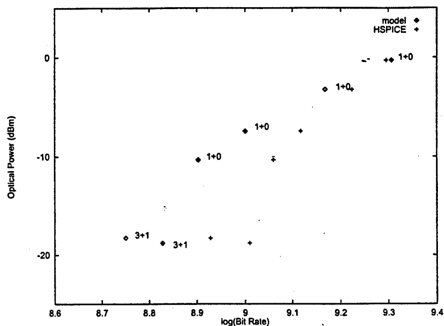
Figure III.50: Comparison of HSPICE results and model of optical power versus bit-rate, for receivers optimized for total power in 0.35\ \mu\text{m} CMOS.
