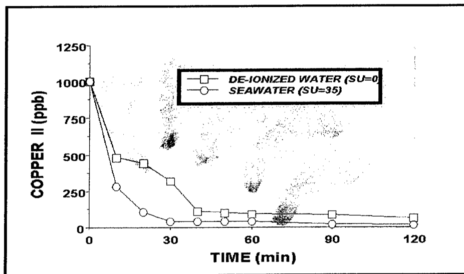
Figure 17. Loss of Cu(II) in 2 types of water with the addition of 1g of Chitosan. SU=salinity units=ppt(parts per thousand).
