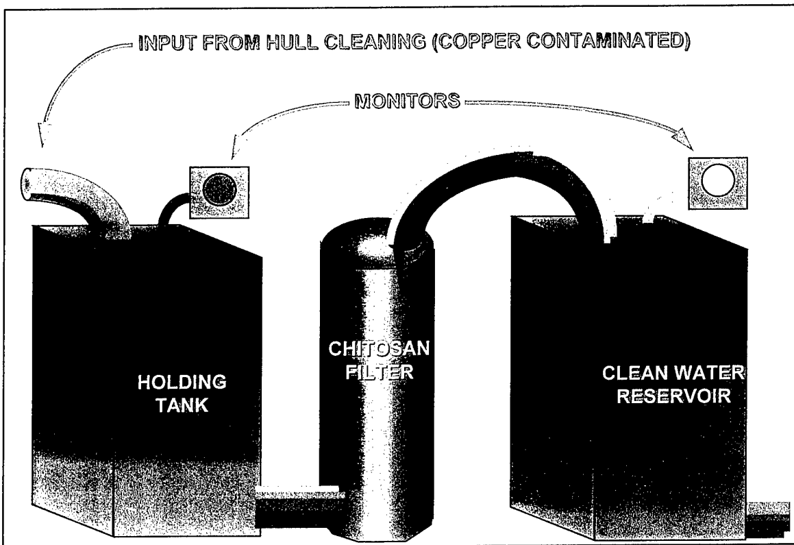
Figure 20. Conceptual model of a waste copper handling facility.
