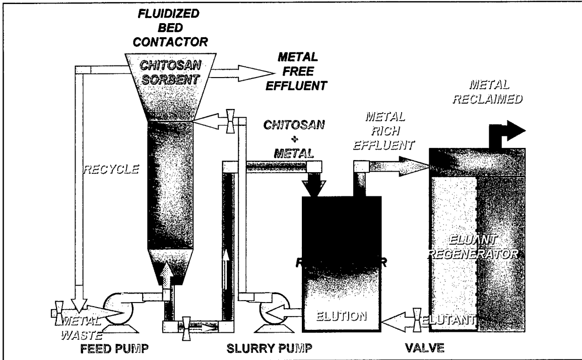
Figure 21. Conceptual model of a fluidized bed reactor for cleaning and recycling copper contaminated water.
