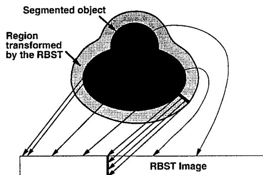
FIG. 3. An illustration of the RBST. The pixels along the object boundary are mapped to the first row of the RBST image. Pixels along a normal to the object boundary are mapped to a column of the RBST image.
