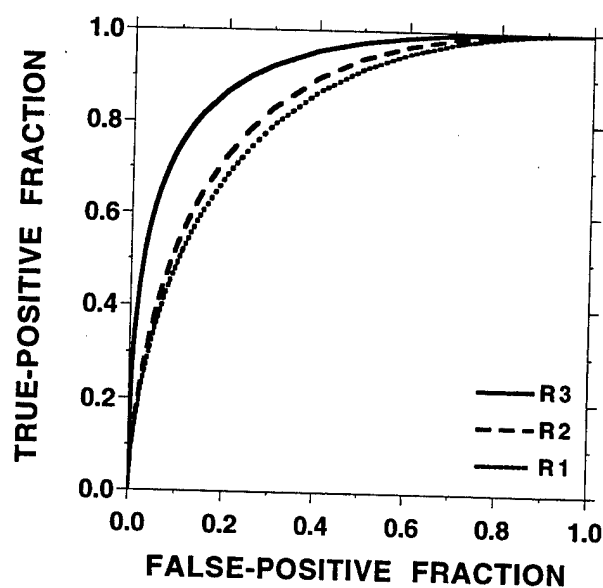
Figure 7: ROC curves for the three image representations using the combined feature space.
