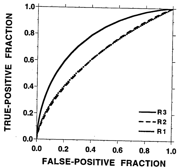
Figure 6: ROC curves for the three image representations using the RLS feature space.
