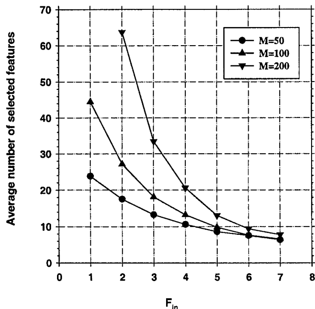
FIG. 6. Case 1 (identity covariance matrix), A_z(\infty)=0.89 . Feature selection from the entire sample space of 100 samples/class: The number of features selected in stepwise feature selection versus F_{in} ( F_{out}=F_{in}-1 ).
