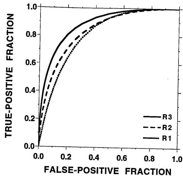
Figure 5: ROC curves for the three image representations using the SGLD feature space.
