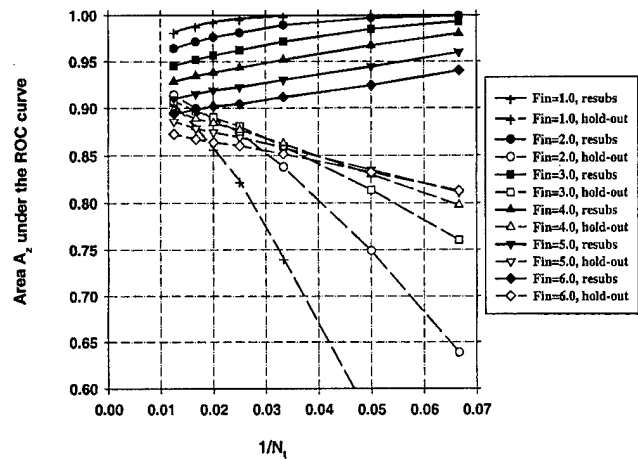
FIG. 4. Case 1 (identity covariance matrix), A_z(\infty)=0.89 . Feature selection from the entire sample space of 100 samples/class: The area A_z under the ROC curve versus the inverse of the number of design samples N_i per class. Feature selection was performed using an input feature space of M=100 available features.
