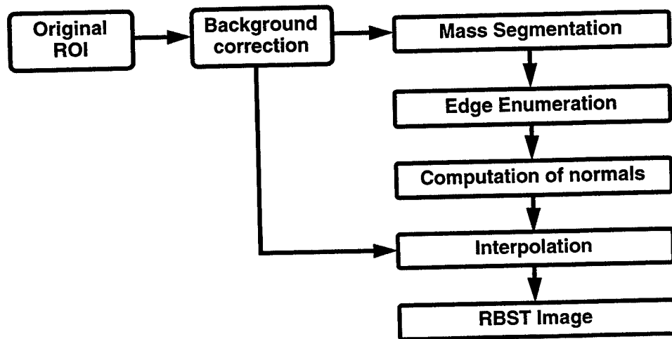
Figure 3: Block diagram of the computation of an RBST image.
