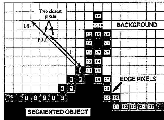
FIG. 6. Computation of RBST pixel values. p(i,j) has a distance j from the pixel i along the normal line L(i) . The (i,j) th pixel value in the RBST image is a distance-weighted average of the two closest pixels to p(i,j) .
