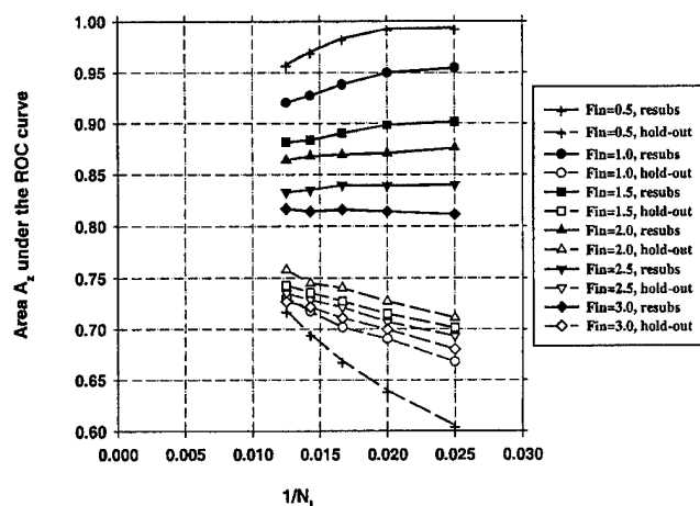
FIG. 17. Case 3(a) (an example from CAD, no diagonalization), A_z(\infty) = 0.86 . Feature selection from the design samples. Total sample size N_s = 100 samples per class. The area A_z under the ROC curve versus the inverse of the number of design samples N_i per class. Feature selection was performed using an input feature space of M = 100 available features.
