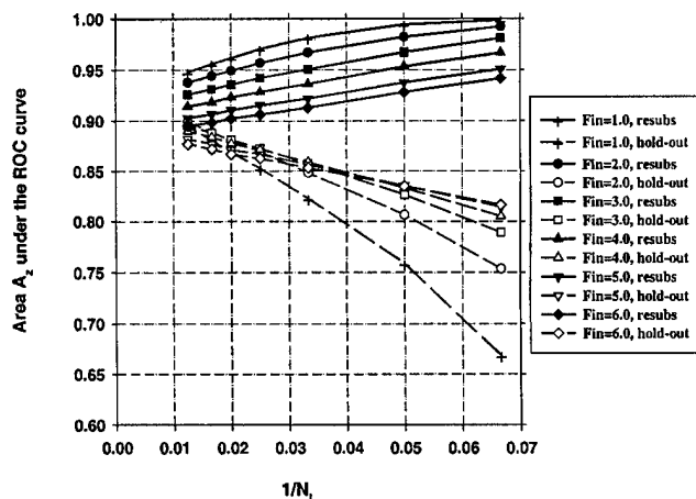
FIG. 3. Case 1 (identity covariance matrix), A_z(\infty)=0.89 . Feature selection from the entire sample space of 100 samples/class: The area A_z under the ROC curve versus the inverse of the number of design samples N_i per class. Feature selection was performed using an input feature space of M=50 available features.
