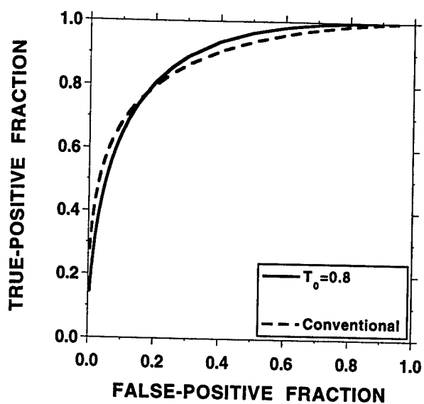
Figure 1. ROC curves for neural networks with 2 hidden layer nodes
