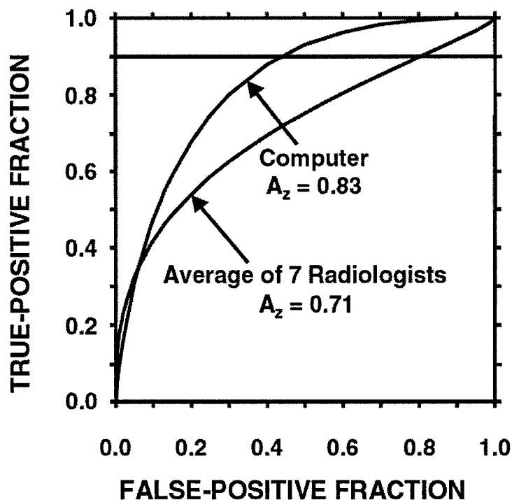
Figure 2. The average ROC curve of the 7 radiologists for the classification of mammographic microcalcifications a malignant or benign and the ROC curve of the computer classifier.
