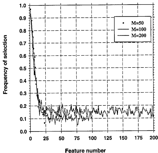
FIG. 7. Case 1 (identity covariance matrix), A_z(\infty)=0.89 . Feature selection from the entire sample space of 100 samples/class: The frequency of feature number i , defined as the fraction of experiments in which feature i was selected. F_{in}=3.0 , F_{out}=2.0 .
