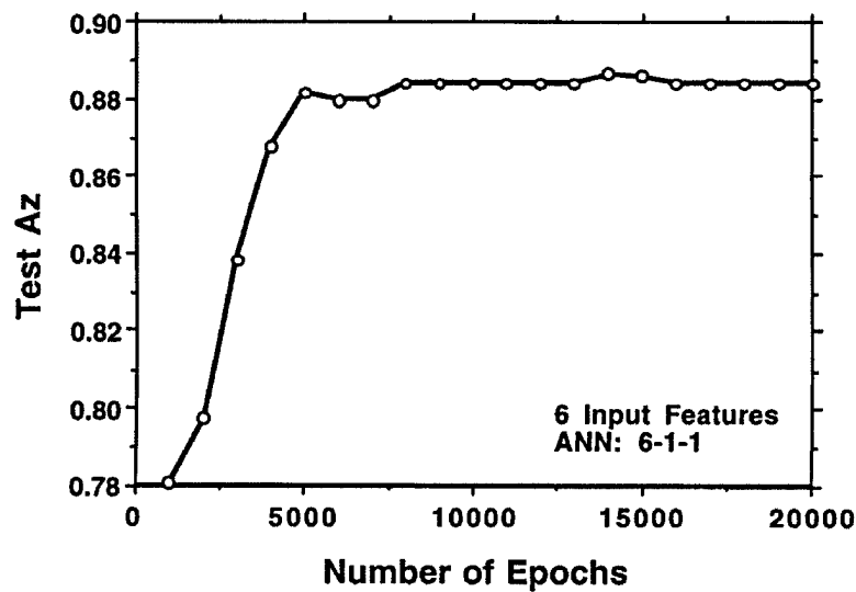
Figure 4. An example demonstrating the dependence of test A_z on the number of training epochs. The test A_z generally increased rapidly during the first 5000 epochs and then gradually reached a plateau or a broad maximum.
