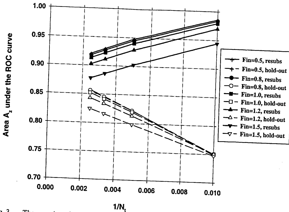
Fig. 3 The area A_z under the ROC curve versus the inverse of the number of design samples N_t per class for Case 1.a, feature selection from the entire sample space of 500 samples/class. Feature selection was performed using an input feature space of M=100 available features. A_z(\infty)=0.89 .
