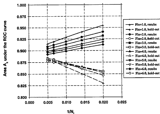
FIG. 8. Case 1 (identity covariance matrix), A_z(\infty)=0.89 . Feature selection from the entire sample space of 250 samples/class: The area A_z under the ROC curve versus the inverse of the number of design samples N_i per class. Feature selection was performed using an input feature space of M=50 available features.
