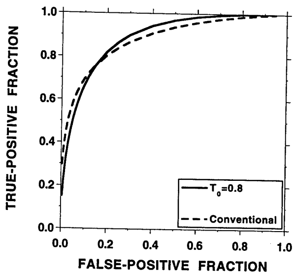
Figure 2. ROC curves for neural networks with 3 hidden layer nodes
