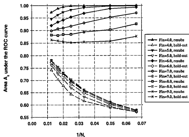
FIG. 11. Case 1 (identity covariance matrix), A_z(\infty)=0.89 . Feature selection from the design samples. Total sample size N_s=100 samples per class. The area A_z under the ROC curve versus the inverse of the number of design samples N_i per class. Feature selection was performed using an input feature space of M=200 available features.
