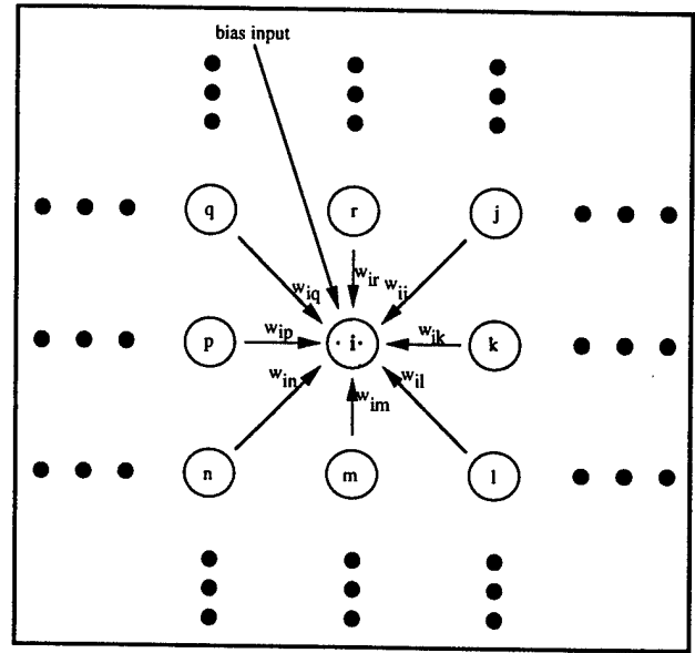
Figure 1. General architecture of a Hopfield neural network.
