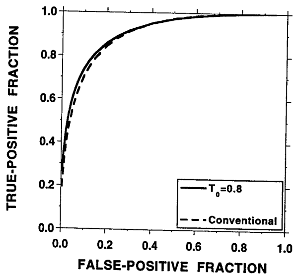
Figure 4. ROC curves for neural networks with 9 hidden layer nodes
