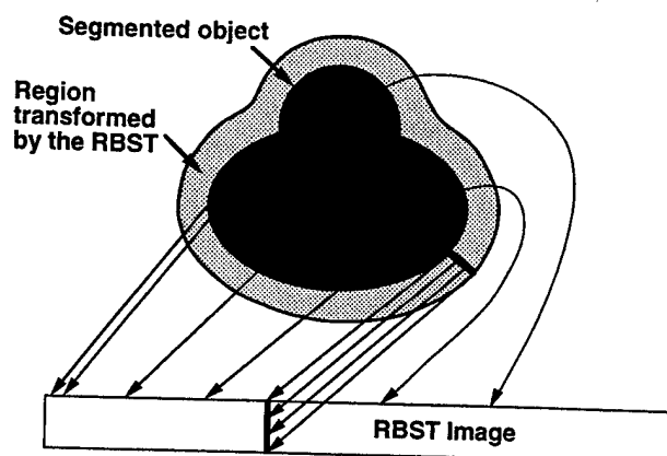
Figure 2: The rubber band straightening transform (RBST). The pixels along the object boundary are mapped to the first row of the RBST image. Pixels on a normal line to the object are mapped to a column of the RBST image.
