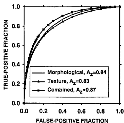
FIG. 10. ROC curves for classification of masses in the morphological, texture, and combined feature spaces.
