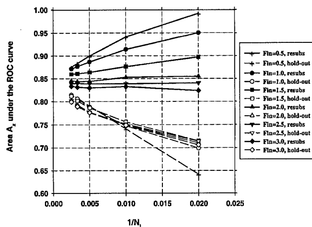
FIG. 18. Case 3(a) (an example from CAD, no diagonalization), A_z(\infty) = 0.86 . Feature selection from the design samples. Total sample size N_s = 500 samples per class. The area A_z under the ROC curve versus the inverse of the number of design samples N_i per class. Feature selection was performed using an input feature space of M = 100 available features.
