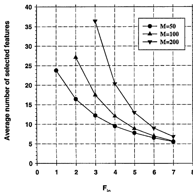
FIG. 12. Case 1 (identity covariance matrix), A_z(\infty)=0.89 . Feature selection from N_i=80 design samples per class. Total sample size N_s=100 samples per class. The number of features selected in stepwise feature selection versus F_{in}(F_{out}=F_{in}-1) .
