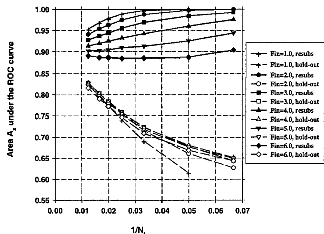
FIG. 9. Case 1 (identity covariance matrix), A_z(\infty)=0.89 . Feature selection from the design samples. Total sample size N_s=100 samples per class. The area A_z under the ROC curve versus the inverse of the number of design samples N_i per class. Feature selection was performed using an input feature space of M=50 available features.
