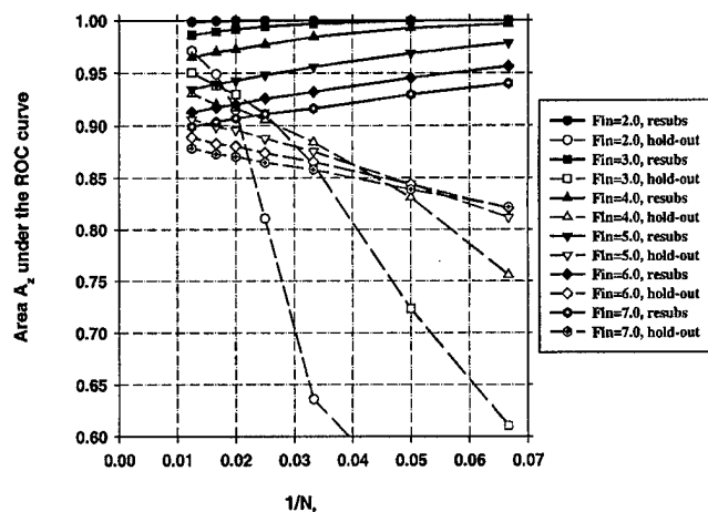
FIG. 5. Case 1 (identity covariance matrix), A_z(\infty)=0.89 . Feature selection from the entire sample space of 100 samples/class: The area A_z under the ROC curve versus the inverse of the number of design samples N_i per class. Feature selection was performed using an input feature space of M=200 available features.
