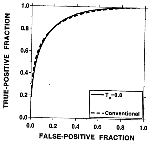
Figure 3. ROC curves for neural networks with 5 hidden layer nodes
