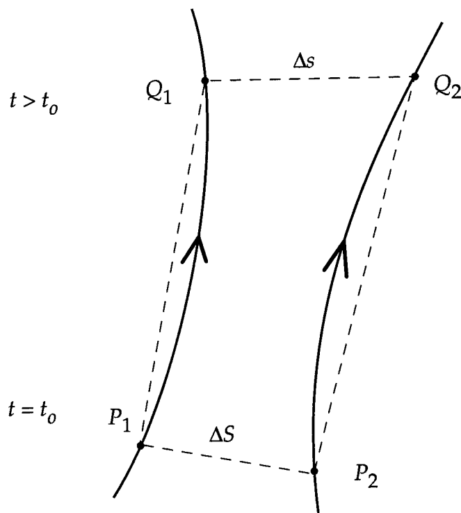
Figure 3. The position P_1 and P_2 of two particles is shown in the reference configuration at t = t_0 , and the positions Q_1 and Q_2 of the same two particles is shown at later time t > t_0 . The path of the particles is shown in solid lines and their displacement is shown in dashed lines.
