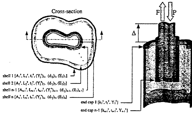
Figure 1. General Telescopic Actuator Architecture: A depiction of a general telescopic actuator composed of n shells and n-1 end caps.
