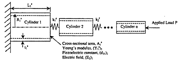
Figure 3. Telescopic Analytical Model: The telescopic actuator is modeled as discrete cylinders connected by end caps modeled as springs.
