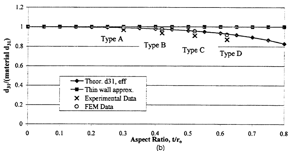
Figure 8. Single fiber prototype free strain. The slope of the strain/field curve yields the effective d_{31} : (a) shows the strain of a single prototype (aspect ratio = 0.42) and (b) plots the effective d_{31} as a function of aspect ratio. The error between theory and measured values of effective d_{31} ranged from approximately 3 to 9 percent. FEM models match theory within one percent.
