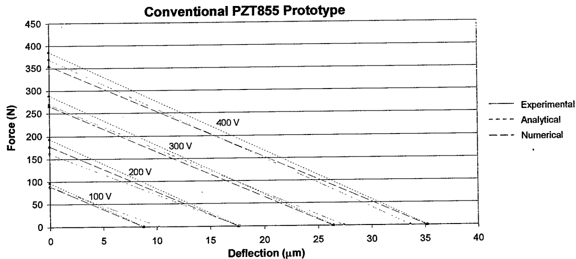
Figure 19: Force-Deflection results
