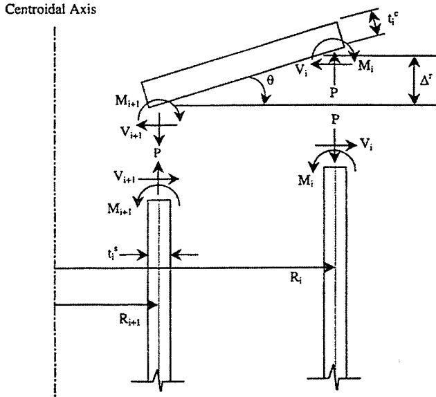
Figure 4. Compliant End Cap Model: Shown is a compliant end cap connection between two piezoelectric cylinders and the resulting forces and moments.
