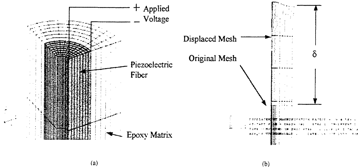
Figure 10. Lamina finite element model. The deflection of a single fiber was modeled using ABAQUS as a solver and Hypermesh as a pre- and post-processor. (a) Hypermesh model and (b) ABAQUS results.
