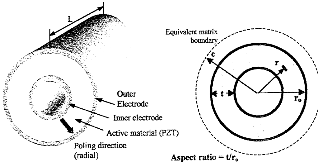
Figure 1. Hollow fiber design. The basic fiber design consists of a hollow cylinder of active material, electroded on both the inside and outside surfaces. In the case of piezoelectric material (PZT), the poling direction is radial; therefore the d_{31} response of the fiber is used to create longitudinal motion.
