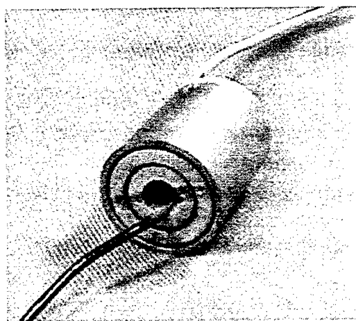
Figure 6 Finished actuator—after poling, electroding, and wiring.
