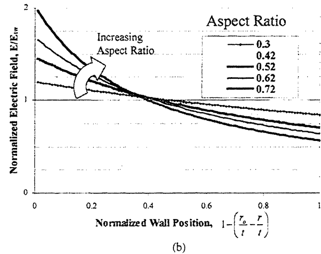
Figure 2. Electric field in thick wall fibers. As the aspect ratio of a hollow fiber increases, the difference between the maximum and minimum electric fields increases. The highest field occurs at the inside wall; the lower field at the outside wall. (a) Normalized field vs. aspect ratio and (b) field vs. normalized wall position.
