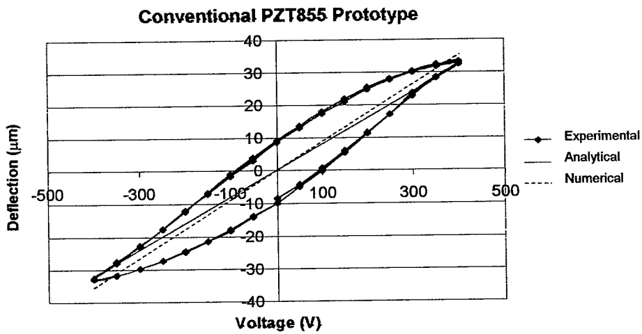
Figure 21: Deflection-Voltage results
