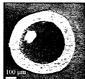
Figure 4. Hollow fiber prototype. Cross-section of coextruded fiber following the burnout/sintering process. Outside radius = 300 μm; thickness = 90 μm.
