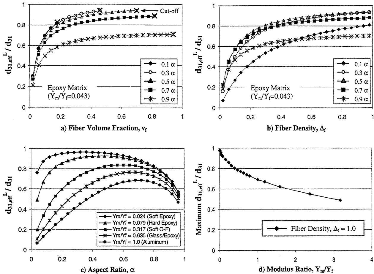
Figure 4. PZT / Epoxy Effective Lamina d_{31} . a) The effective lamina d_{31} normalized by material d_{31} ( d_{31,eff}^L / d_{31} ) was plotted as a function of volume fraction for several aspect ratios. b) The normalized effective lamina d_{31} was plotted as a function of fiber density. The largest lamina d_{31} was 94% of the material d_{31} , corresponding to 254 pm/V for PZT-5H, for fiber aspect ratios from approximately 0.3 to 0.5. c) The normalized effective lamina d_{31} (calculated at maximum fiber density) was plotted as a function of aspect ratio for several modulus ratios. d) The maximum value of the normalized effective lamina d_{31} was plotted versus the modulus ratio and varied from 0.96 for very soft epoxy to 0.48 for steel.
