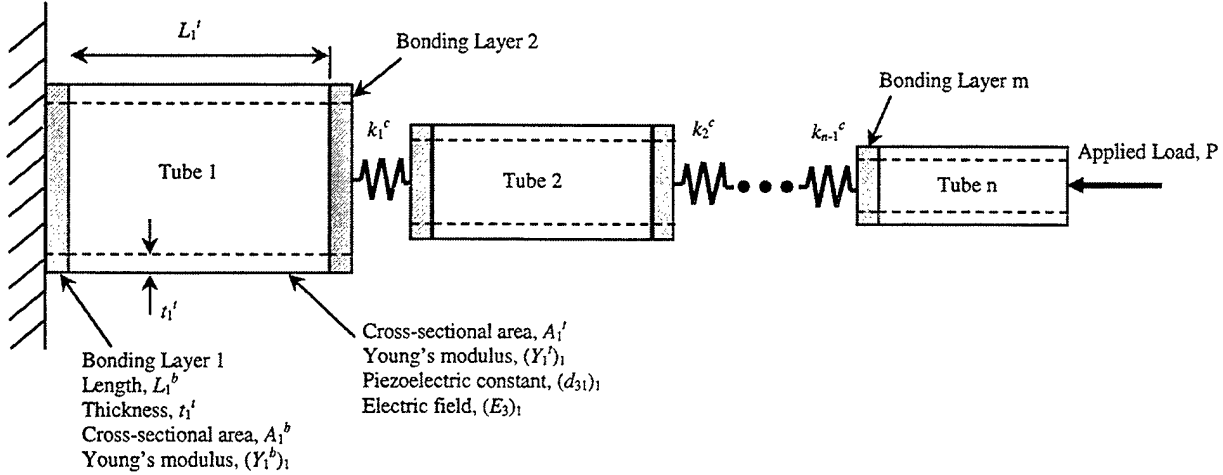
Figure 7: Revised analytical model of the telescopic architecture
