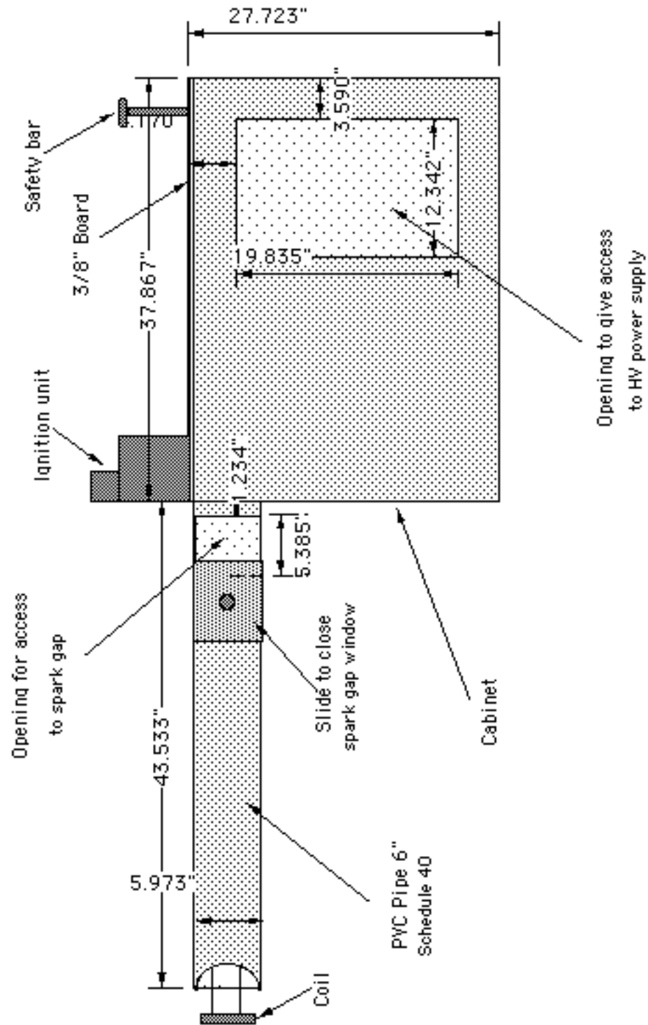
Figure II-6. Drawing of One Unit
