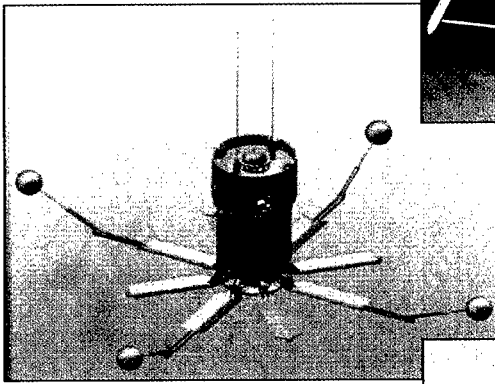
Air-Deliverable Acoustic Sensor (ADAS)
