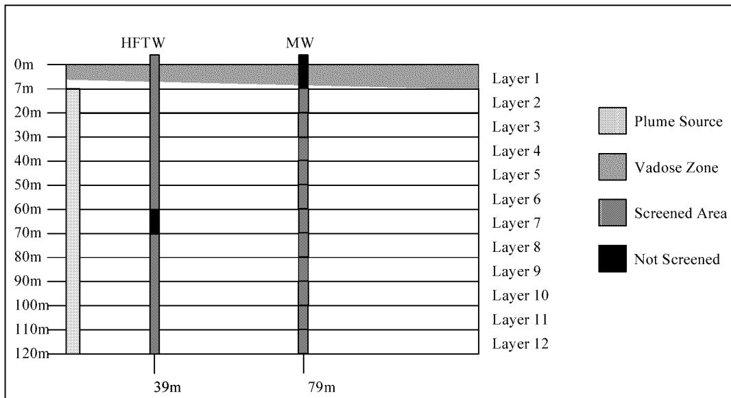
Figure 3.5b: Section A-A
