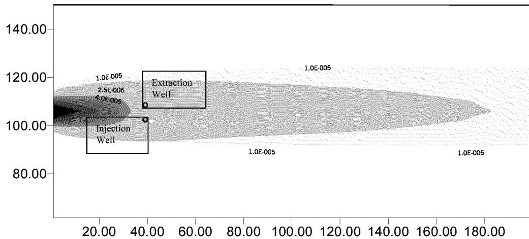
Figure 4.14: Concentration contours ( \text{mg/m}^3 ) in layer 6 at 50,000 days. Note that the contaminant plume bypasses the capture zone of the HFTW system, and is transported downgradient
