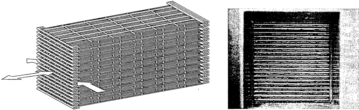
Figure 4. Assembled anisotropic stack/heat-exchanger unit, in schematic form (with acoustic gas motion and heat exchanger fluid motion indicated), and an end view photograph of an actual ASHE unit.
