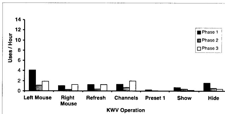
Figure 35. KVV software use on the FCC K-Desk.
