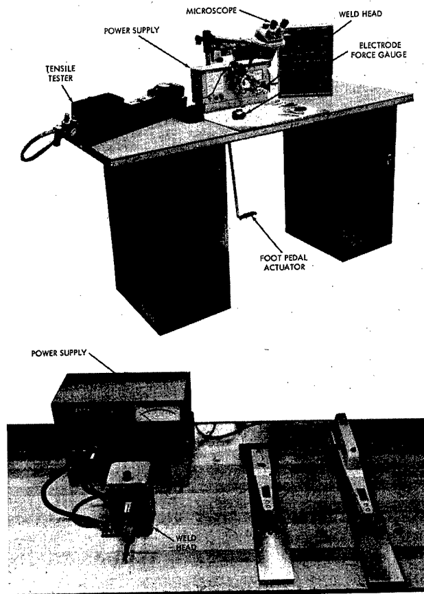
Figure 3—Shop equipment.
