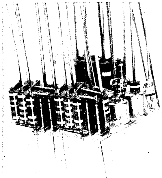
Figure 12—Submodule-transistor assembly.
