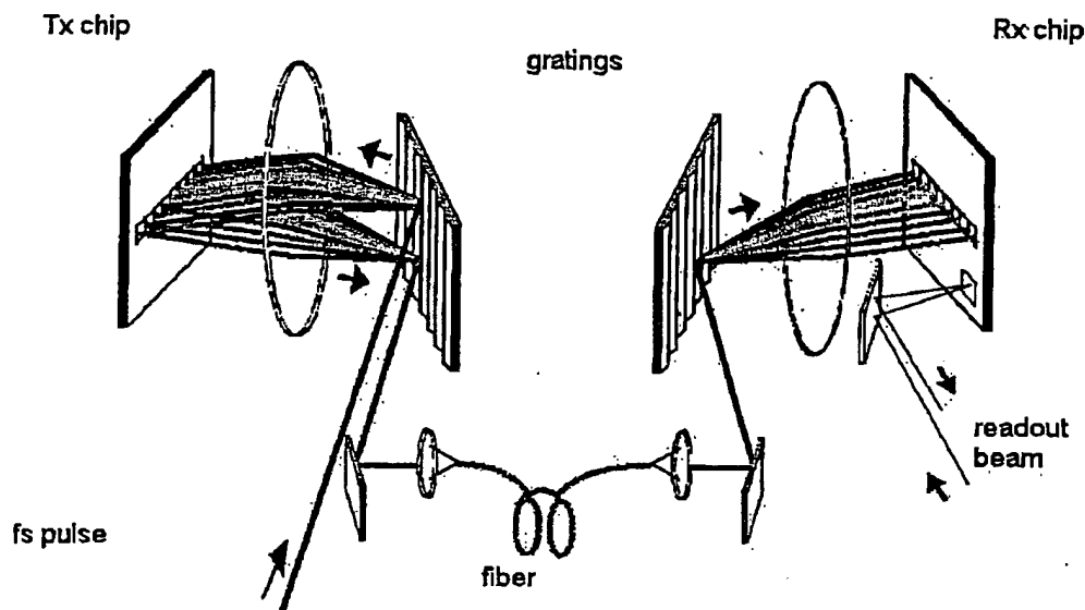
Figure 6: Schematic representation of WDM optical link
