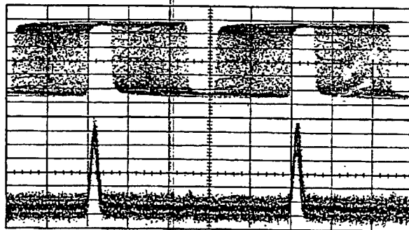
Figure 16. Demonstration of jitter removal from a single interconnect channel, at a clock rate of 82 MHz. Upper trace is the electrical input signal; lower trace is the receiver circuit optical readout
