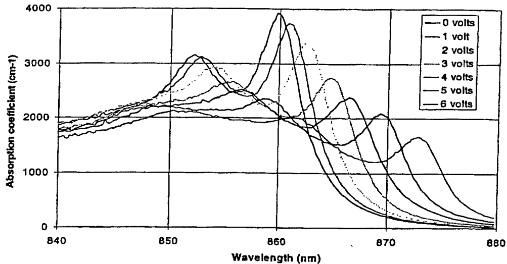
Figure 2: Plot of the absorption spectrum of modulator at different voltage bias
