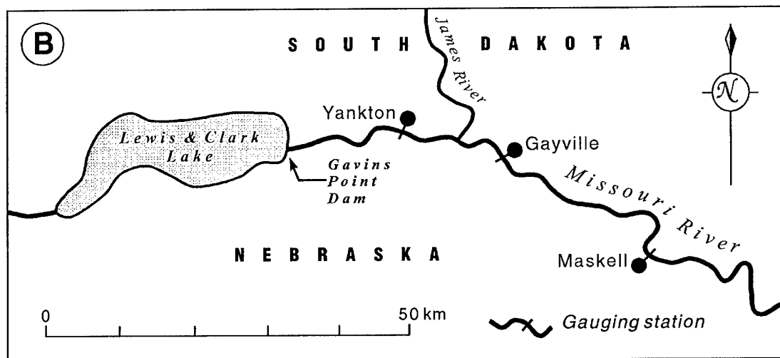
Figure 3-1a) Location and (b) detail of the study reach of the Missouri River, USA. The modelled reach is from Gavins Point Dam to Maskell and includes the gauging stations at Yankton and Gayville.
