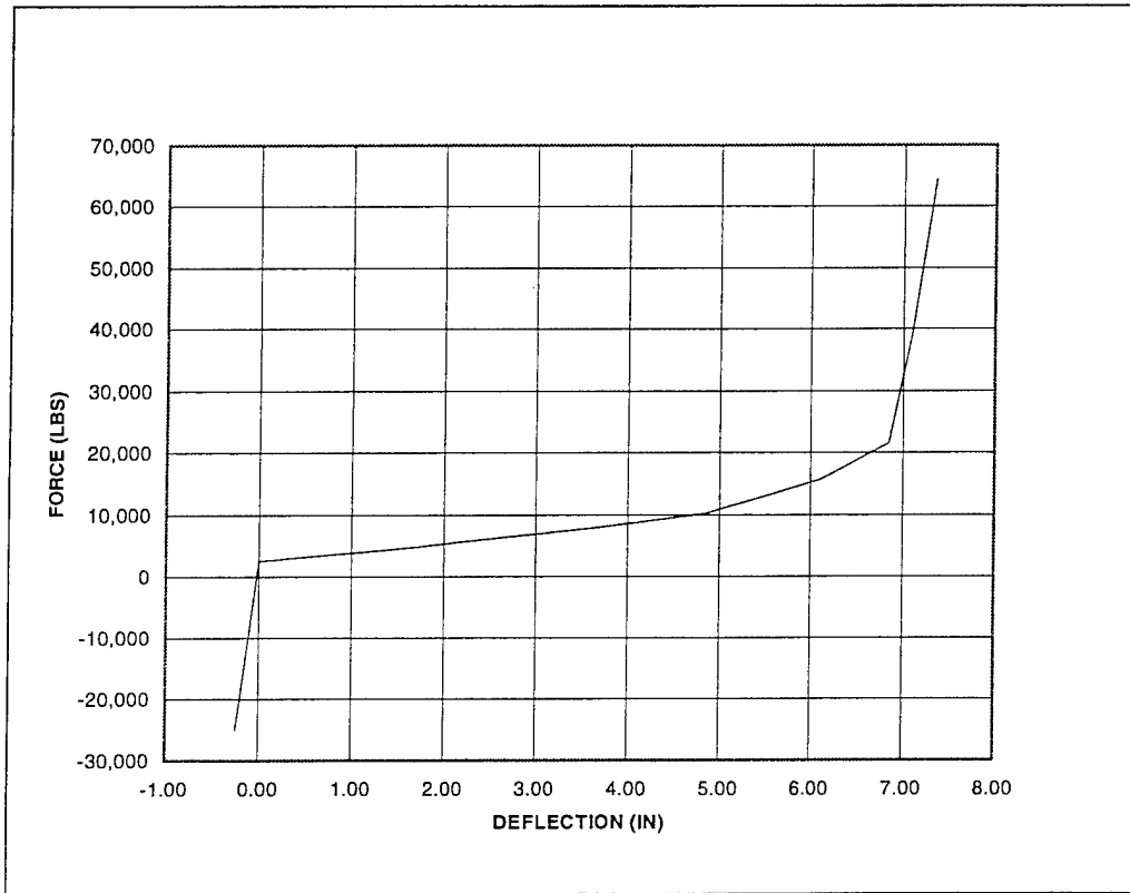
Figure 5.3.2-2 - NEWAY Suspension Spring Characteristics
