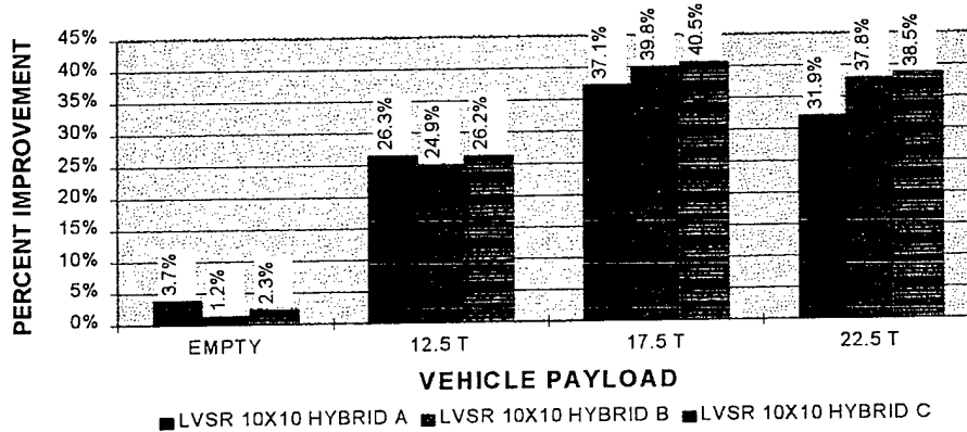
Figure 4.3.2-2b - Hybrid Vehicle Trafficability Improvement
