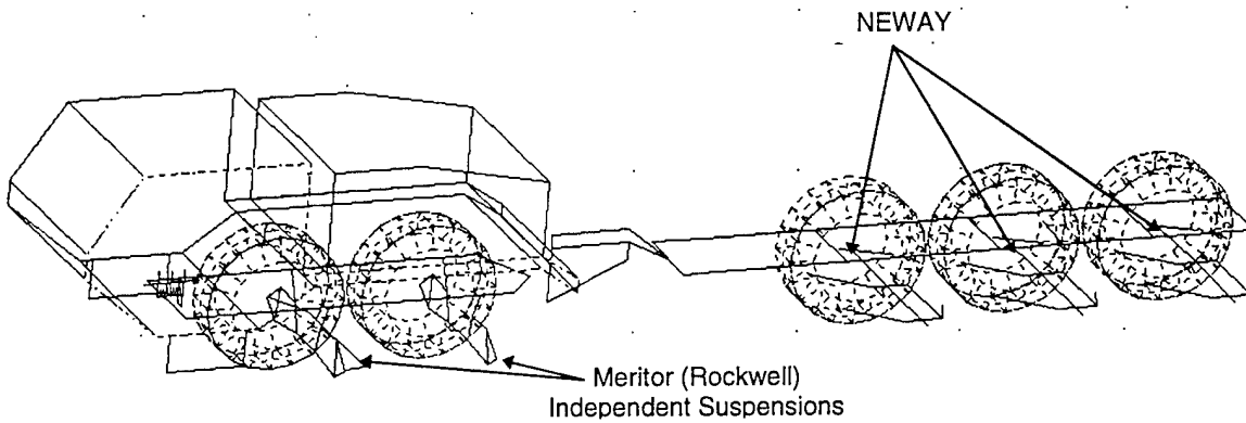
Figure 5.2-2 Model with Recommended LVSR Suspension (deck and left side wheels omitted for clarity)
