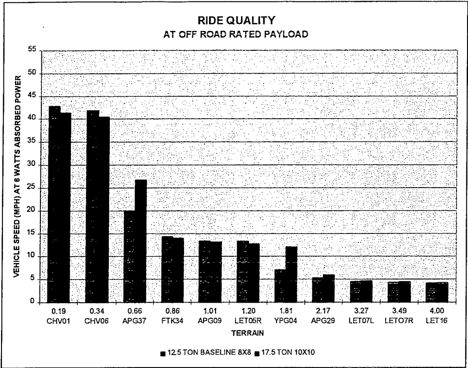
Figure 4.1.3-6a - Ride Quality Comparison (Rated Payload)
