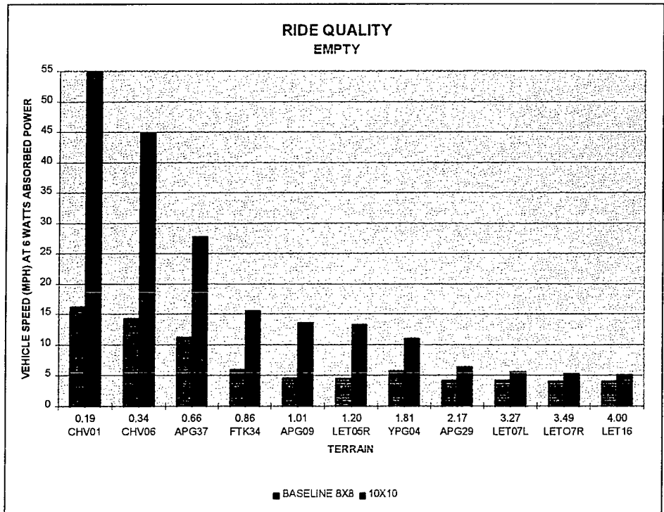
Figure 4.1.3-6b - Ride Quality Comparison (Empty)
