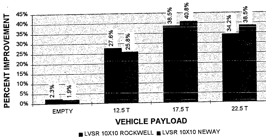
Figure 4.3.2-1b - Vehicle Trafficability Improvement
