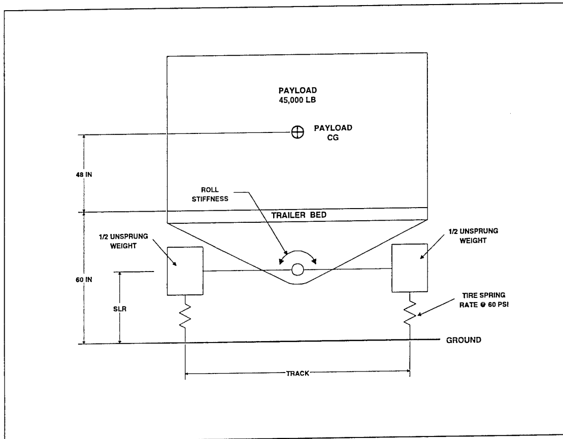
Figure 4.3.4-1 Rollover Model
