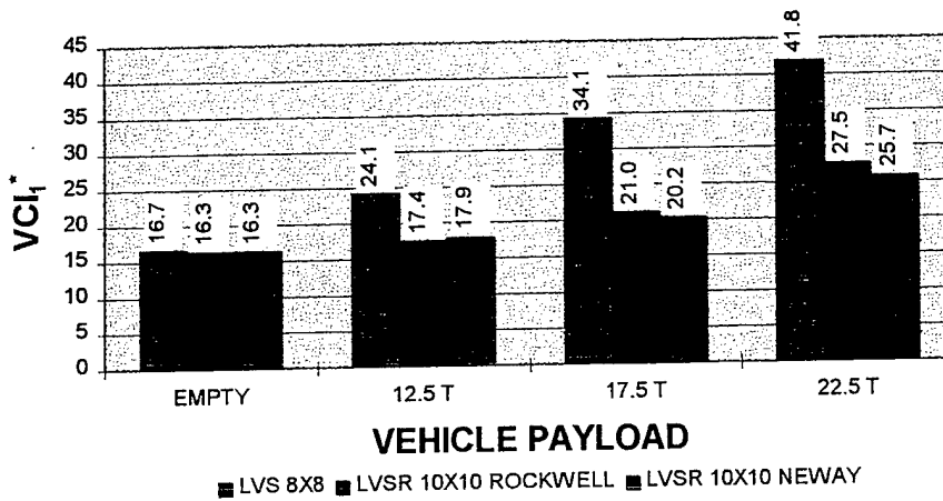
Figure 4.3.2-1a- Vehicle Trafficability
