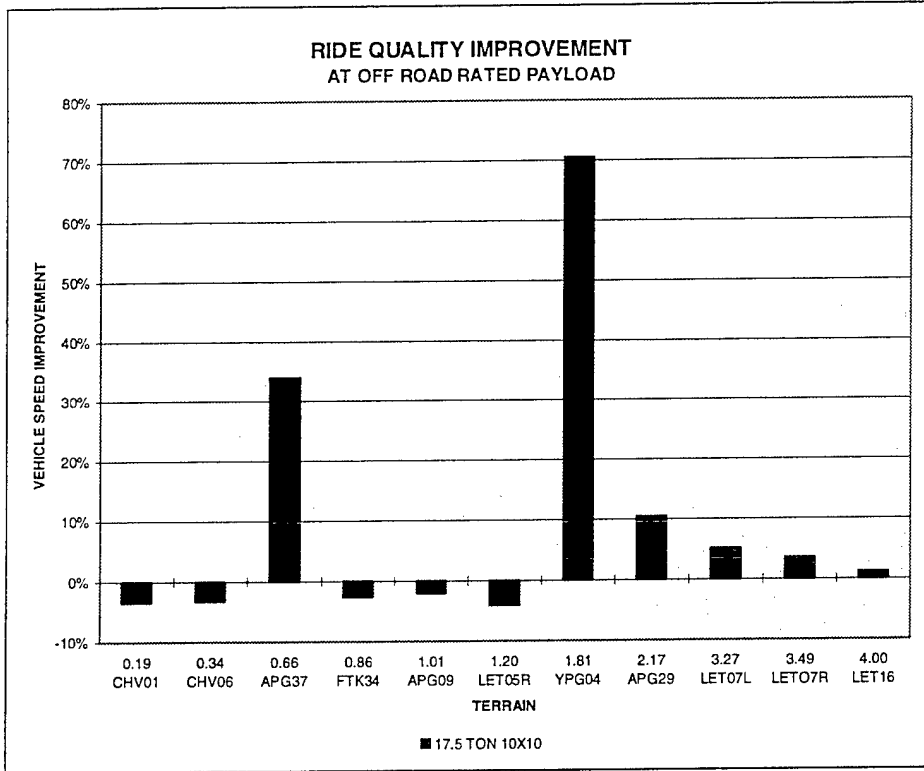
Figure 4.1.3-7a - Ride Quality Improvement (Rated Payload)
