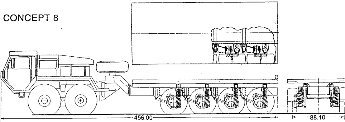
Figure 4.0-1c Preliminary LVSR Concepts
