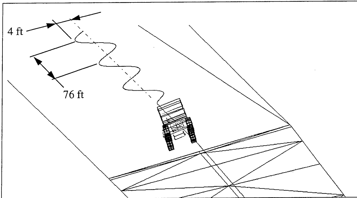
Figure 5.2.2-1 Side Slope with Obstacle Avoidance
