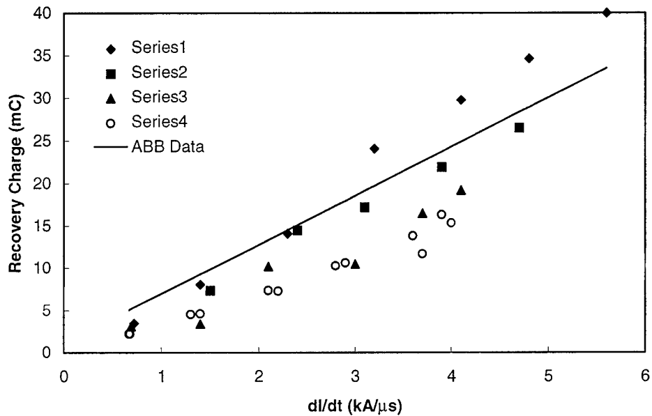
Figure 17. Recovery Charge for Four Test Series.
