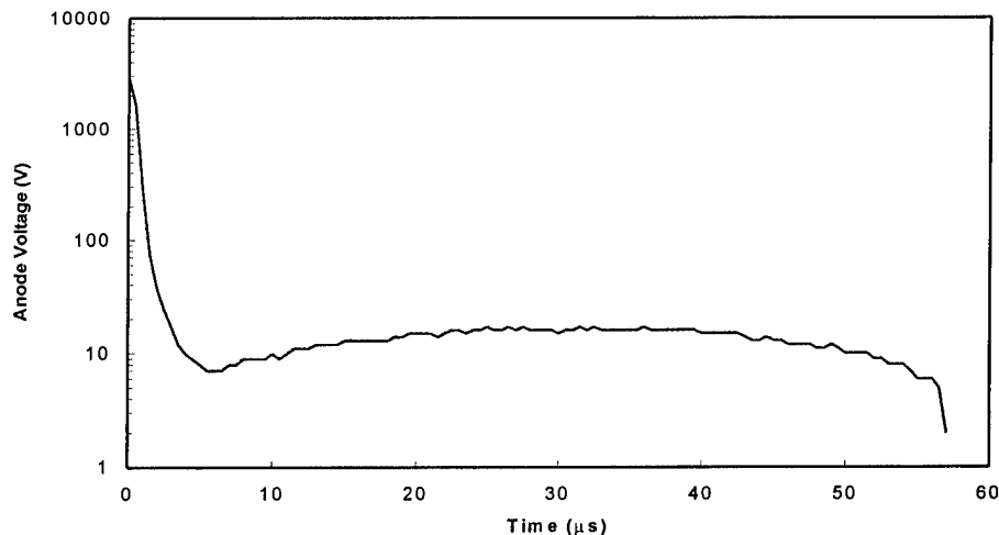
Figure 12. Voltage Drop Across the Thyristor.
