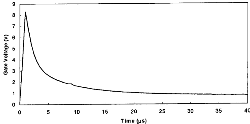
Figure 6. The Gate Voltage.
