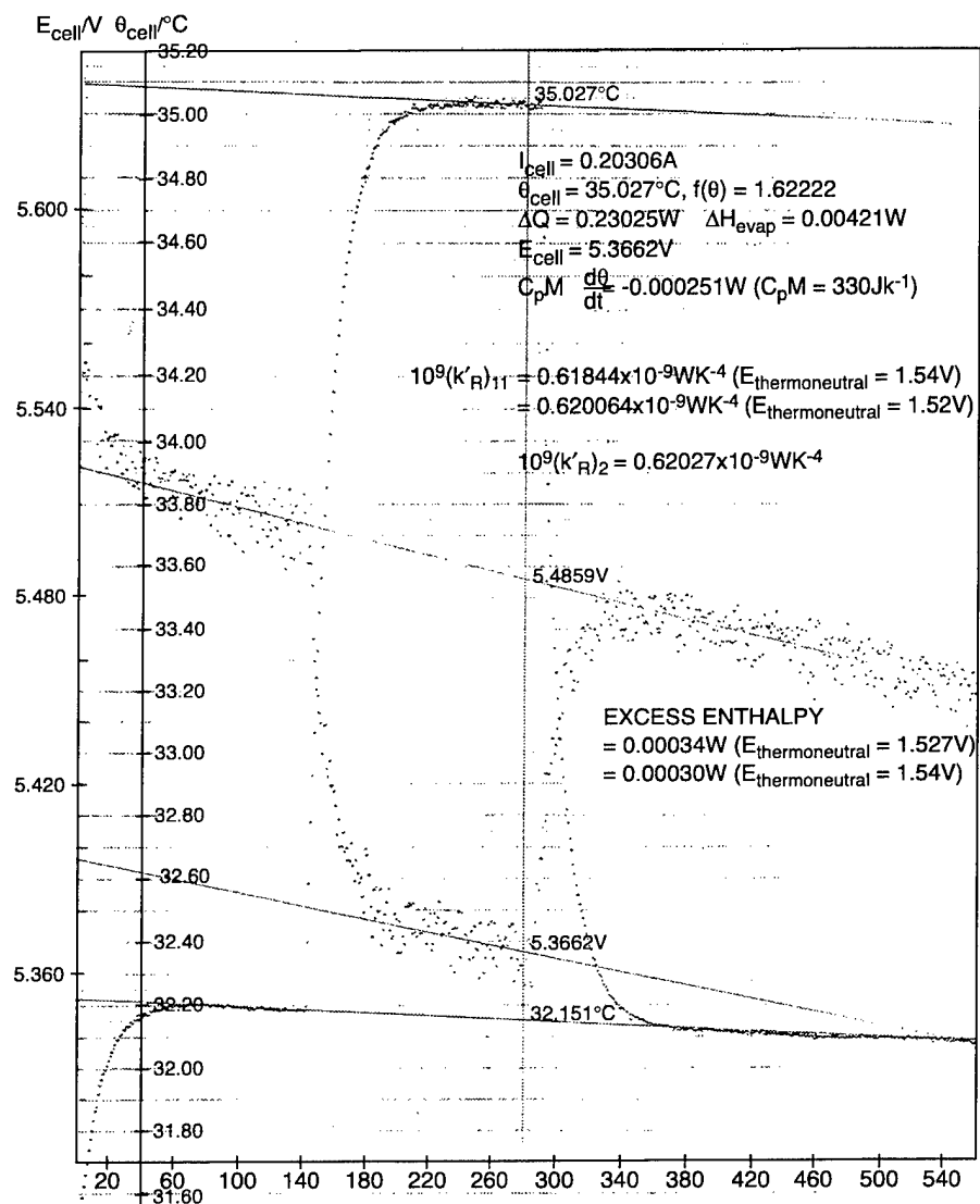
Fig. 38. The "raw data" for a blank experiment (Pt in 0.1M LiOD/D 2 O) in an ICARUS-2 calorimeter. Third measurement cycle. Evaluation of (k'_4)_{11} and (k'_R)_2 using the graphical method.
