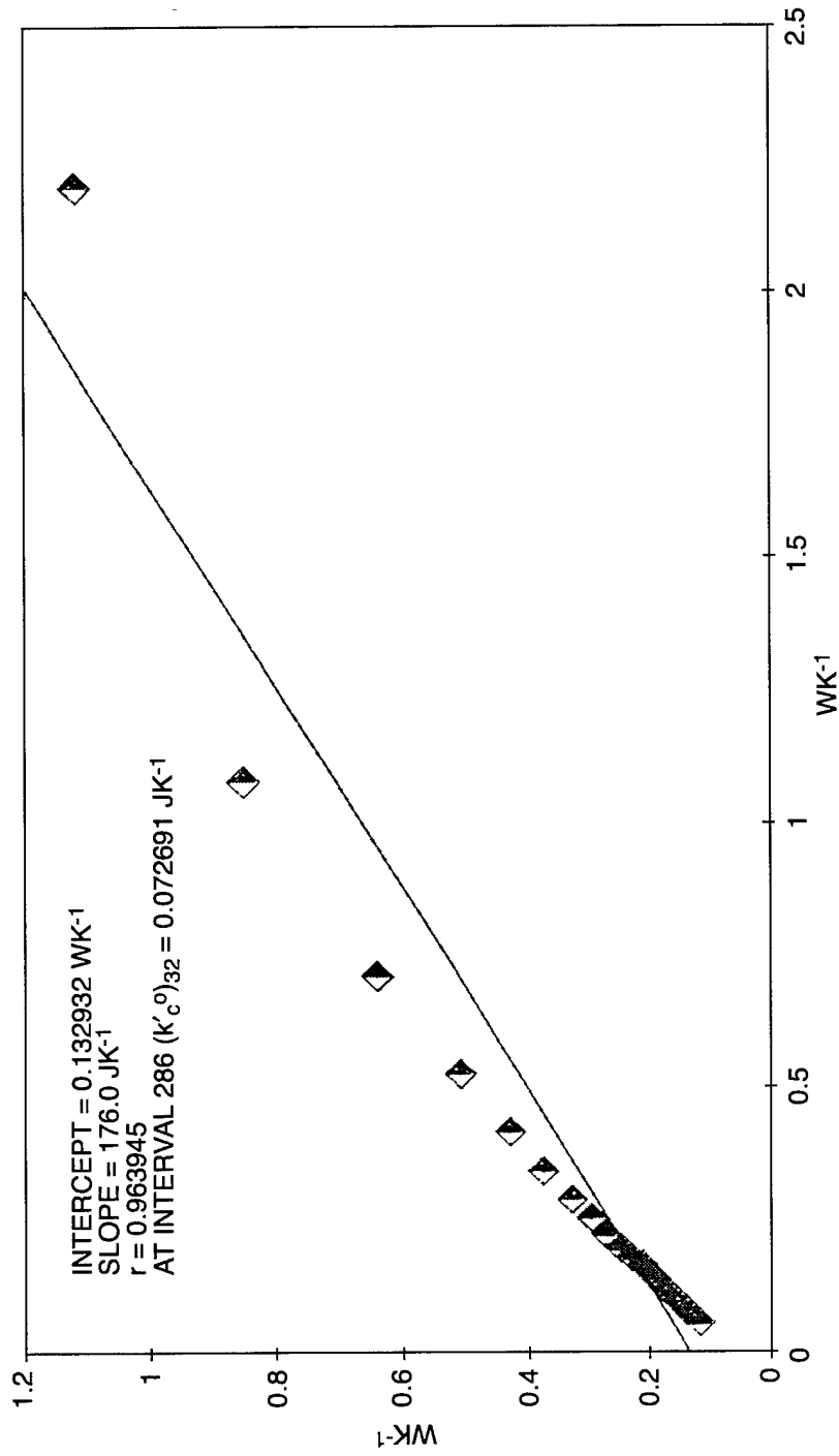
Fig. 35. ICARUS-2 simulation. Evaluation of (k'_c)^{362} with error -30J in input enthalpy and using intervals 145-177.
