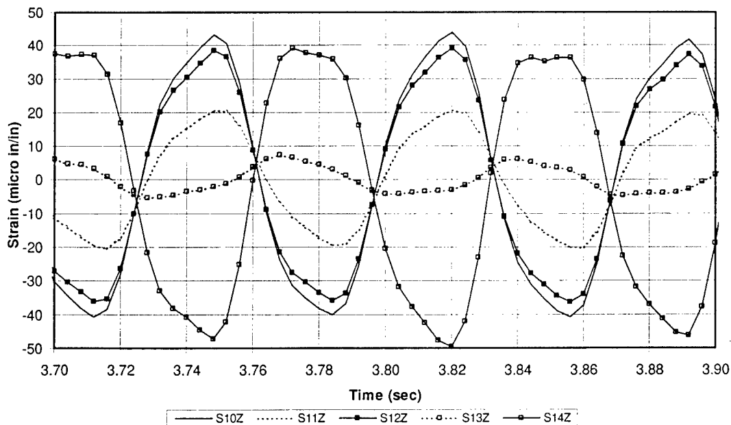
Figure 30. Strain measurements along the back face.
