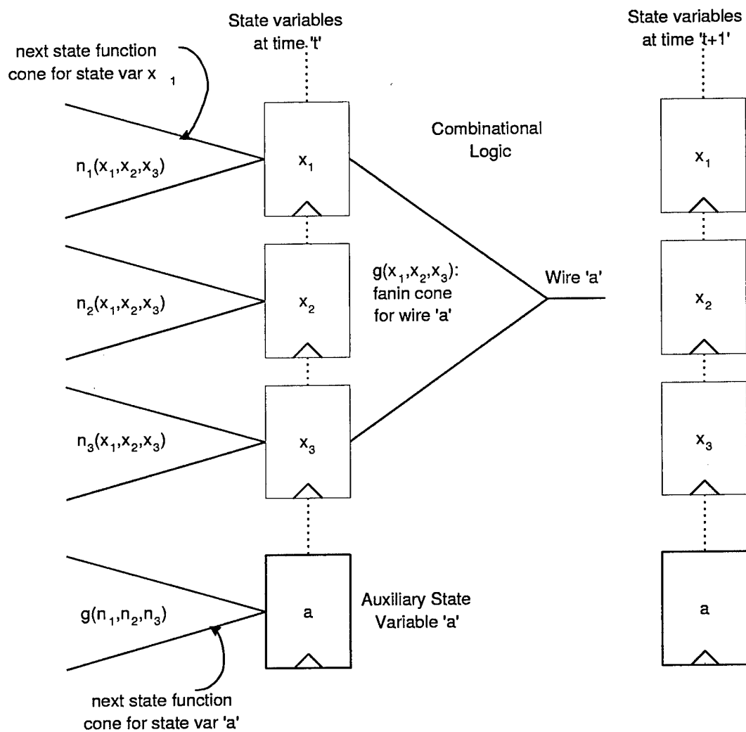
Figure 6.3: Design including auxiliary state variables
