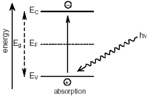
Figure IV-4. Electron-Hole Creation from Light.
