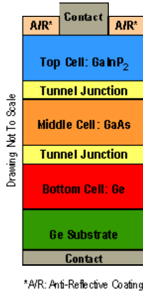
Figure VI-1. Spectrolab GaInP 2 /GaAs/Ge Triple-Junction Solar Cell [From: Appendix A].
