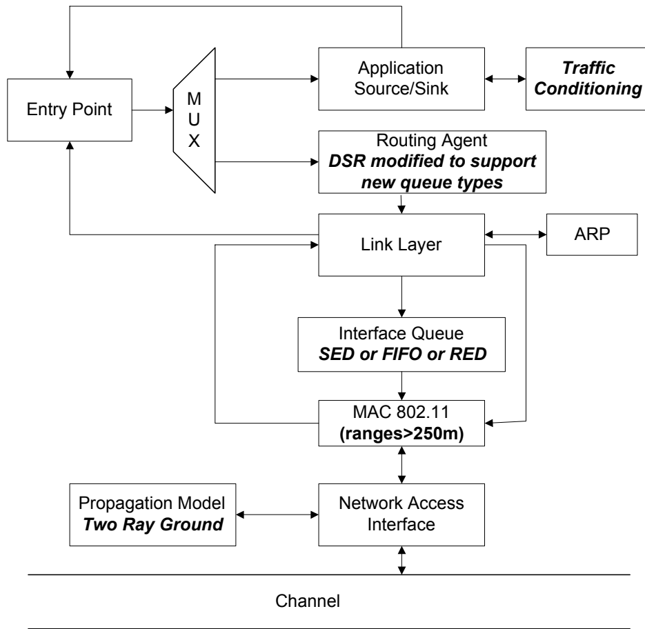
Figure 18. Schematic of a Mobile Node Protocol Stack in NS2 (After Ref. [42]).
