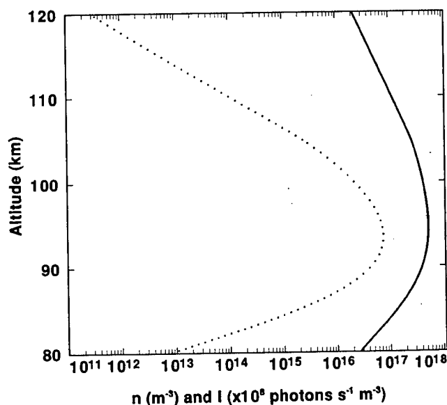
Figure 2. Atomic oxygen density taken from the model of Garcia and Solomon [1985] for January 18°N (solid line) and derived \text{O}^1\text{S} emission profile (dashed line) employing the chemistry given in the appendix.
