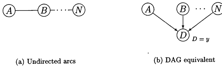
Figure 6.2: Dealing with undirected relations
