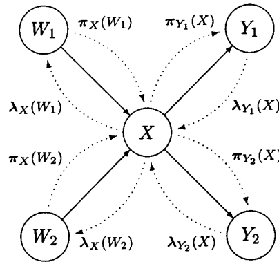
Figure 5.4: Propagation in a causal polytree network
