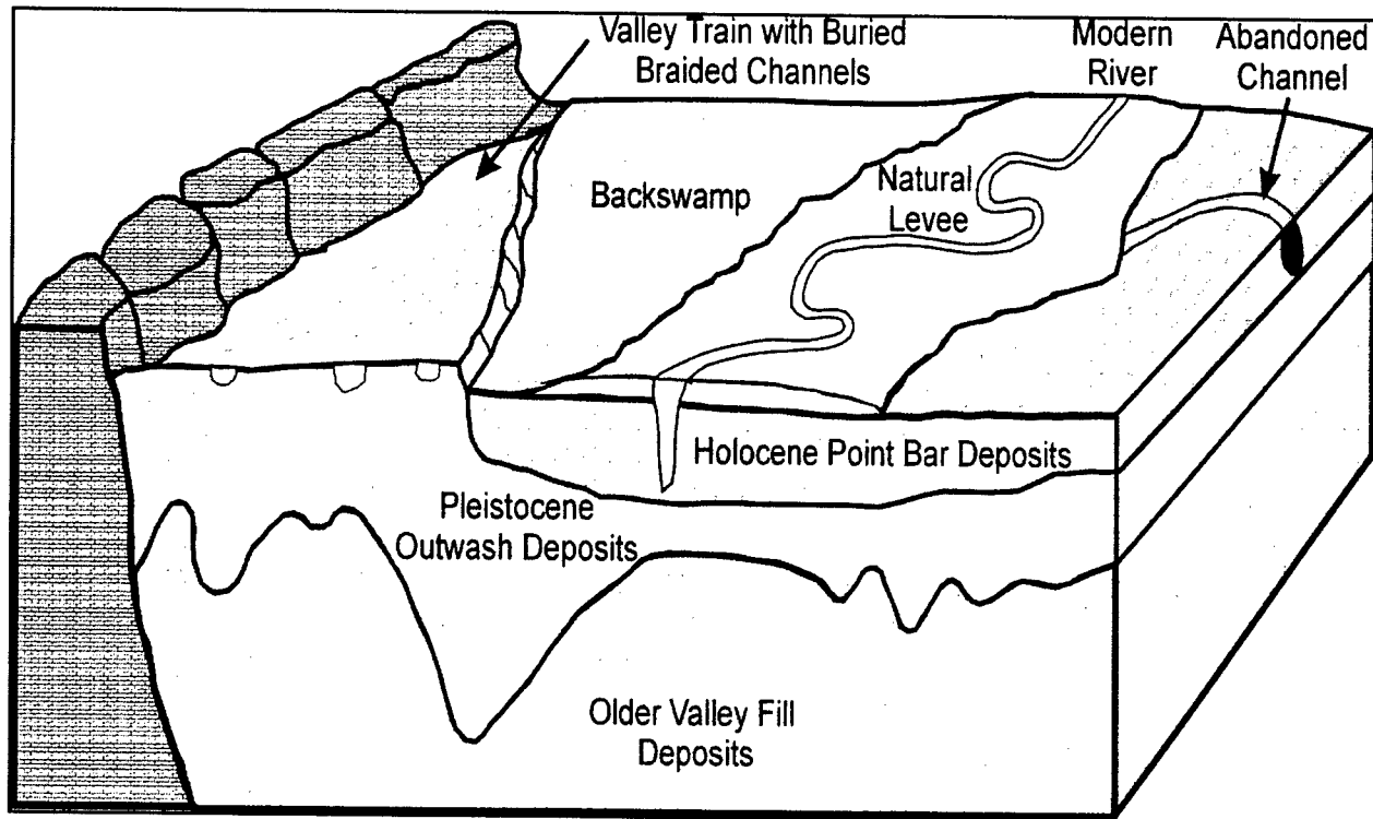
Figure 5. Block schematic of geomorphic features of the Yazoo Basin (from Saucier 1994)
