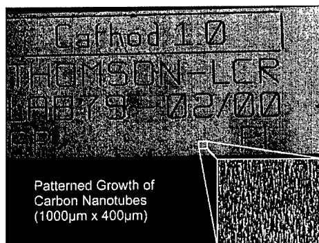
Figure 4(a). Uniform preferential growth of carbon nanotubes achieved by patterning the initial Ni catalyst by optical lithography.
