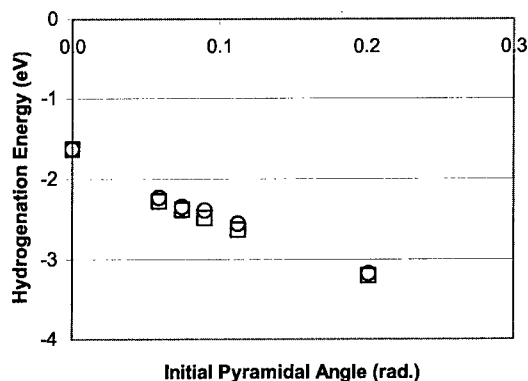
Figure 3. Hydrogenation energies of graphene sheet, various nanotubes, and C_{60} . Circles are DFT simulation data with full relaxations, and squares are the predicted values from our analysis. Data points represent from left to right, graphene sheet, and four different sizes of nanotubes listed above, and C_{60} .
