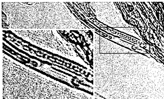
Figure 3: \text{Er}_3\text{N}@\text{C}_{80}@\text{SWNT} at
