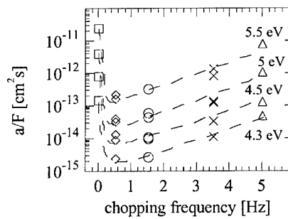
Figure.4 The dependence of CPM data, a/F, in LLa-CN x #103 at a fixed photon energy on chopping frequency.(F [cm 2 s]: photon number)
