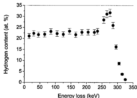
Figure 3. Hydrogen depth profile for a film grown at 0.5 mTorr with V_0 = -250 V.
