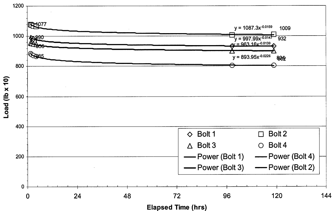
Figure 2.2 – Sample Results From Compression Block Test
