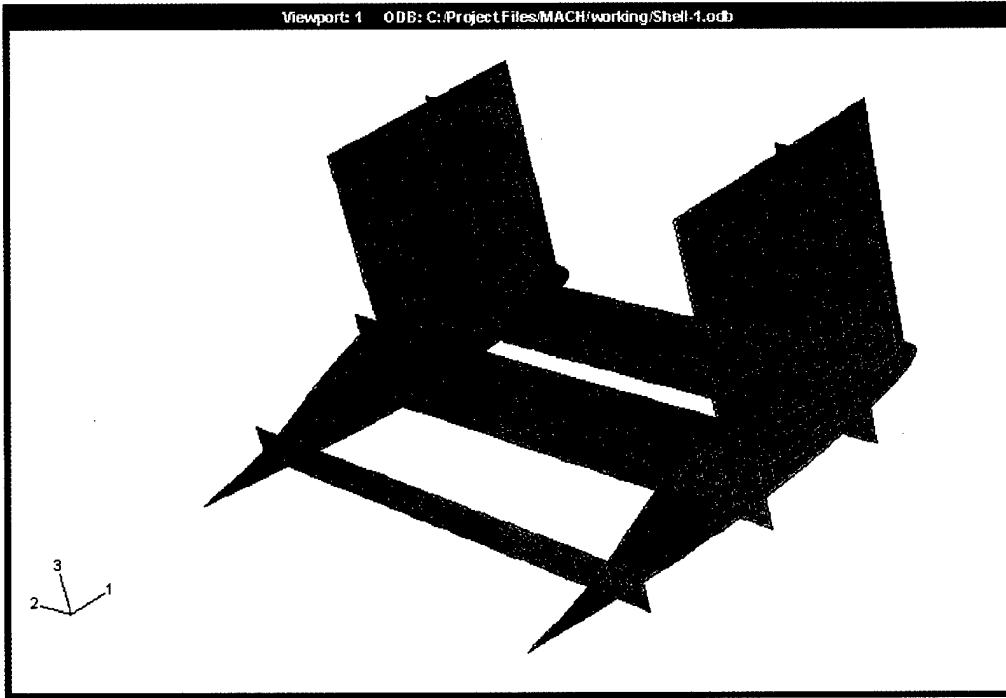
Figure 6.2 - Primary structure element set
