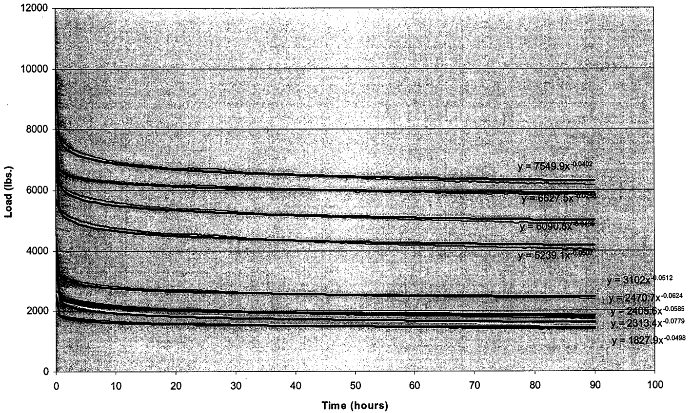
Figure 2.4 – Sample Results From Single Bolt Tests.
