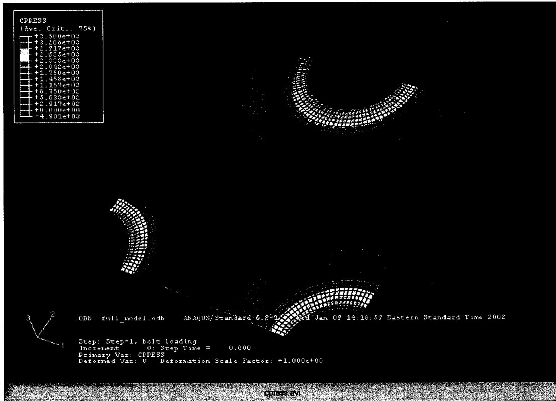
Figure 2.10 - Contact stresses
