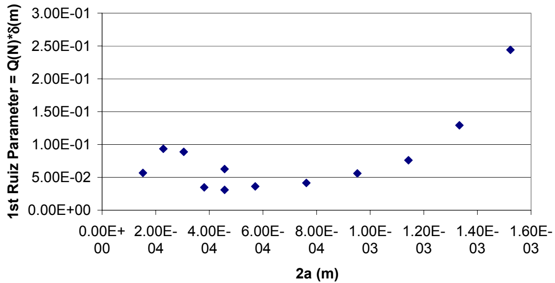
Figure 4.48 Maximum Values of F_1 Ruiz Parameter, with max \delta and max Q (Both from the Experimental Test Output) Versus Contact Width
