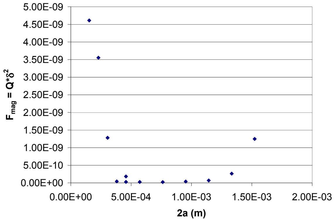
Figure 4.49 Maximum Values of Modified Ruiz Parameter Versus Contact Width
