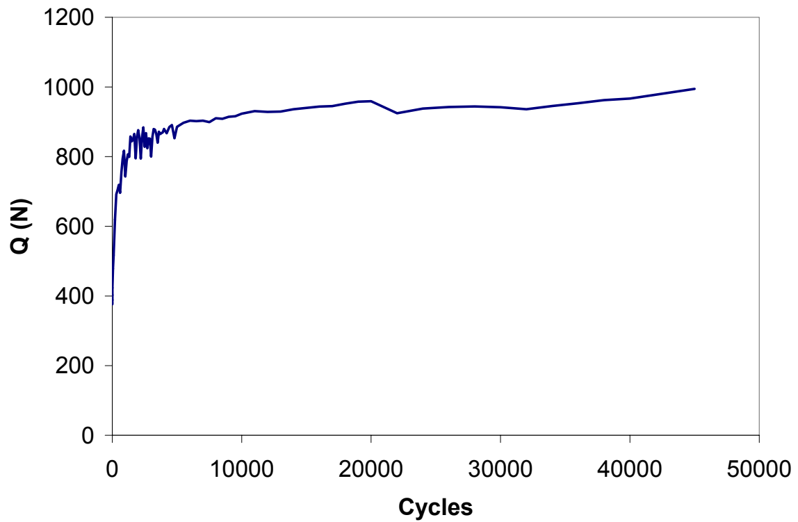
A1.6 Q vs Cycle Curve for Experimental Test Using Pad R=0.0127 m
