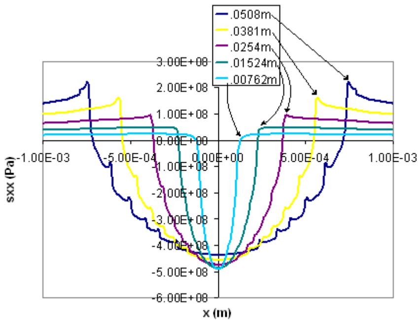
Figure A4.4 The trend from ridged to smooth transition on the curve form compressive maximum to tensile maximum in the P-only analysis of 5 different radii fretting pads.
