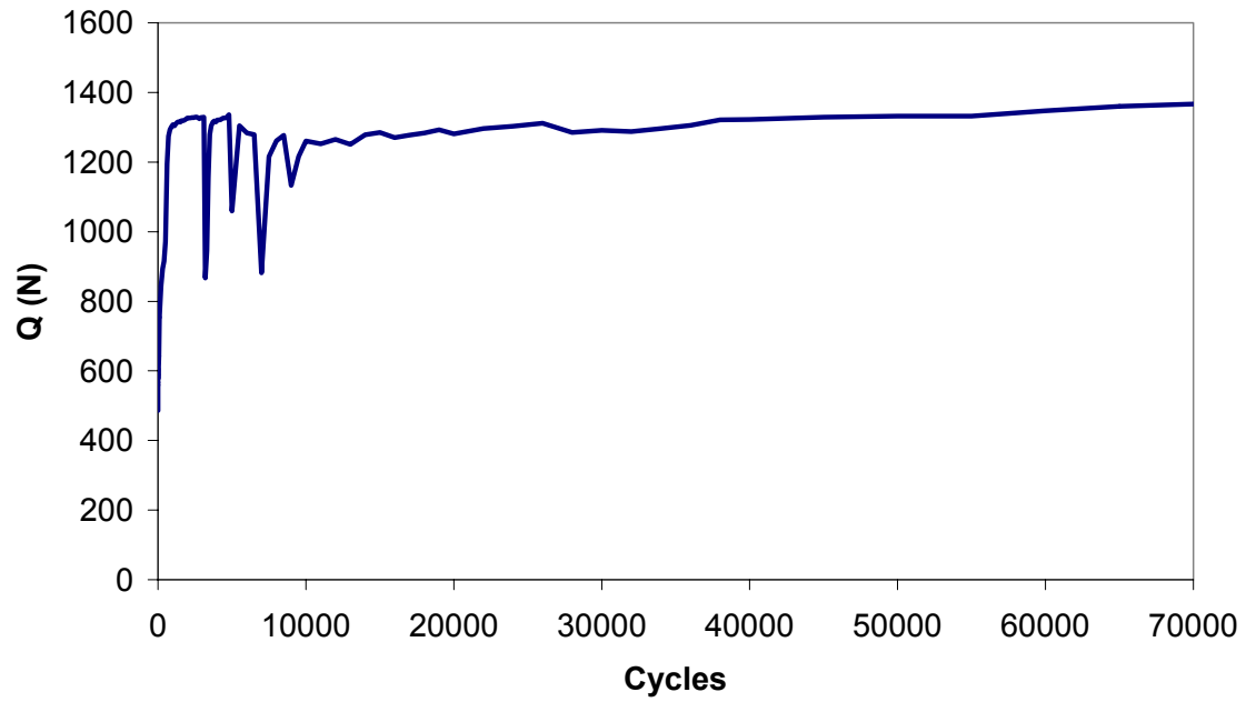
Figure 4.29 Q versus Cycle Curve for Test Using 19.05 mm Radius Fretting Pads
