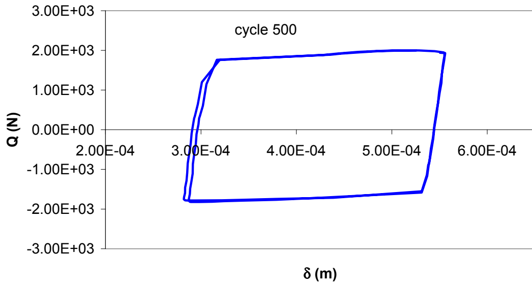
Figure 4.32 Hysteresis Loop for Test Using 44.45 mm Radius Fretting Pads: Cycle 500
