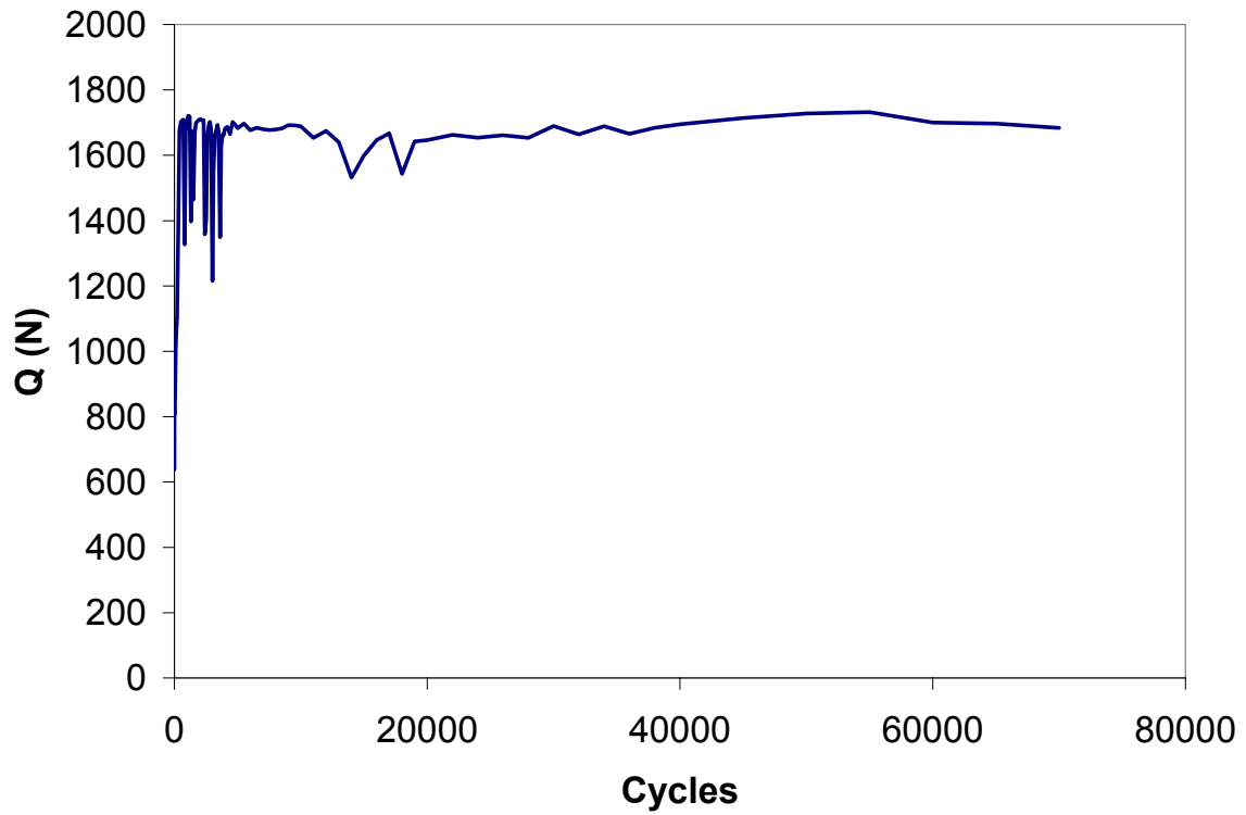
A1.3 Q vs Cycle Curve for Experimental Test Using Pad R=0.0254 m
