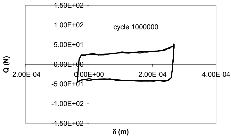
Figure 4.10 Hysteresis Loop for Test Using 5.08 mm Radius Fretting Pads: Cycle 1000000
