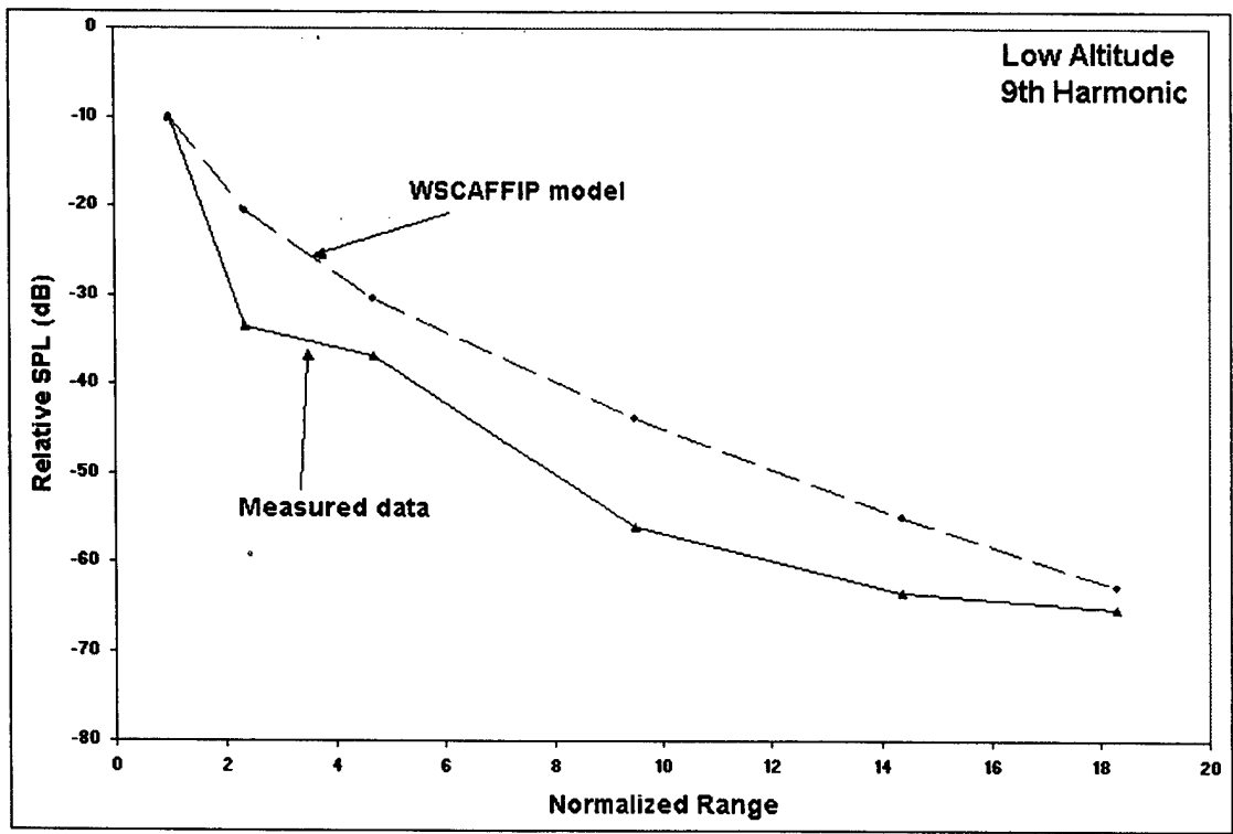
Figure 20. Comparison between WSCAFFIP model and measured data for ninth harmonic at low altitude.
