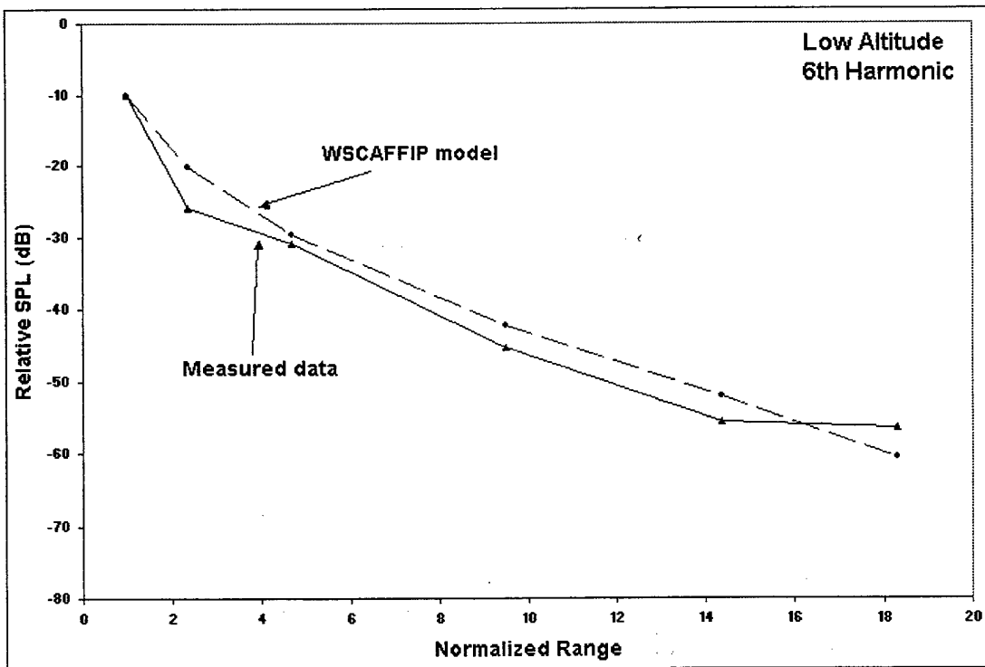
Figure 14. Comparison between WSCAFFIP model and measured data for sixth harmonic at low altitude.
