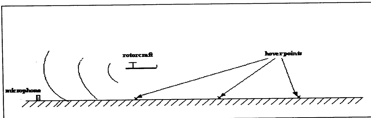
Figure 1. Setup for hovering measurements.
