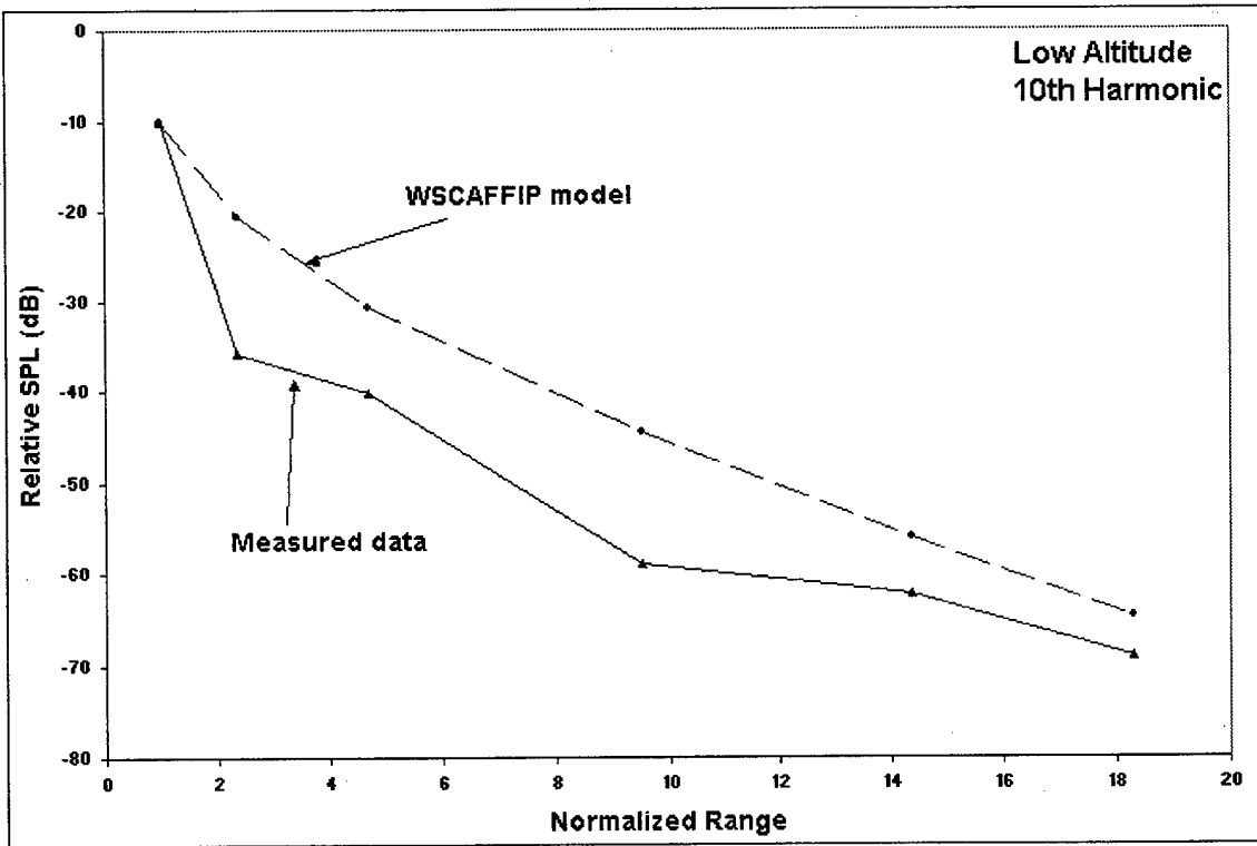
Figure 22. Comparison between WSCAFFIP model and measured data for tenth harmonic at low altitude.
