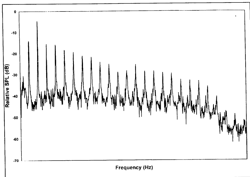
Figure 2. Rotorcraft spectrum.
