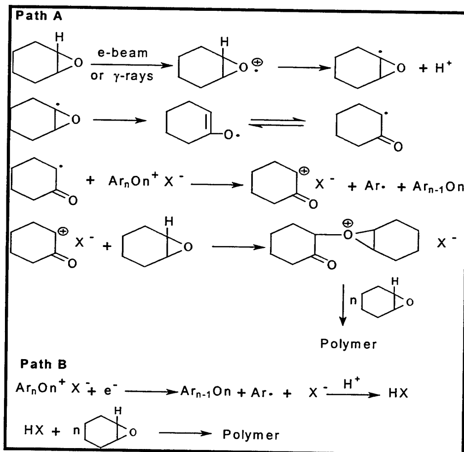
Figure 1. Proposed reaction mechanism for cationic ring-opening of epoxides using E-beam initiation.
