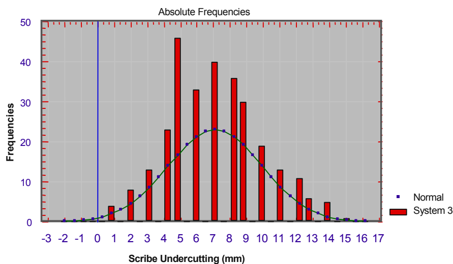
Figure 2. Histogram of System 3 versus normal distribution.
