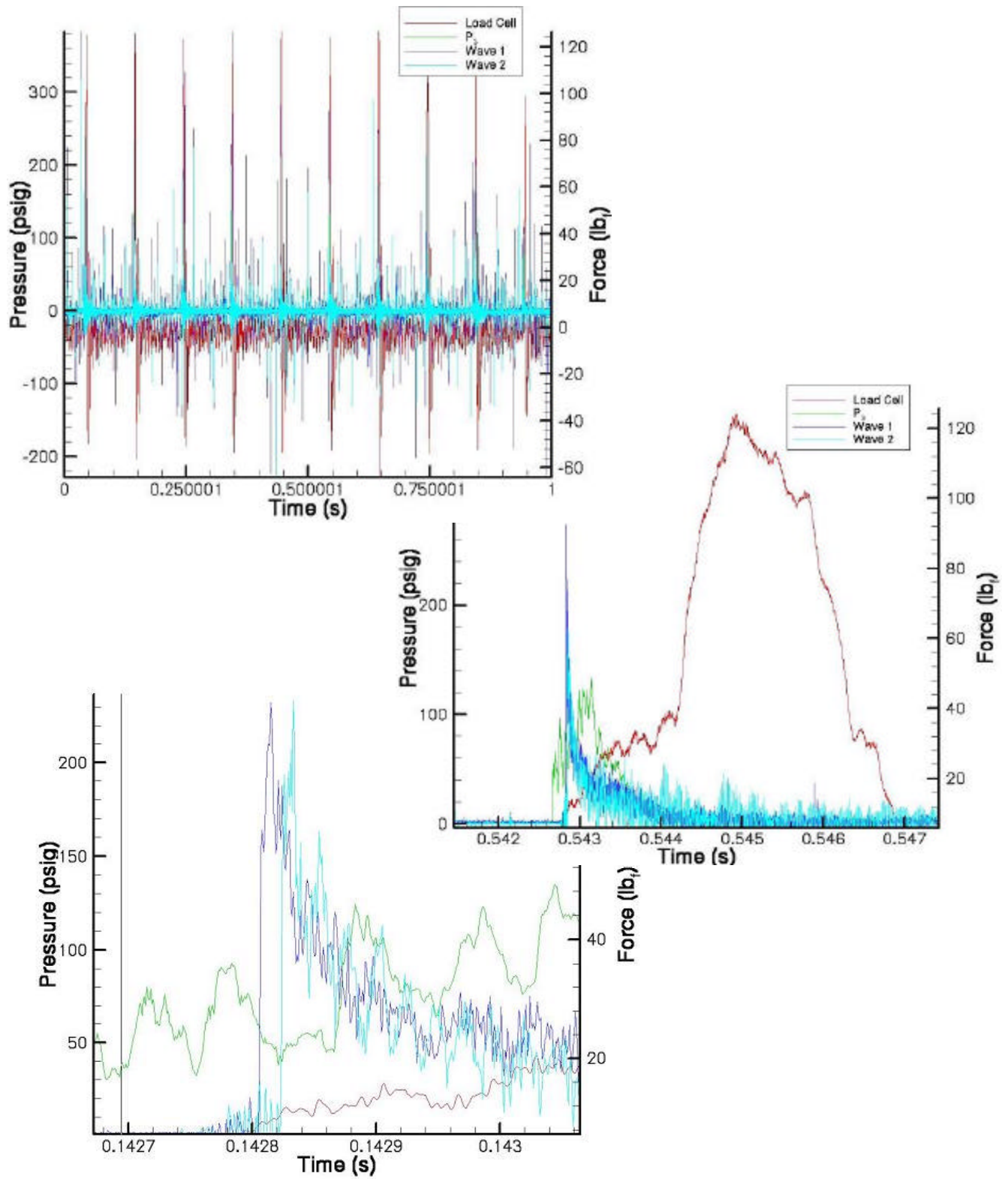
Figure 36. TecPlot™ Output
