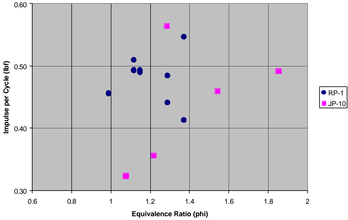
Figure 42. Impulse per Cycle vs. Equivalence Ratio
