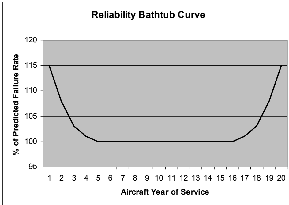
Figure 10 Comanche Bathtub Curve
