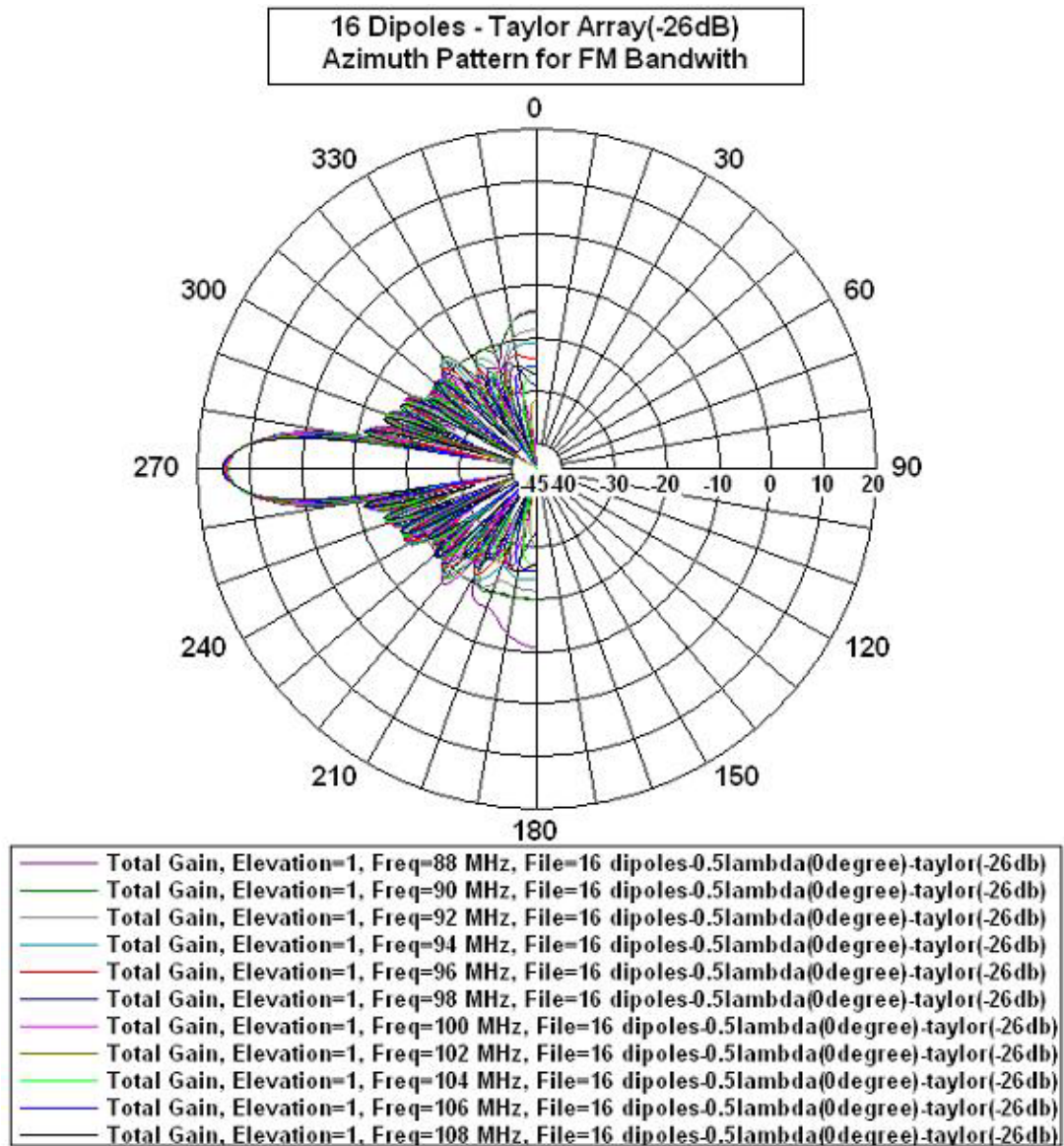
Figure 70: Azimuth Pattern of Taylor Array (-26dB) Operating at 88-108MHz
