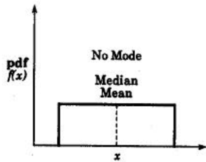
Figure 50. Uniform Distribution.
