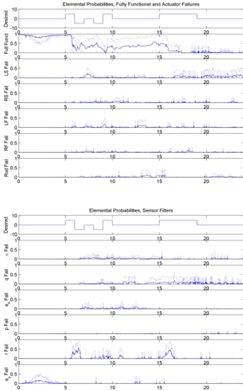
Figure 72a: Elemental Probabilities, Right Flaperon Failure, \epsilon = 75\% Using \epsilon_{\text{HAT}}
