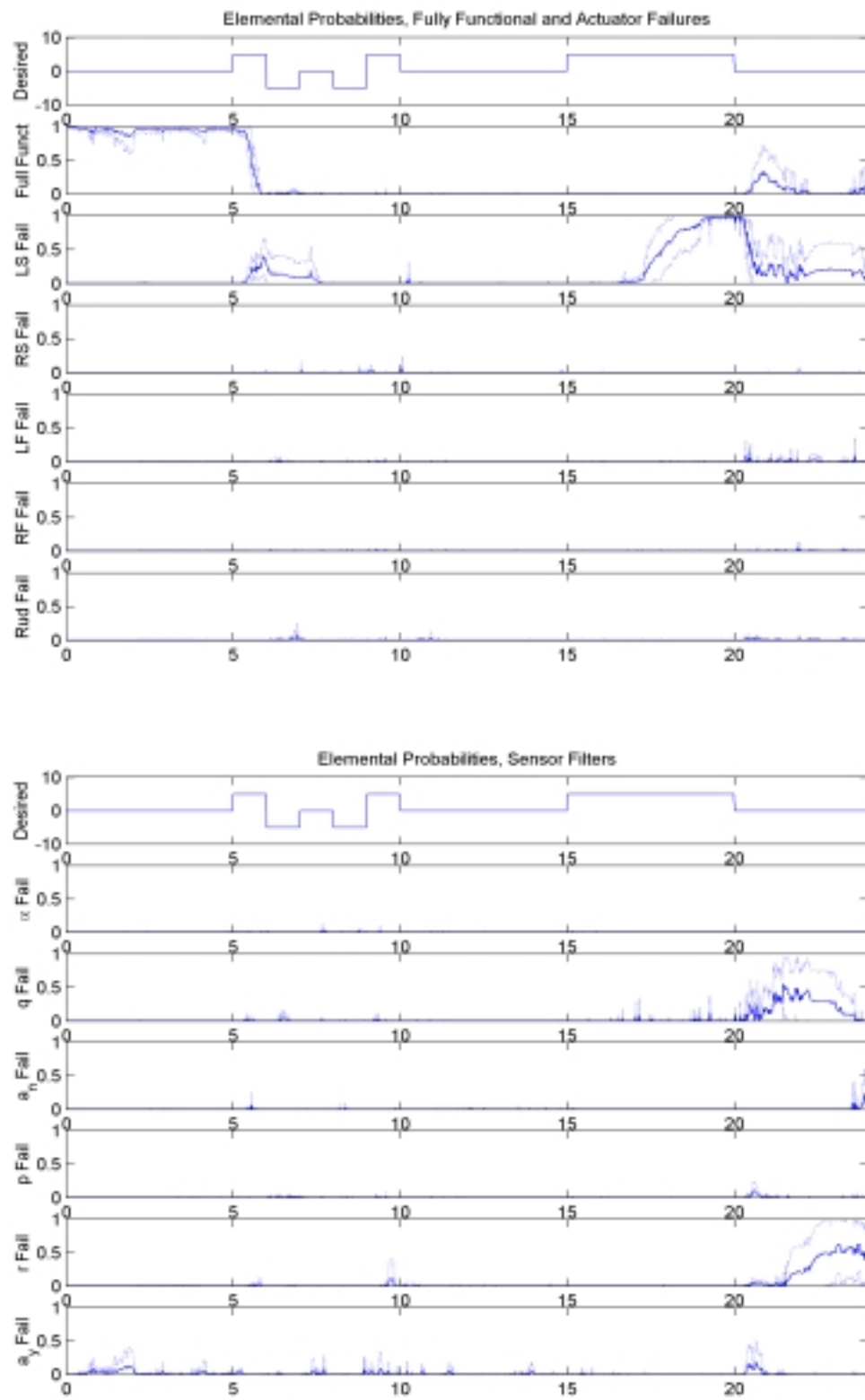
Figure 10a: Elemental Probabilities, Left Stabilator Failure, \epsilon = 25\%
