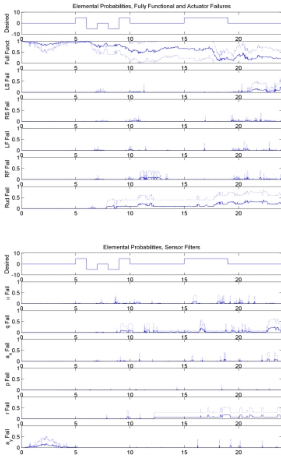
Figure 28a: Elemental Probabilities, Rudder Failure, \epsilon = 75\%
