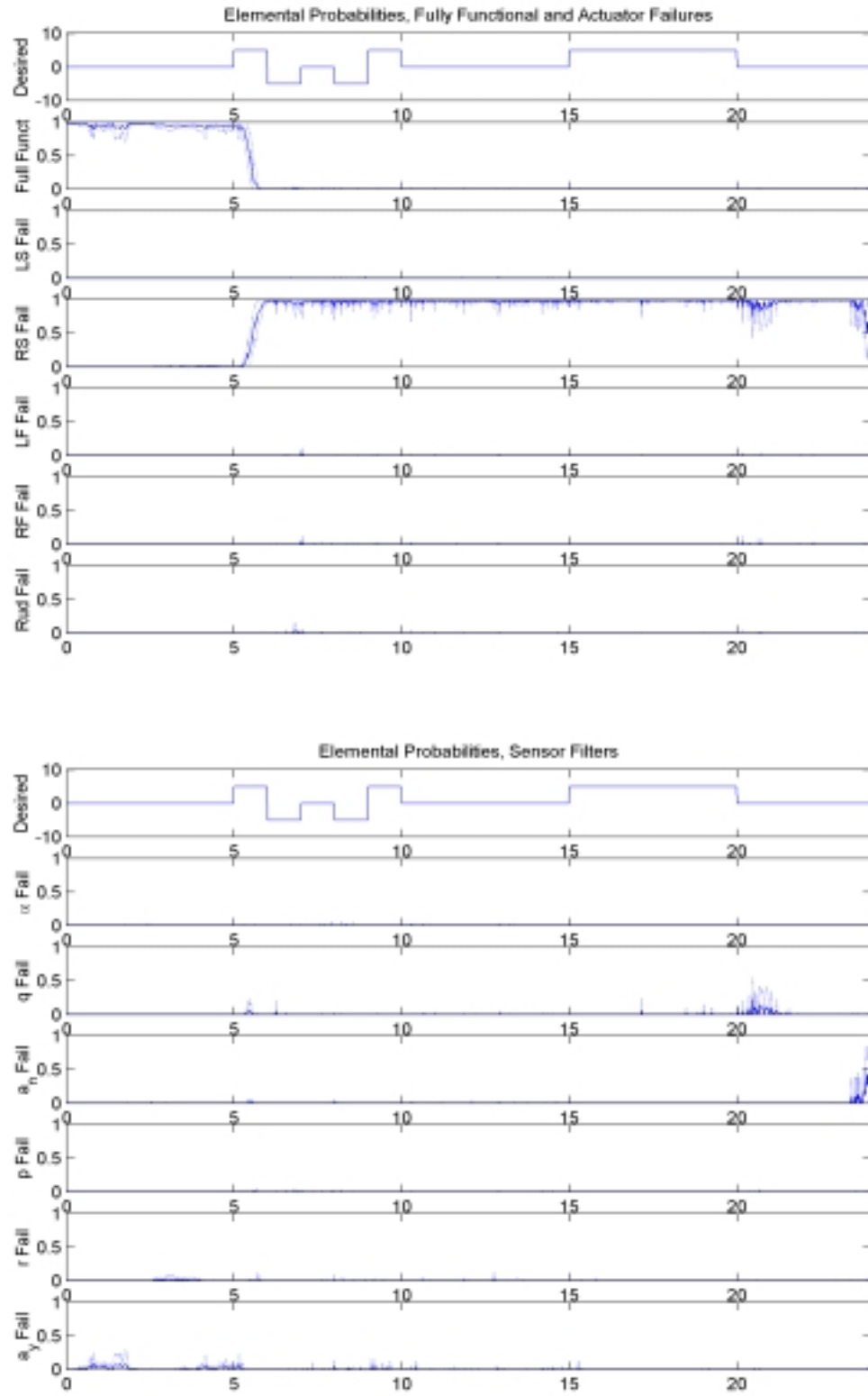
Figure 61a: Elemental Probabilities, Right Stabilator Failure, \epsilon = 0\% Using \epsilon_{\text{HAT}}
