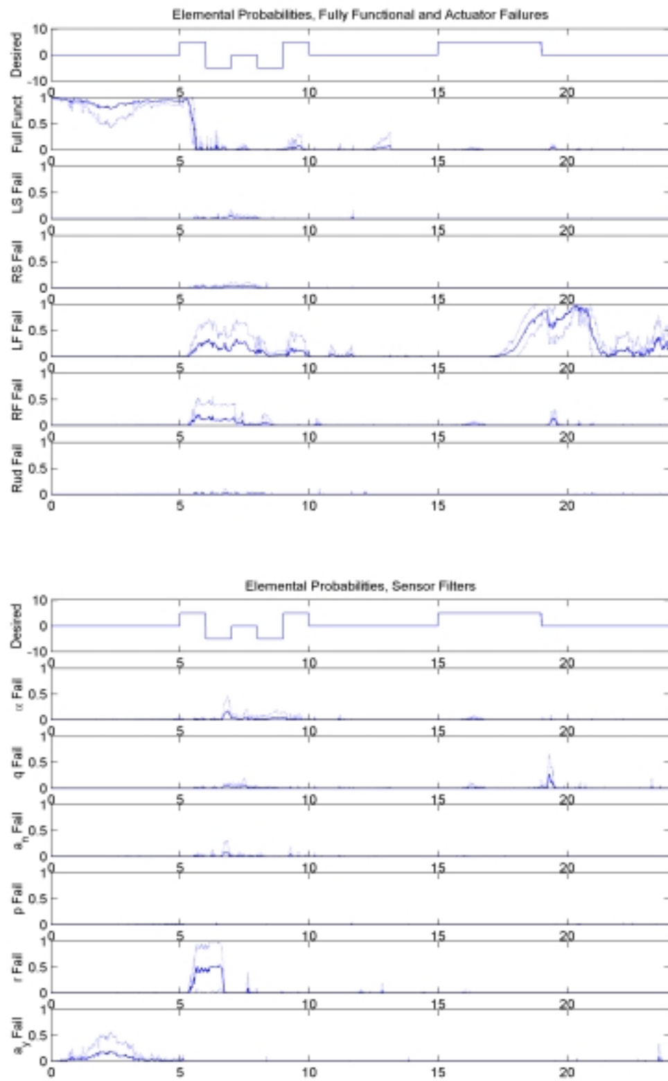
Figure 18a: Elemental Probabilities, Left Flaperon Failure, \epsilon = 25\%
