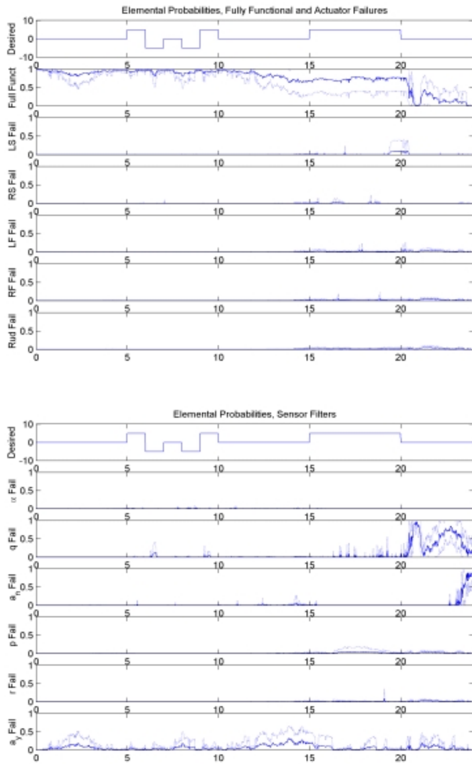
Figure 7a: Elemental Probabilities, Fully Functional Aircraft, Pitch Maneuver
