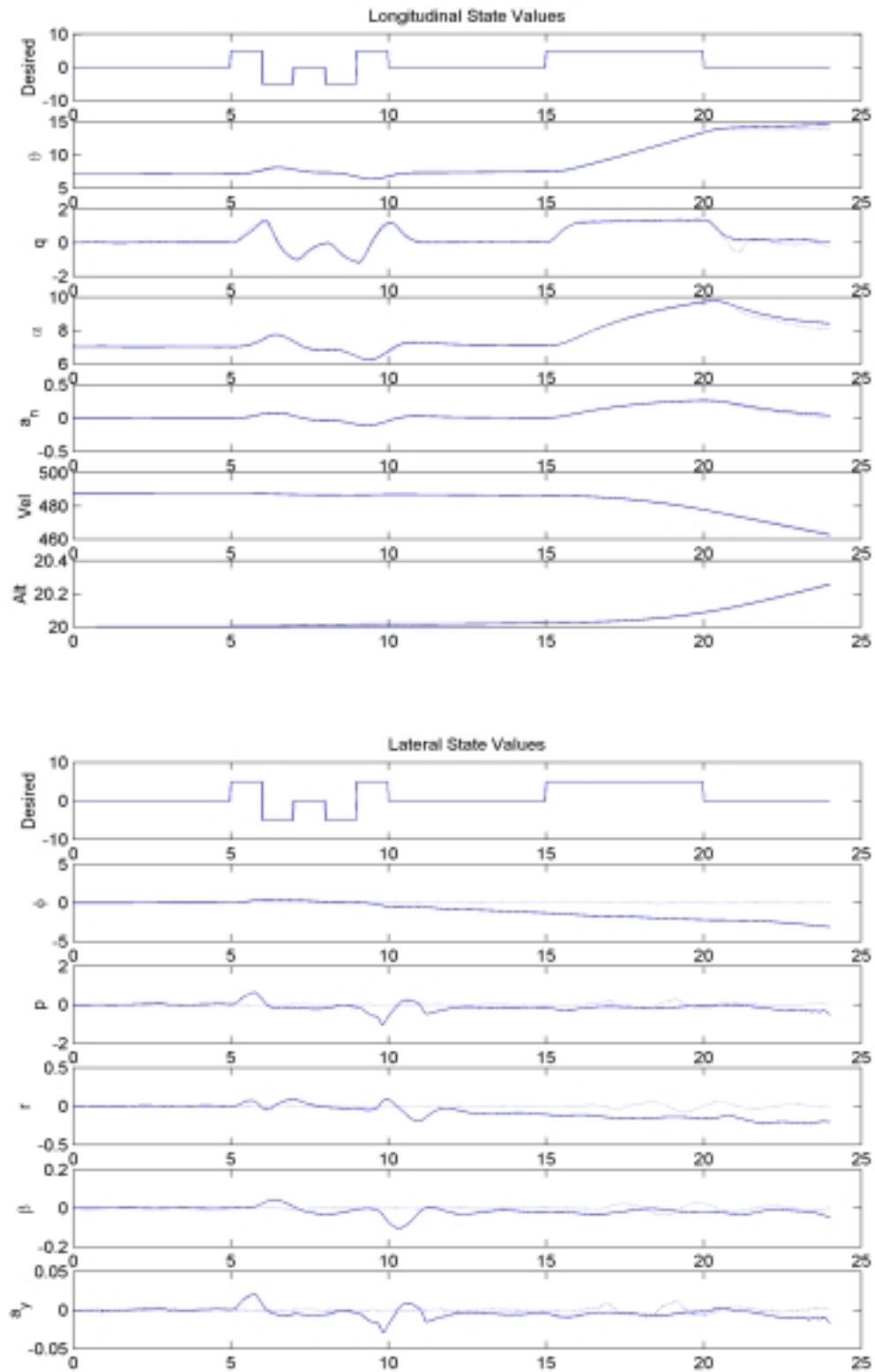
Figure 58c: State Values, Left Stabilator Failure, \epsilon = 25\% Using \epsilon_{\text{HAT}}
