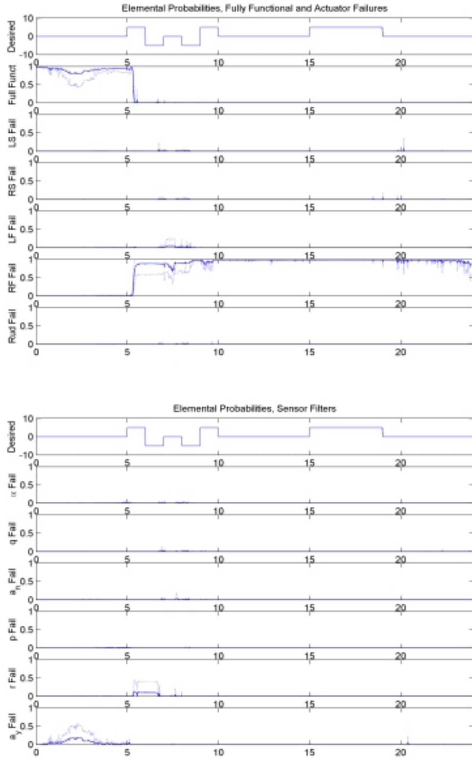
Figure 69a: Elemental Probabilities, Right Flaperon Failure, \epsilon = 0\% Using \epsilon_{\text{HAT}}
