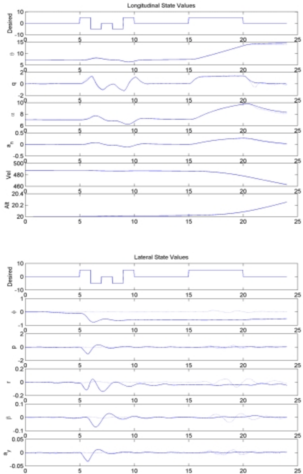
Figure 61c: State Values, Right Stabilator Failure, \epsilon = 0\% Using \epsilon_{\text{HAT}}
