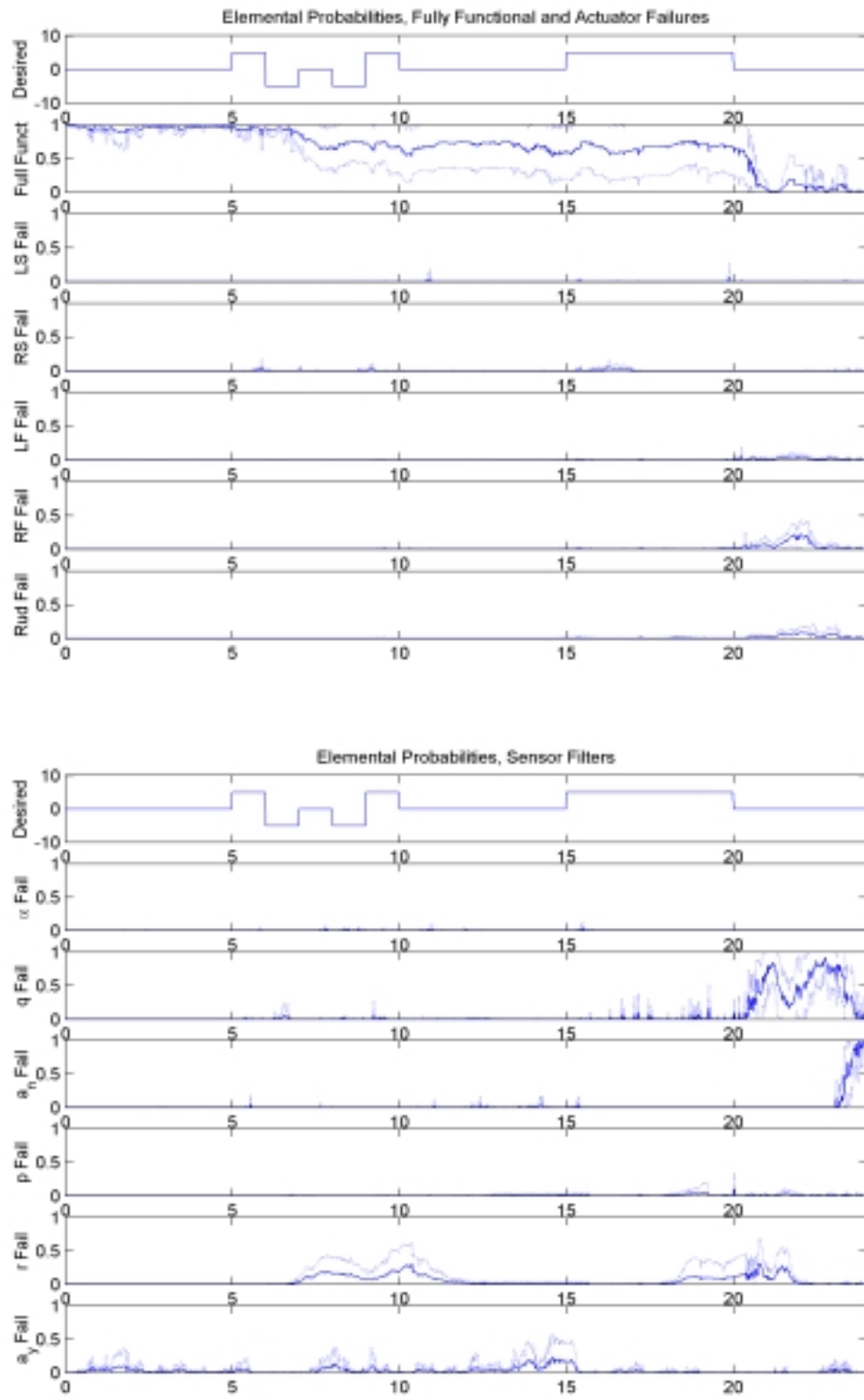
Figure 16a: Elemental Probabilities, Right Stabilator Failure, \epsilon = 75\%
