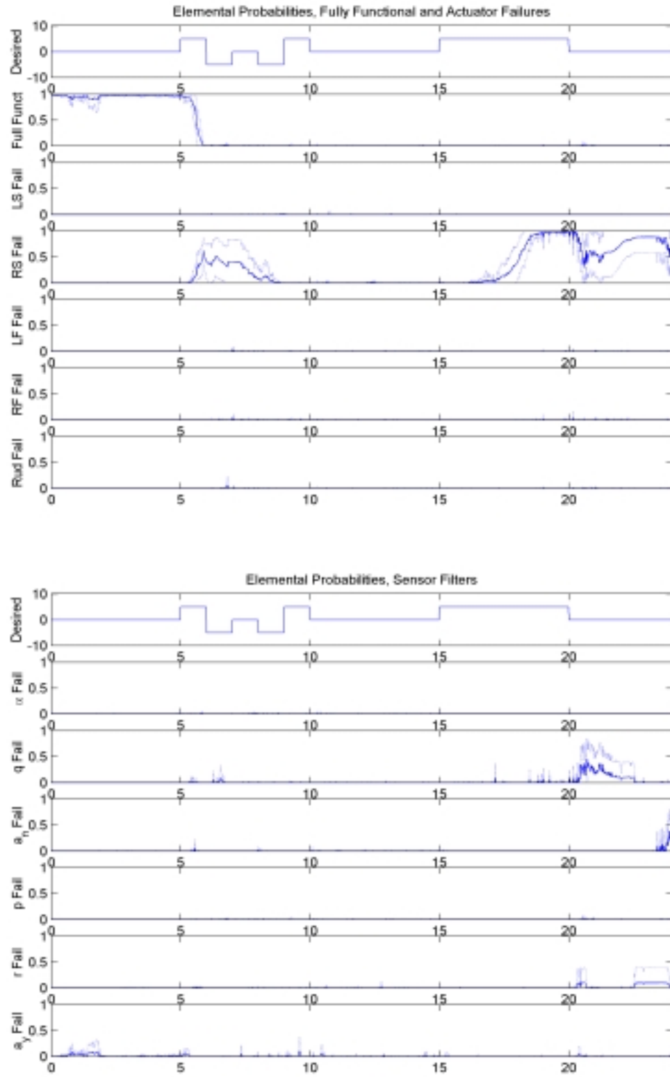
Figure 62a: Elemental Probabilities, Right Stabilator Failure, \epsilon = 25\% Using \epsilon_{\text{HAT}}
