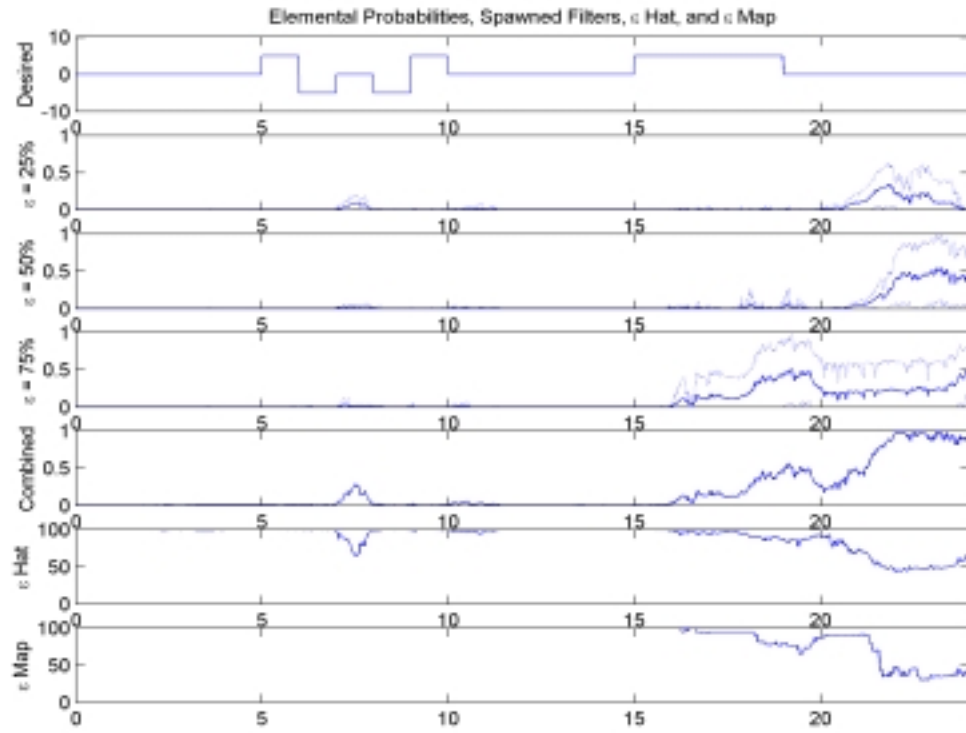
Figure 8b: Elemental Probabilities, Fully Functional Aircraft, Roll Maneuver
