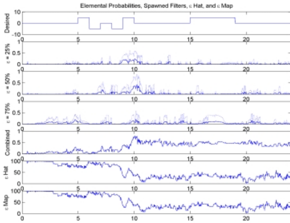
Figure 6b: Elemental Probabilities, Fully Functional Aircraft, Roll Maneuver With Dither
