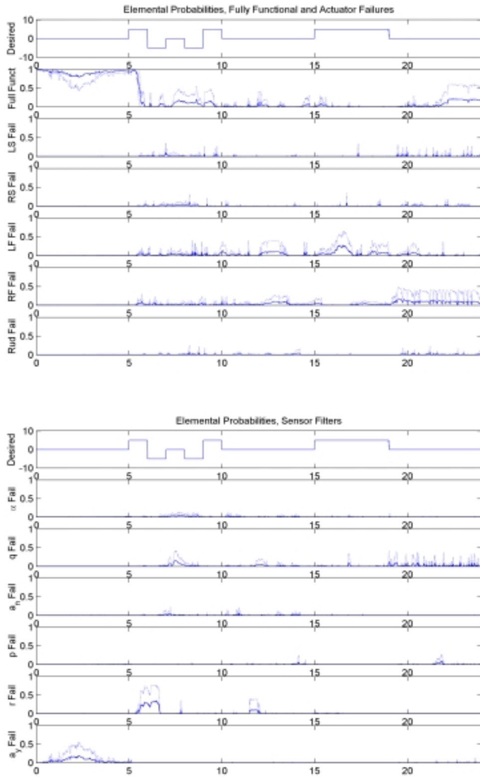
Figure 19a: Elemental Probabilities, Left Flaperon Failure, \epsilon = 50\%
