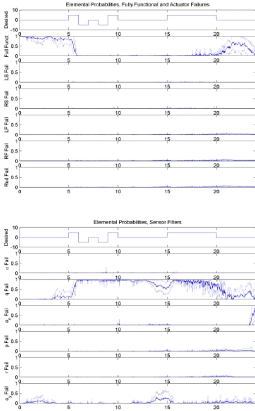
Figure 30: Elemental Probabilities, Pitch Rate Sensor Failure
