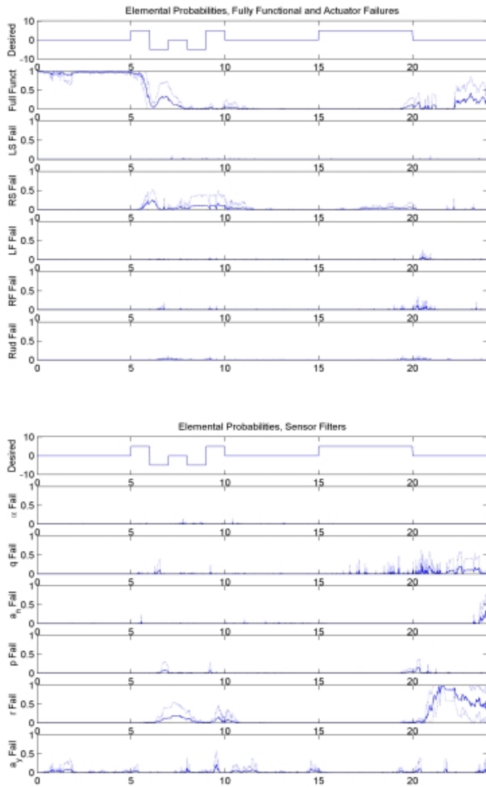
Figure 15a: Elemental Probabilities, Right Stabilator Failure, \epsilon = 50\%
