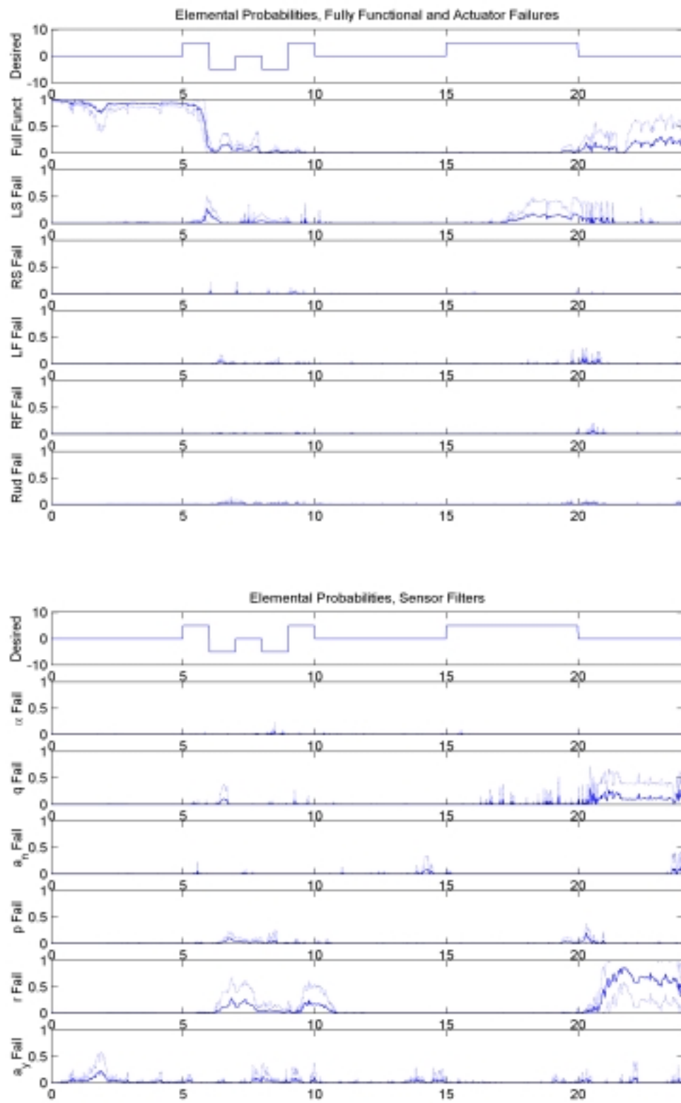
Figure 11a: Elemental Probabilities, Left Stabilator Failure, \epsilon = 50\%
