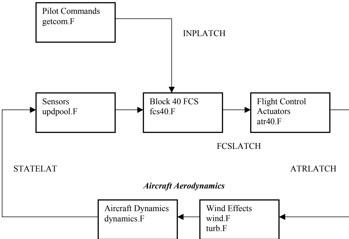
Figure 79: Original VISTA F-16 SRF Algorithm
