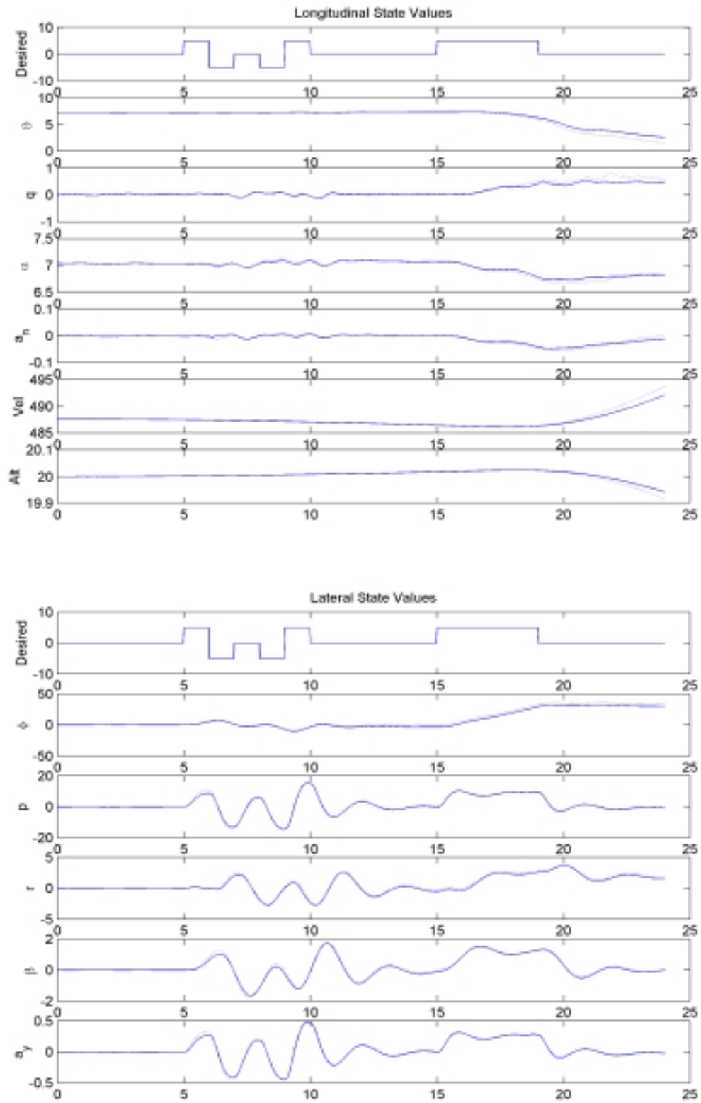
Figure 66c: State Values, Left Flaperon Failure, \epsilon = 25\% Using \epsilon_{\text{HAT}}
