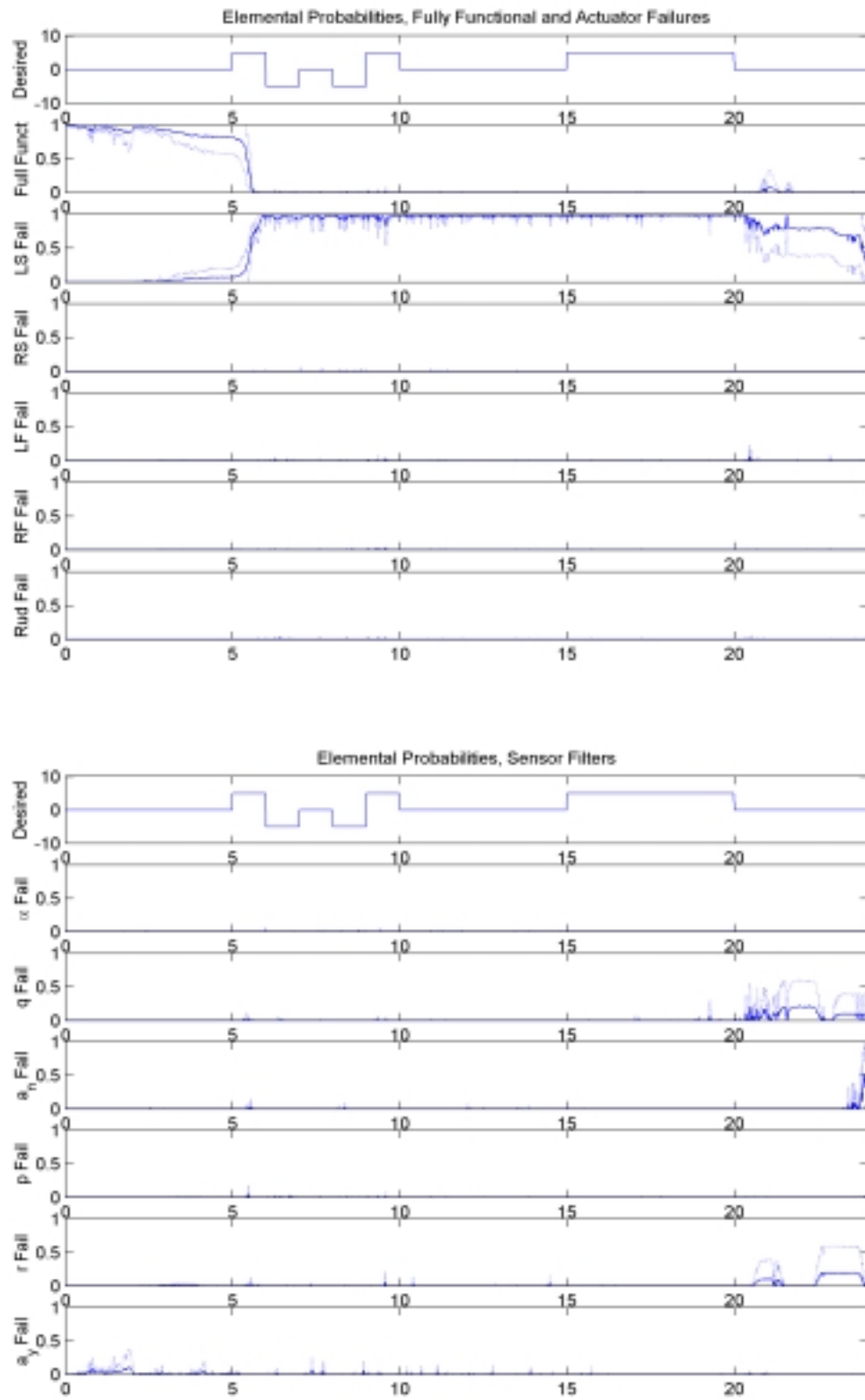
Figure 9a: Elemental Probabilities, Left Stabilator Failure, \epsilon = 0\%
