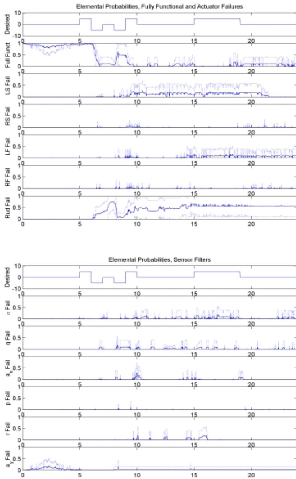
Figure 27a: Elemental Probabilities, Rudder Failure, \epsilon = 50\%
