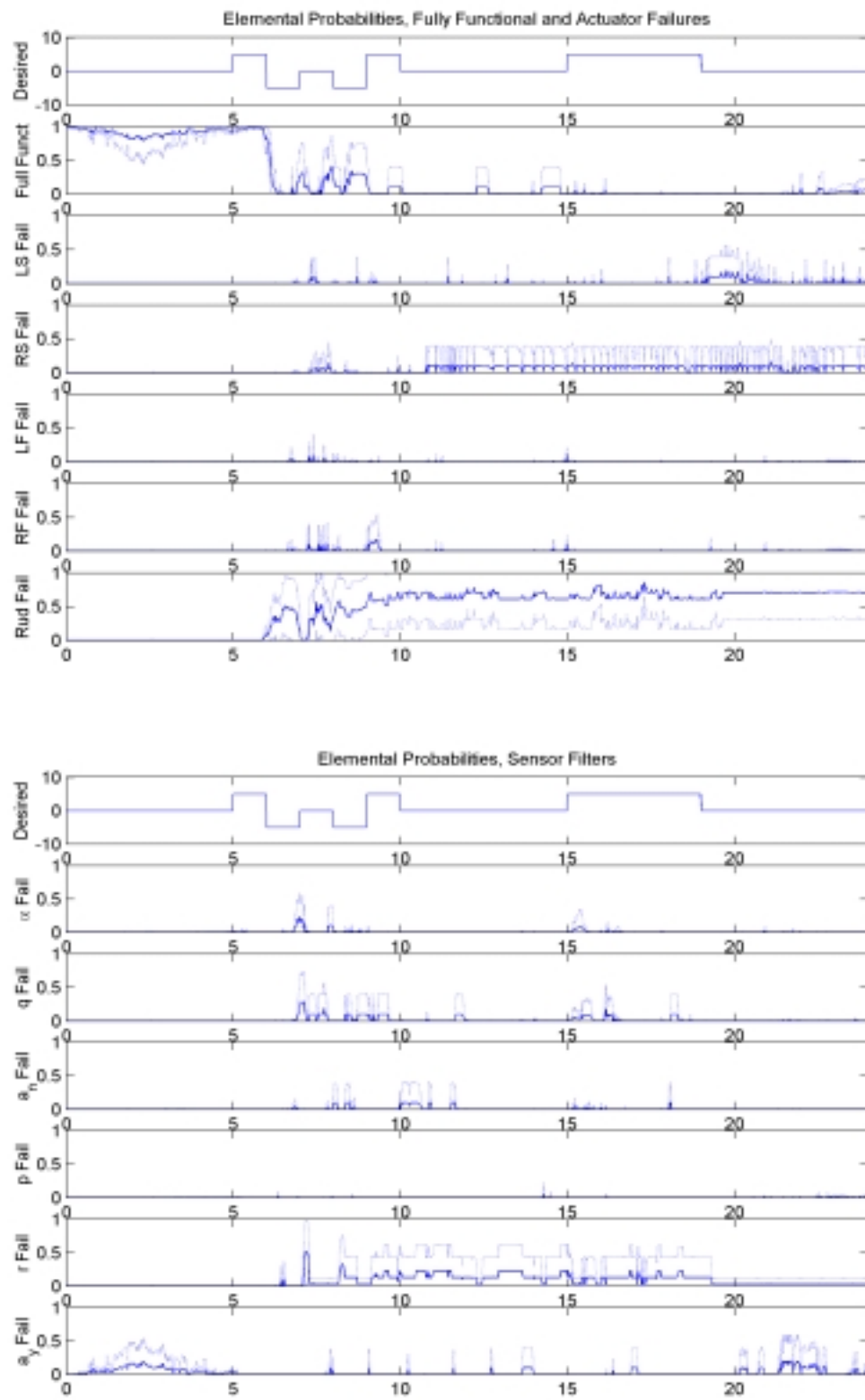
Figure 26a: Elemental Probabilities, Rudder Failure, \epsilon = 25\%
