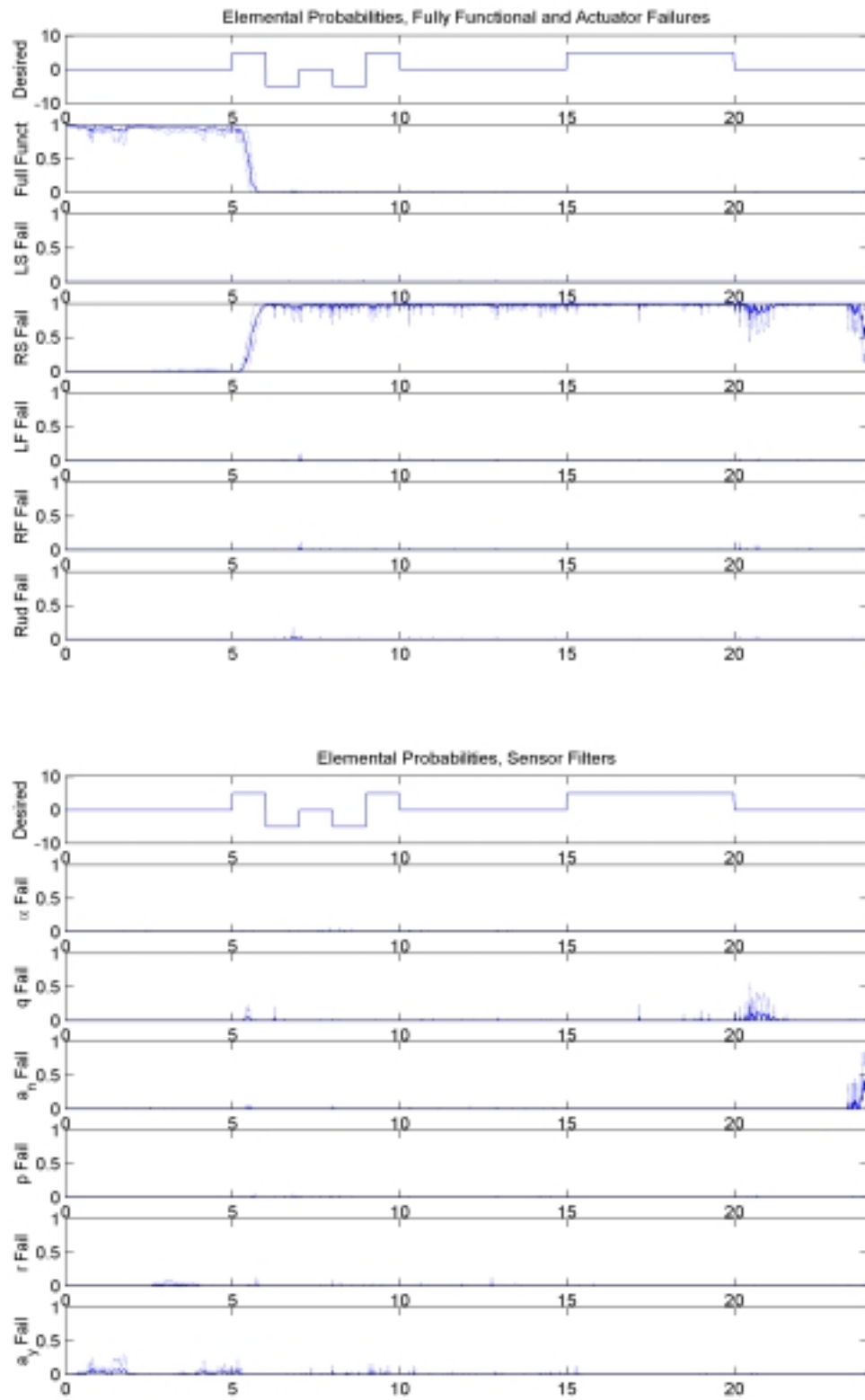
Figure 13a: Elemental Probabilities, Right Stabilator Failure, \epsilon = 0\%
