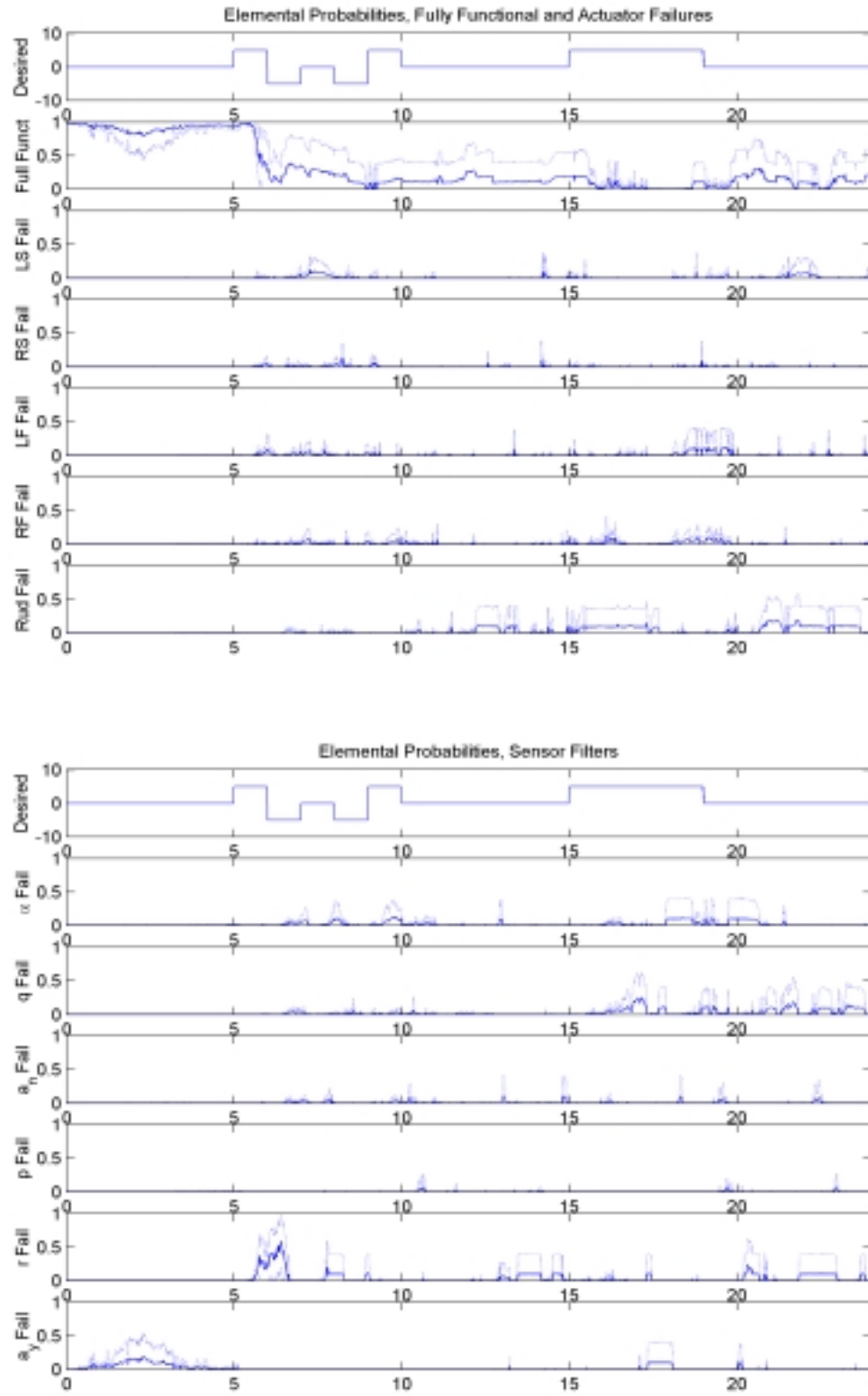
Figure 68a: Elemental Probabilities, Left Flaperon Failure, \epsilon = 75\% Using \epsilon_{\text{HAT}}
