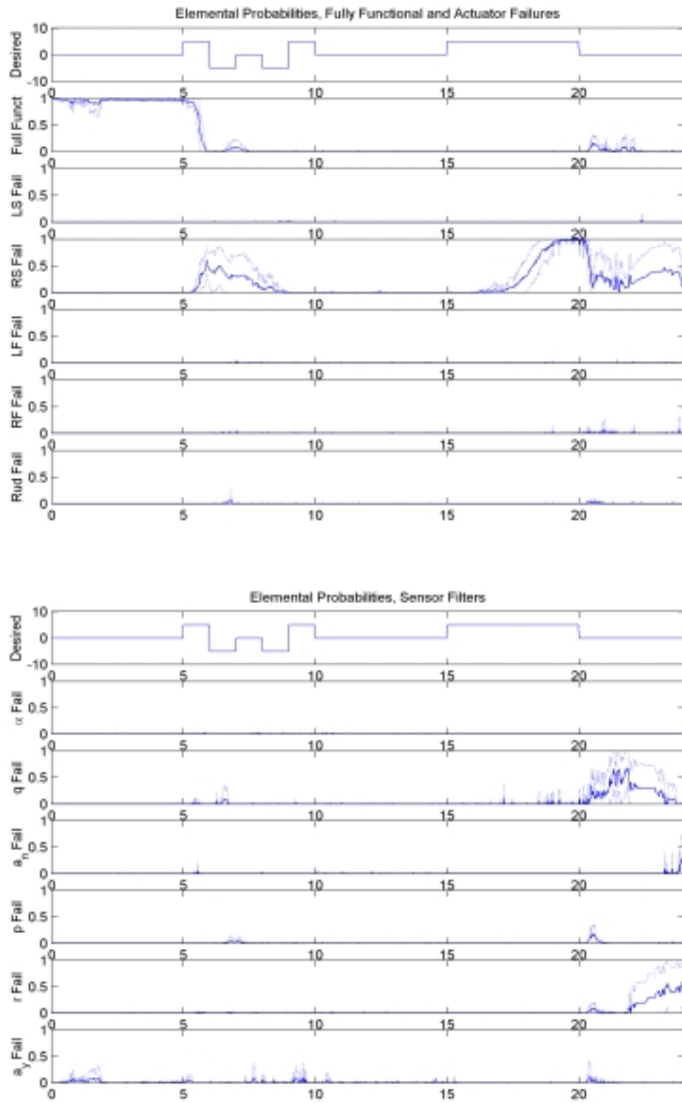
Figure 14a: Elemental Probabilities, Right Stabilator Failure, \epsilon = 25\%
