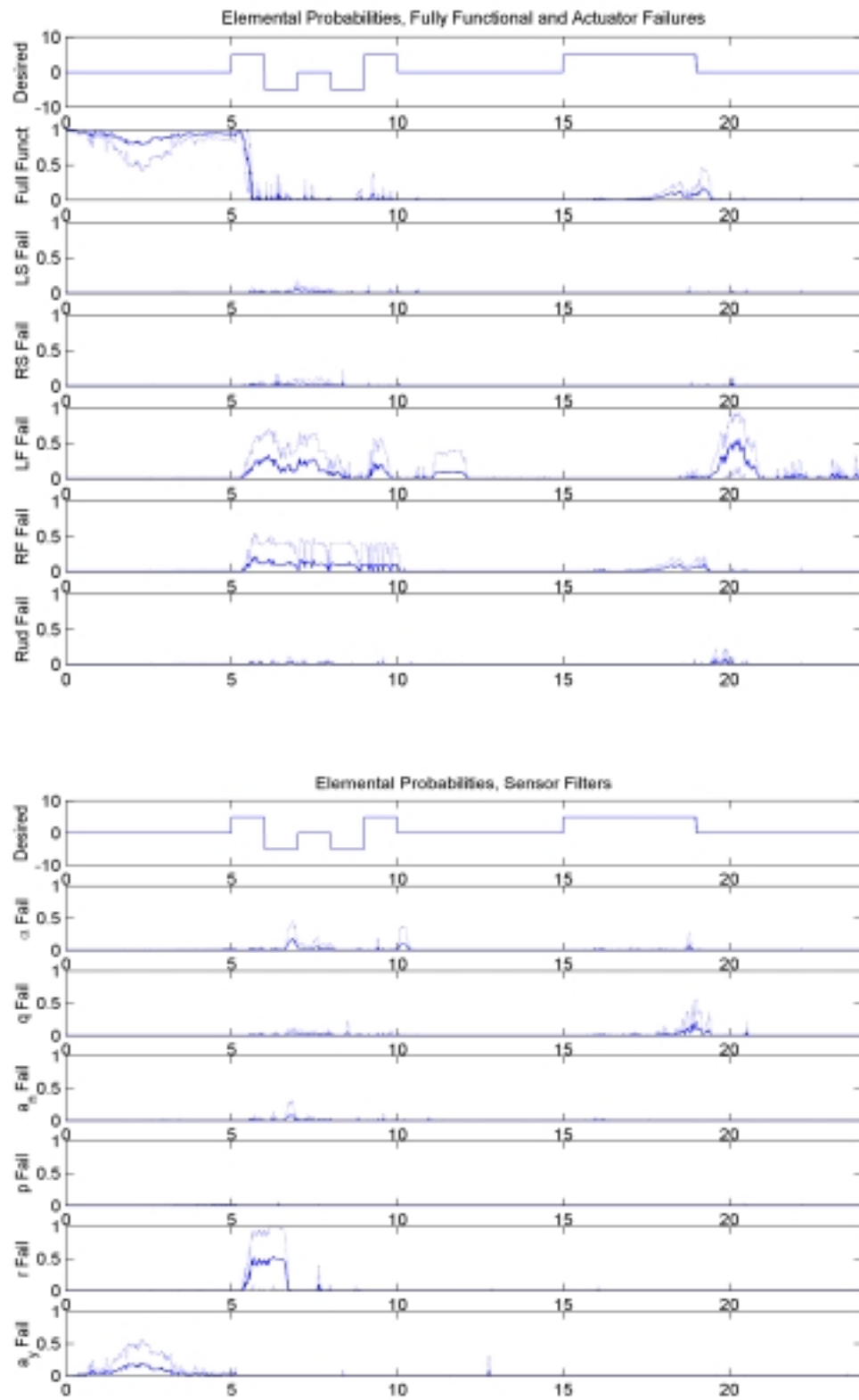
Figure 66a: Elemental Probabilities, Left Flaperon Failure, \epsilon = 25\% Using \epsilon_{\text{HAT}}
