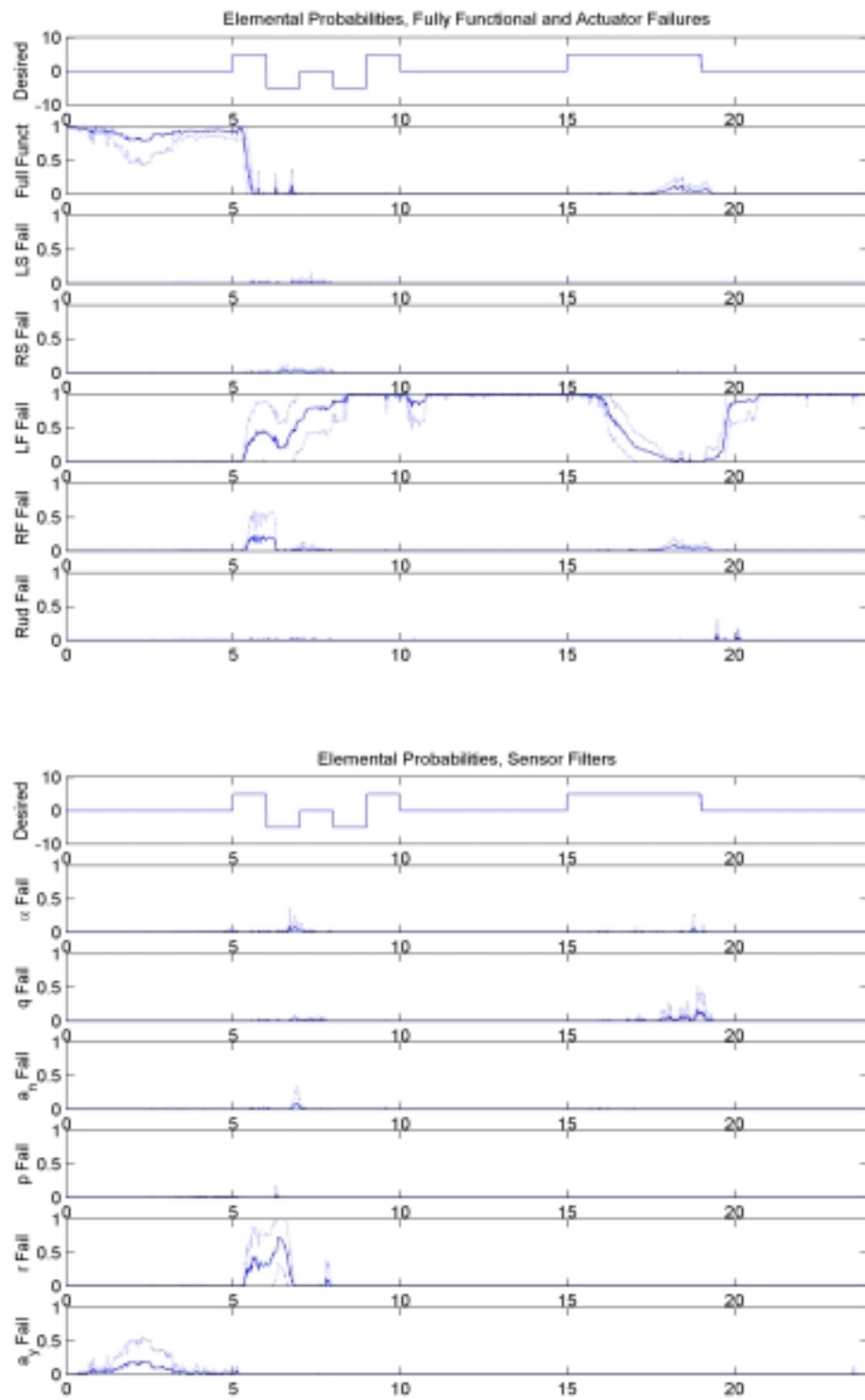
Figure 17a: Elemental Probabilities, Left Flaperon Failure, \epsilon = 0\%
