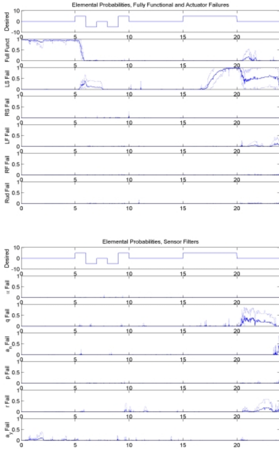
Figure 58a: Elemental Probabilities, Left Stabilator Failure, \epsilon = 25\% Using \epsilon_{\text{HAT}}
