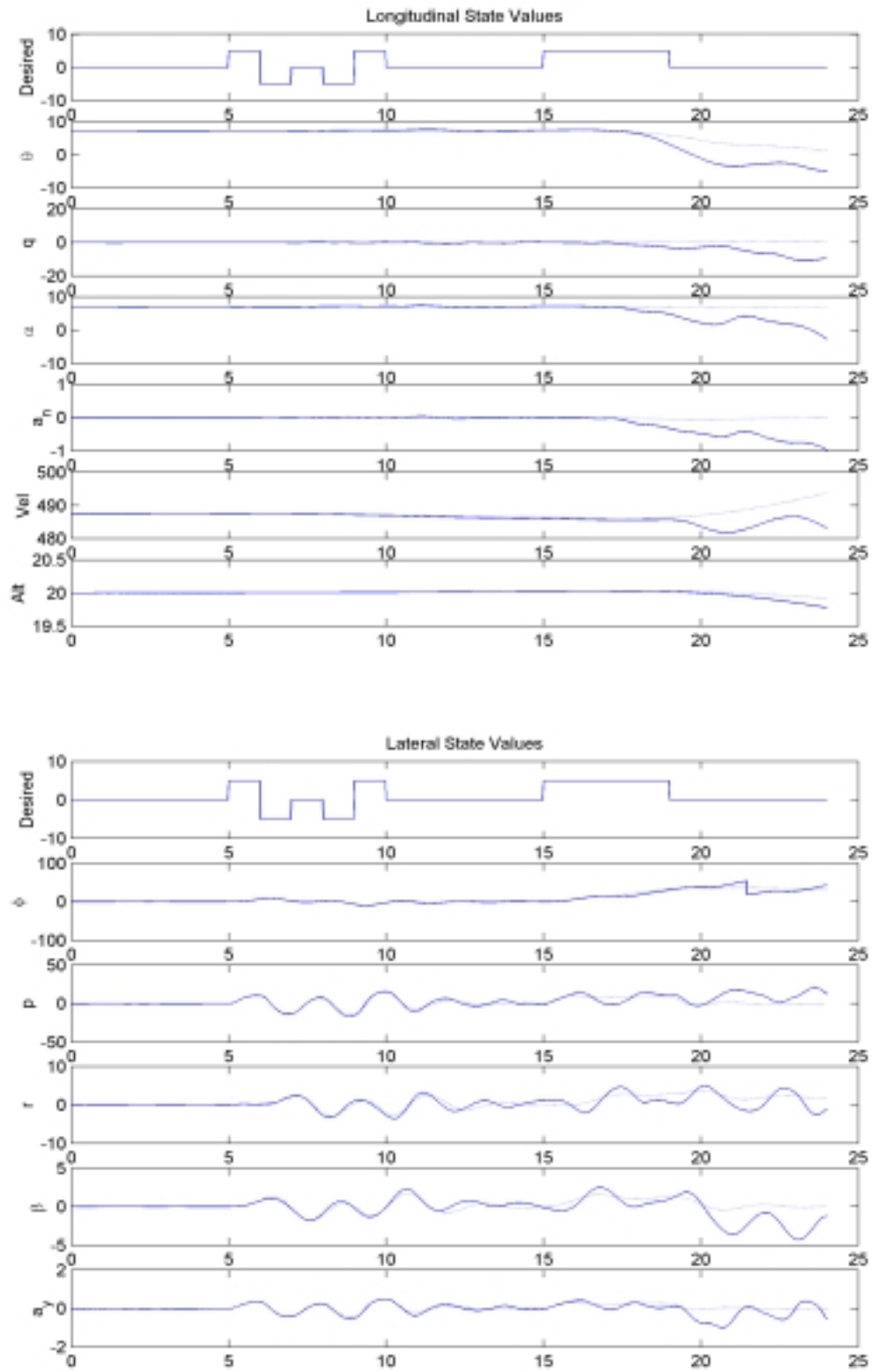
Figure 76c: State Values, Rudder Failure, \epsilon = 75\% Using \epsilon_{\text{HAT}}
