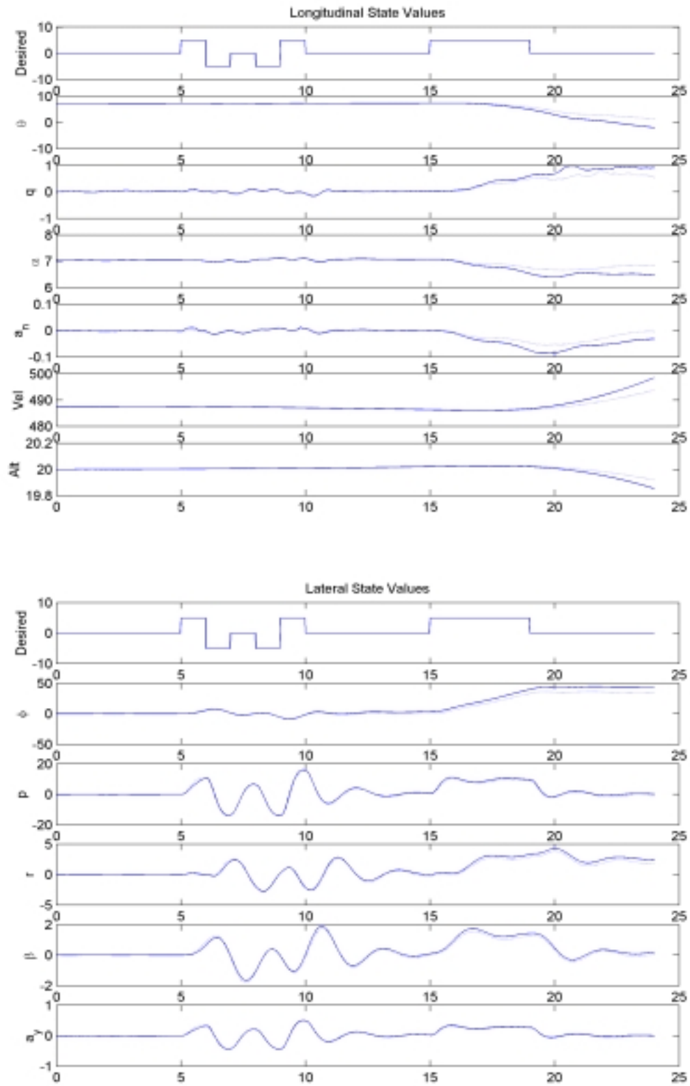
Figure 70c: State Values, Right Flaperon Failure, \epsilon = 25\% Using \epsilon_{\text{HAT}}
