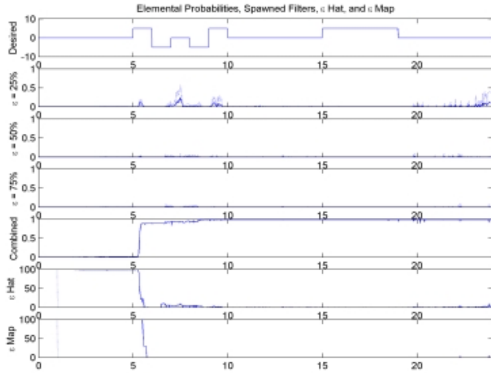
Figure 21b: Elemental Probabilities, Right Flaperon Failure, \epsilon = 0\%
