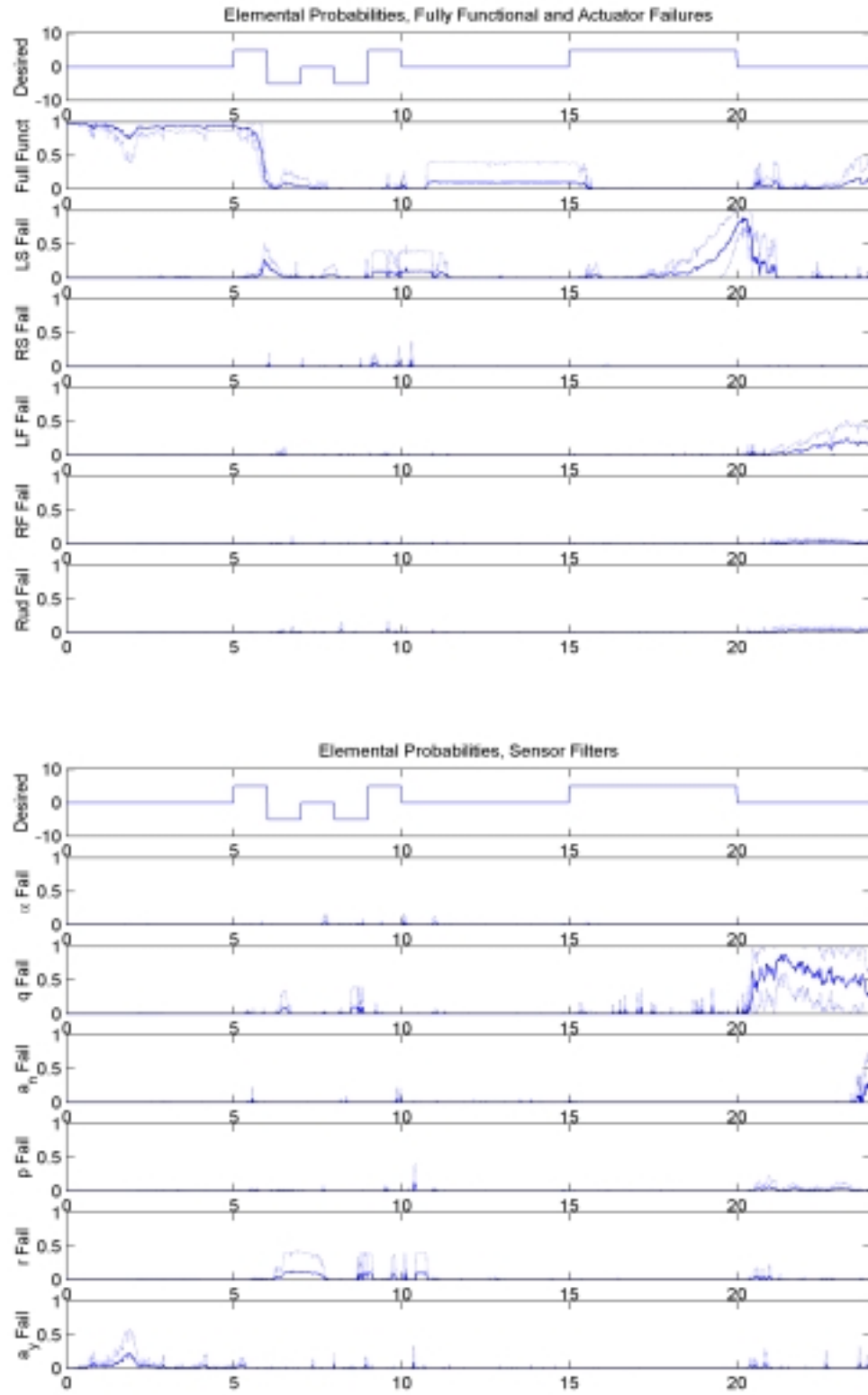
Figure 59a: Elemental Probabilities, Left Stabilator Failure, \epsilon = 50\% Using \epsilon_{\text{HAT}}
