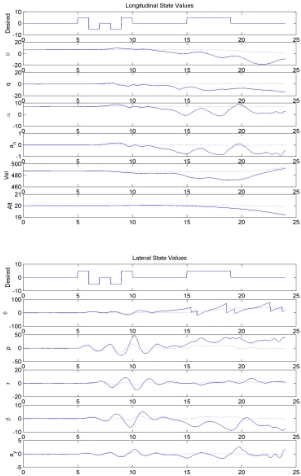
Figure 75c: State Values, Rudder Failure, \epsilon = 50\% Using \epsilon_{\text{HAT}}
