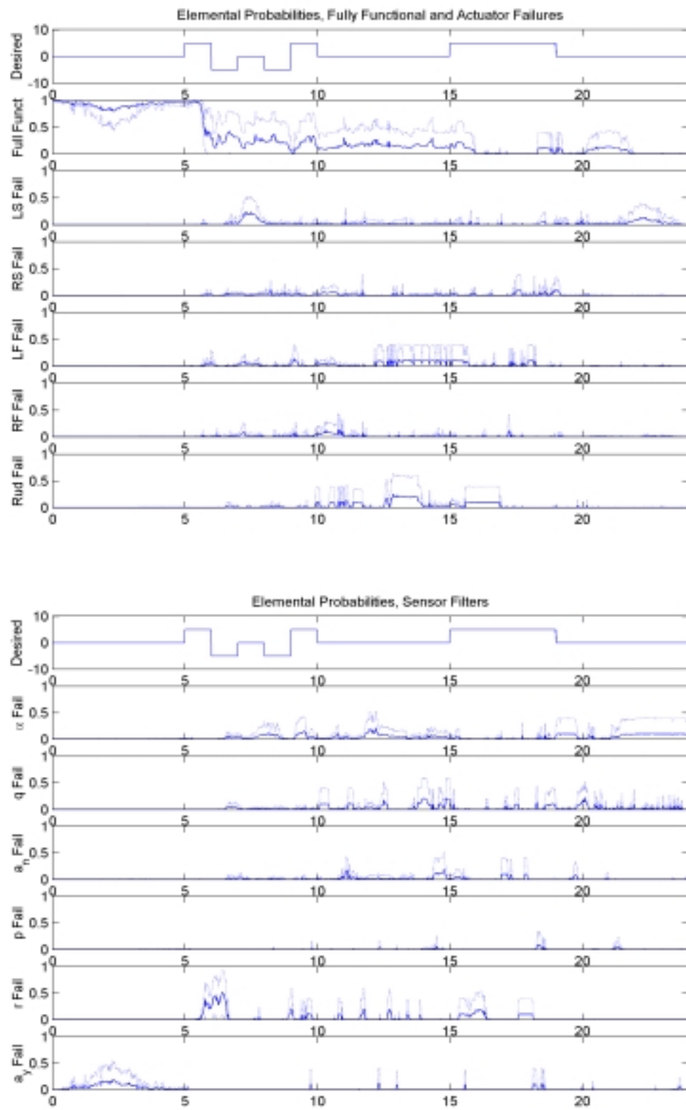
Figure 24a: Elemental Probabilities, Right Flaperon Failure, \epsilon = 75\%
