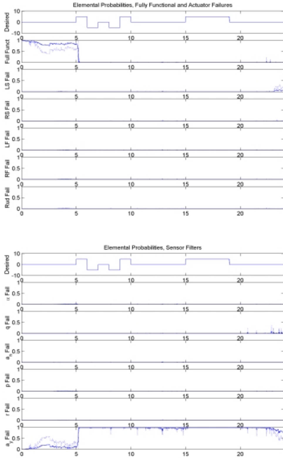
Figure 34: Elemental Probabilities, Lateral Acceleration Sensor Failure
