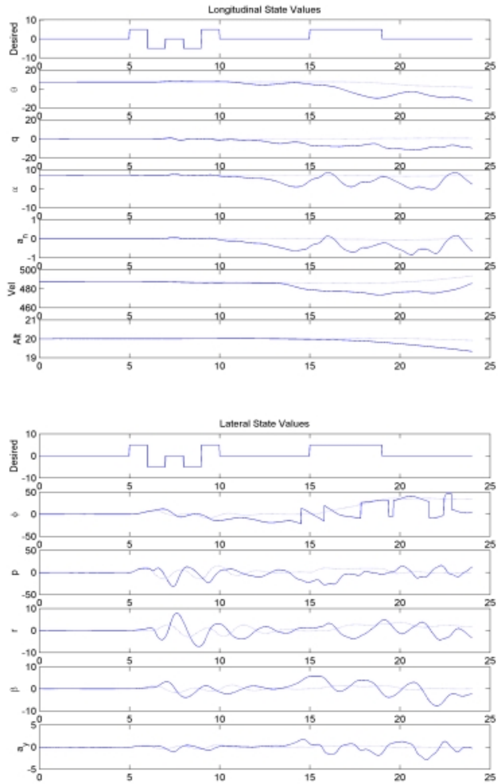
Figure 73c: State Values, Rudder Failure, \epsilon = 0\% Using \epsilon_{\text{HAT}}
