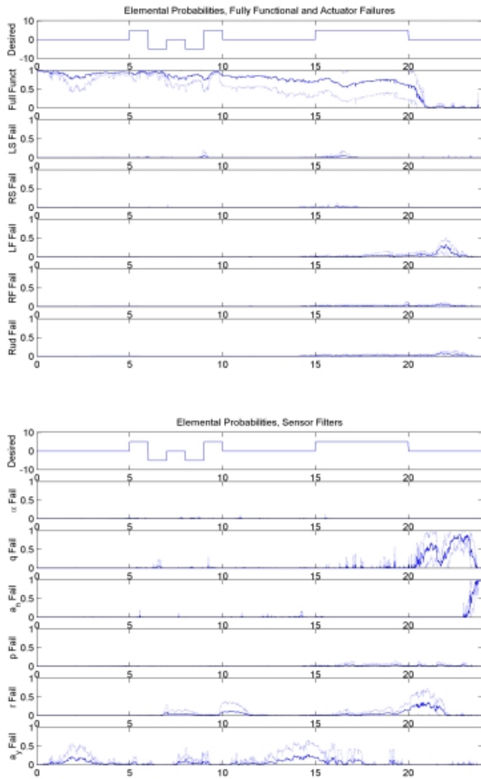
Figure 12a: Elemental Probabilities, Left Stabilator Failure, \epsilon = 75\%
