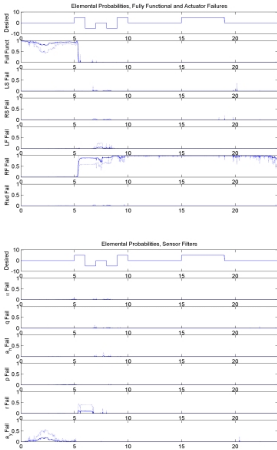
Figure 21a: Elemental Probabilities, Right Flaperon Failure, \epsilon = 0\%
