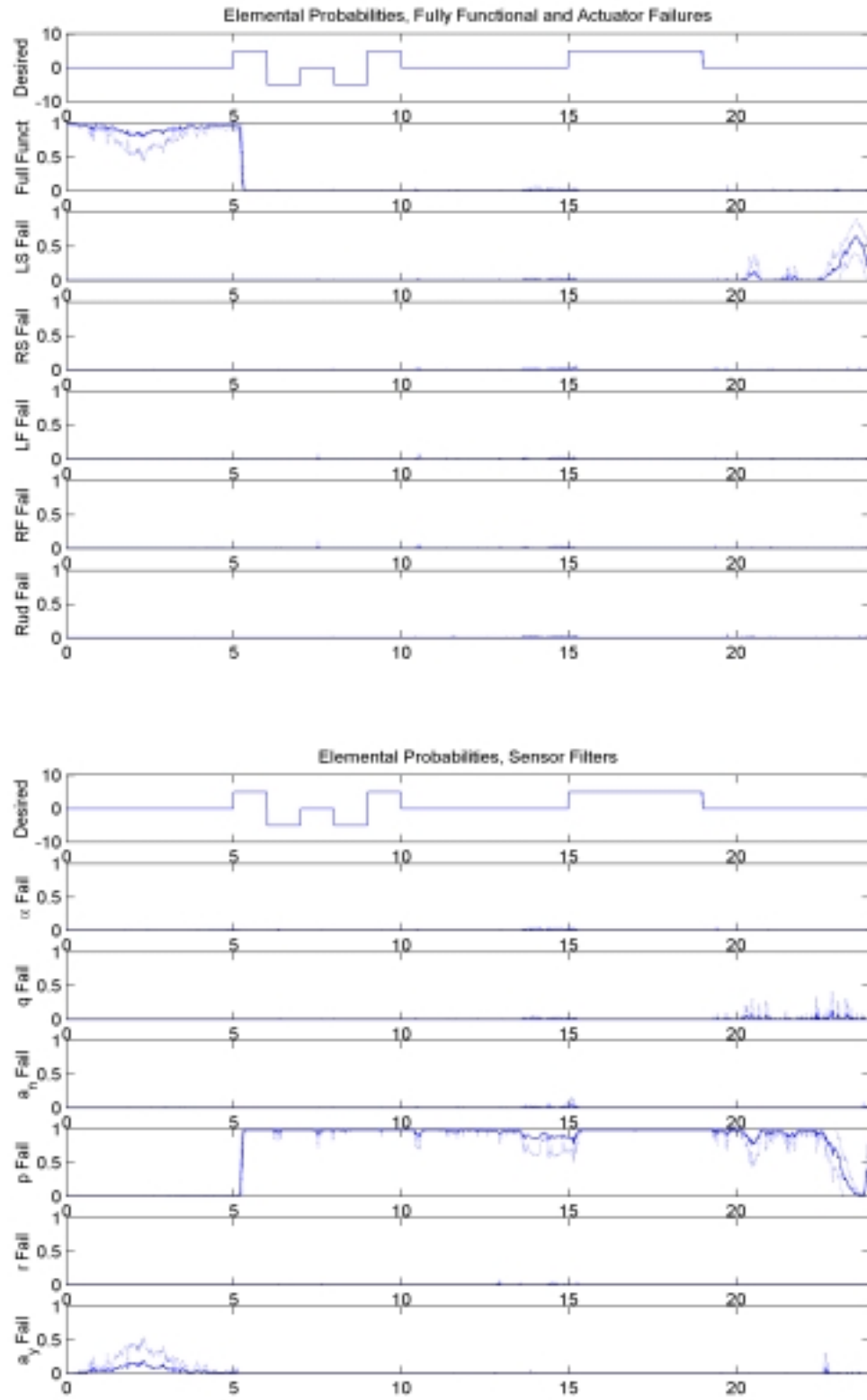
Figure 32: Elemental Probabilities, Roll Rate Sensor Failure
