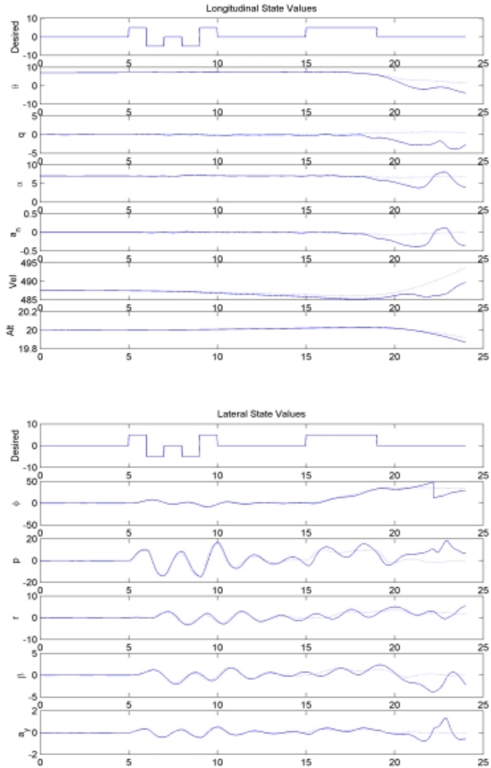
Figure 48: State Values, Left Flaperon Failure, \epsilon = 75\%
