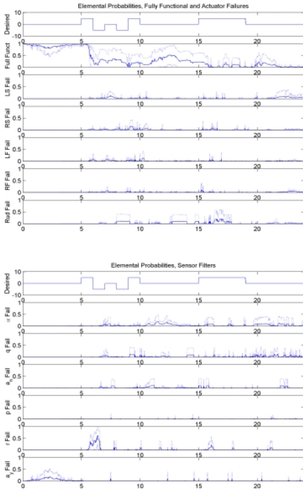
Figure 20a: Elemental Probabilities, Left Flaperon Failure, \epsilon = 75\%
