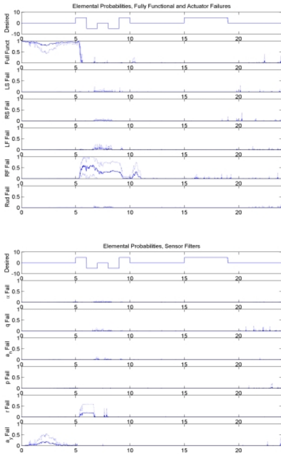
Figure 22a: Elemental Probabilities, Right Flaperon Failure, \epsilon = 25\%
