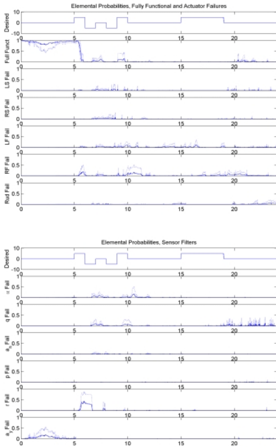
Figure 23a: Elemental Probabilities, Right Flaperon Failure, \epsilon = 50\%
