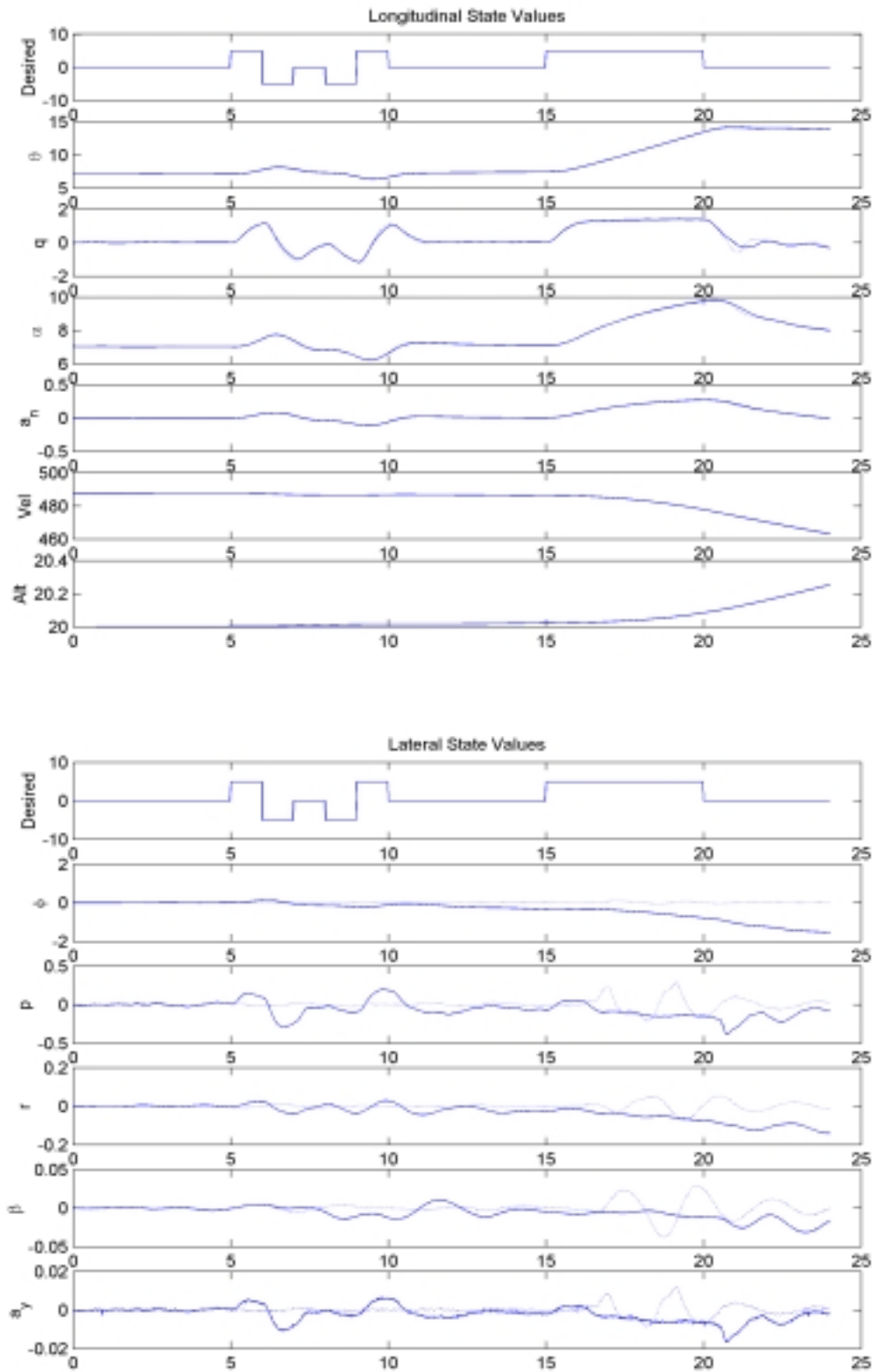
Figure 60c: State Values, Left Stabilator Failure, \epsilon = 75\% Using \epsilon_{\text{HAT}}
