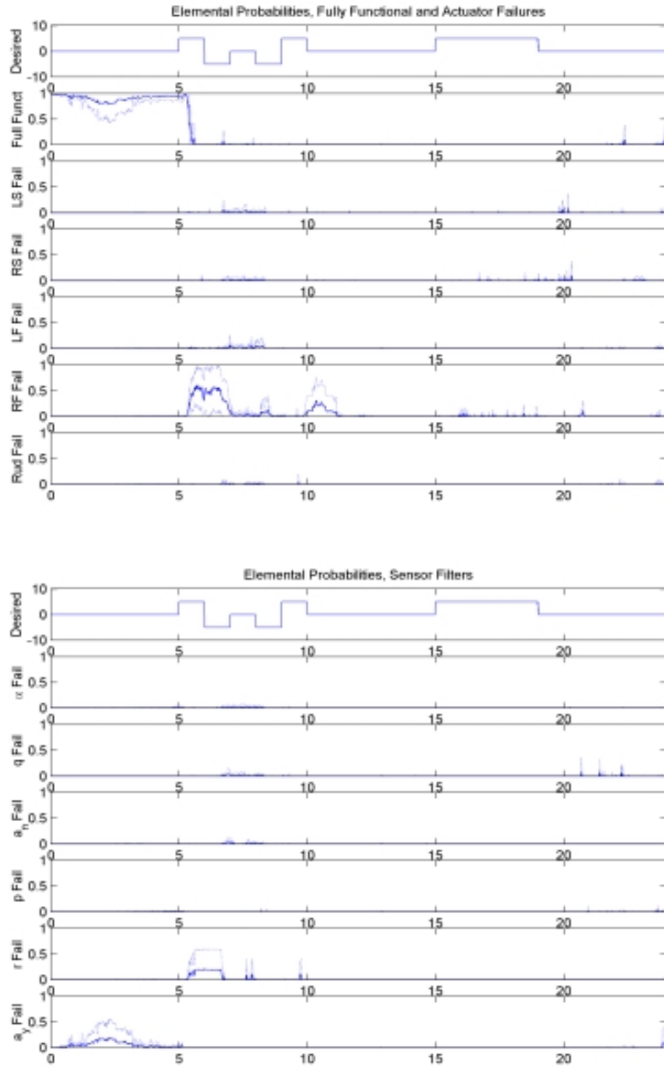
Figure 70a: Elemental Probabilities, Right Flaperon Failure, \epsilon = 25\% Using \epsilon_{\text{HAT}}
