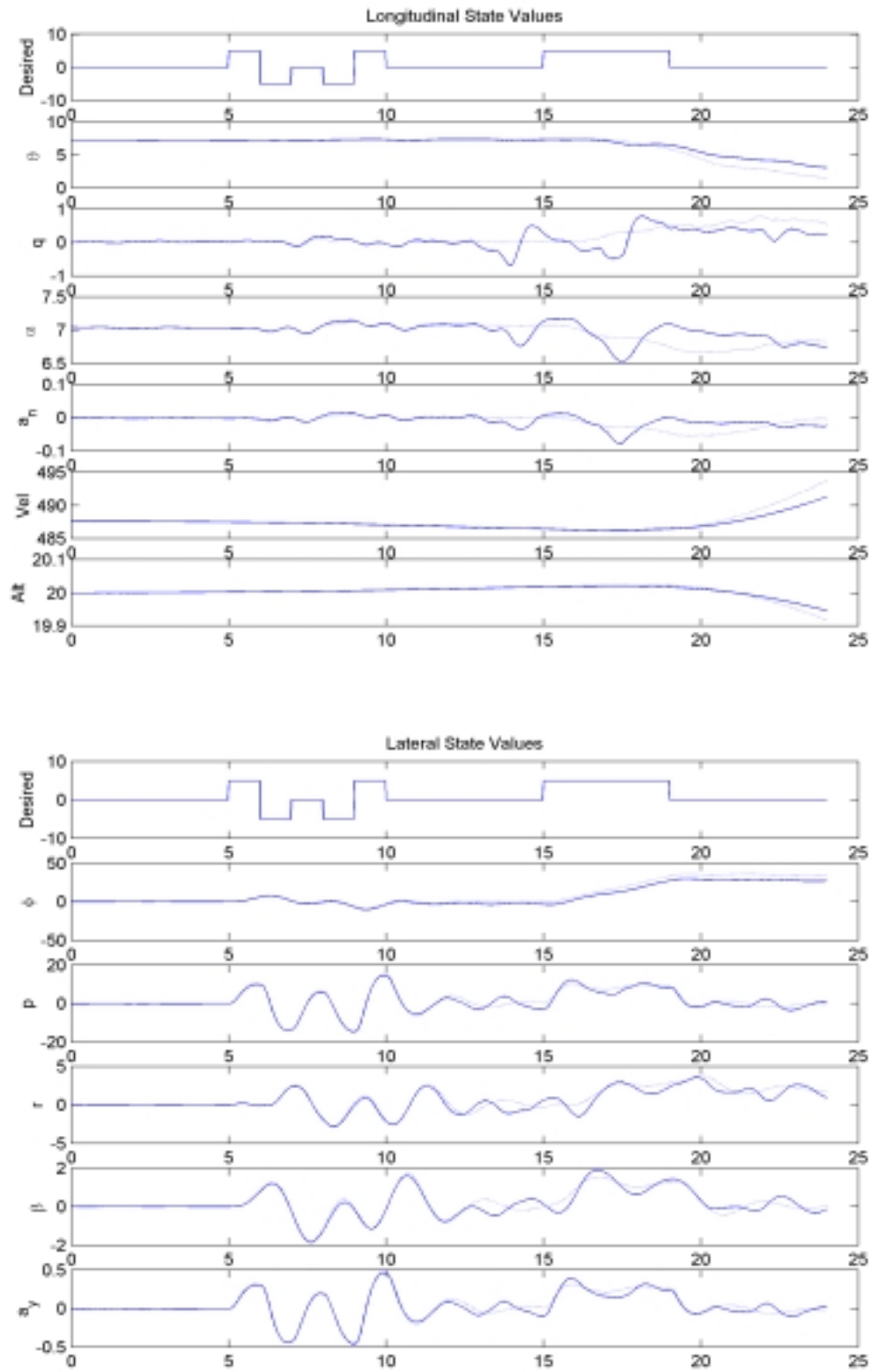
Figure 68c: State Values, Left Flaperon Failure, \epsilon = 75\% Using \epsilon_{HAT}
