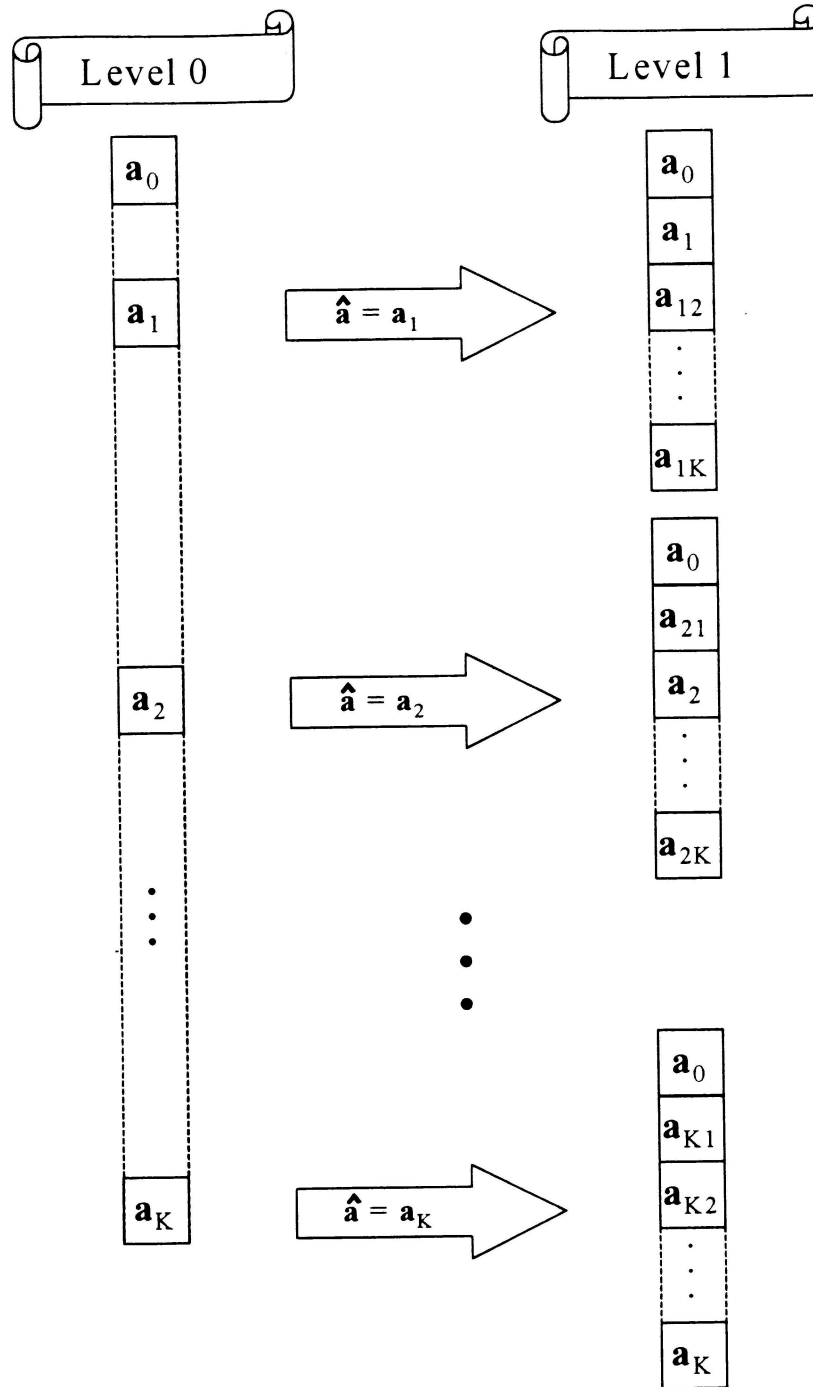
Figure 2: Hierarchical Structure [11]
