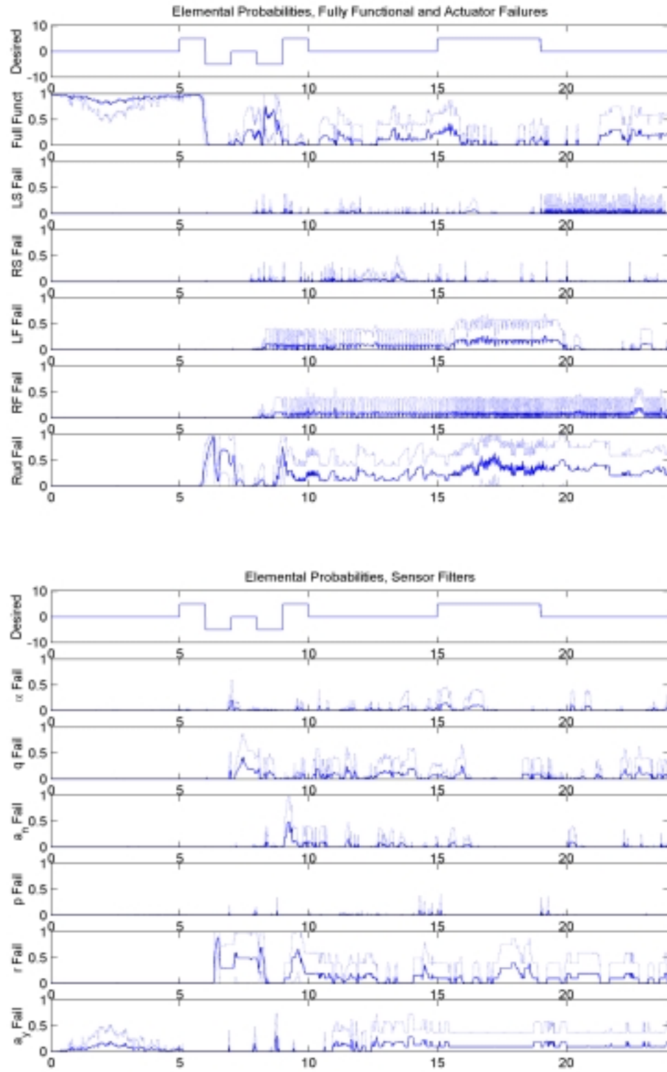
Figure 73a: Elemental Probabilities, Rudder Failure, \epsilon = 0\% Using \epsilon_{\text{HAT}}
