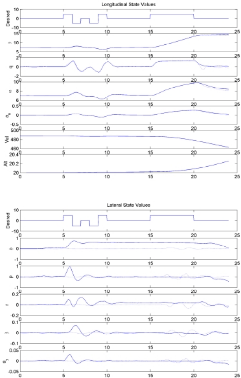
Figure 57c: State Values, Left Stabilator Failure, \epsilon = 0\% Using \epsilon_{\text{HAT}}
