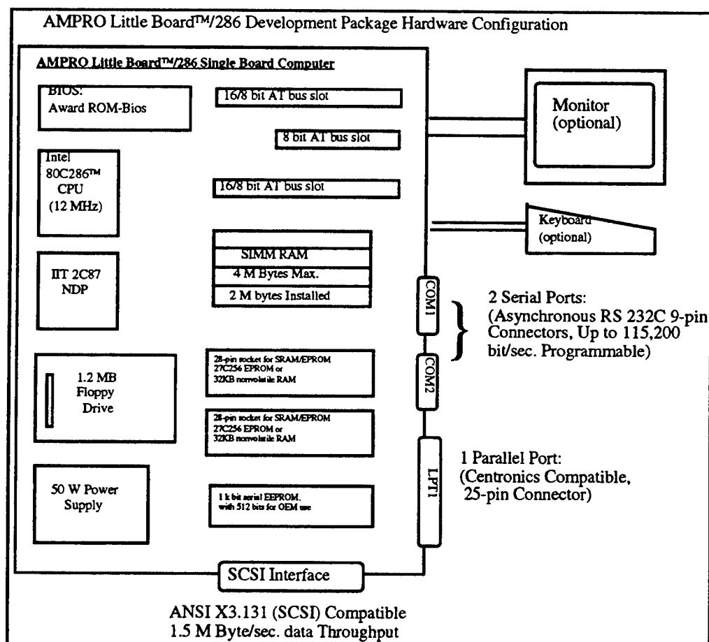
Figure 7: Local processor hardware configuration.
