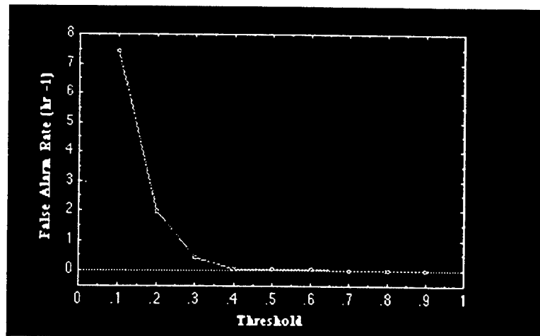
Figure 3.2: False Alarm Rate per Hour for Comma Events as a Function of Neural Network Threshold
