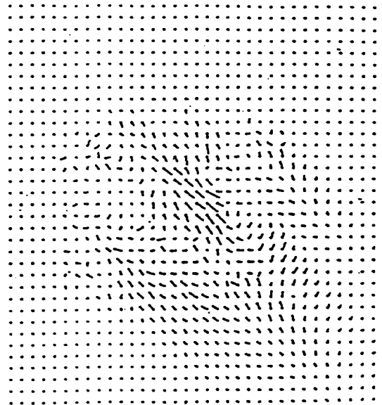
Figure 6.2: Results of Applying the Horn and Schunck's Algorithm on the same Random Dot Moving Pattern
