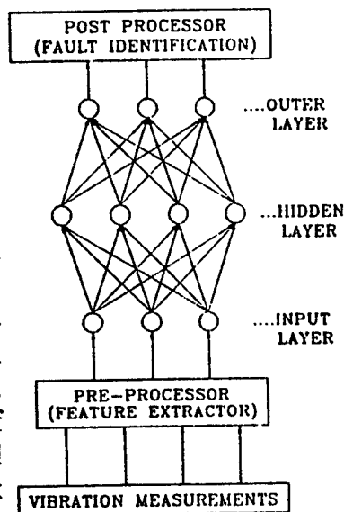
Fig. 2. Neural network architecture
