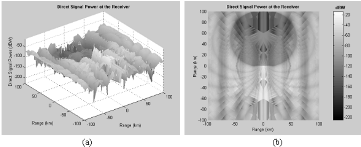
Figure 4.6 Received power of the direct signal, including the effects of the receiver antenna, assuming that the receiver can be located anywhere on the terrain
