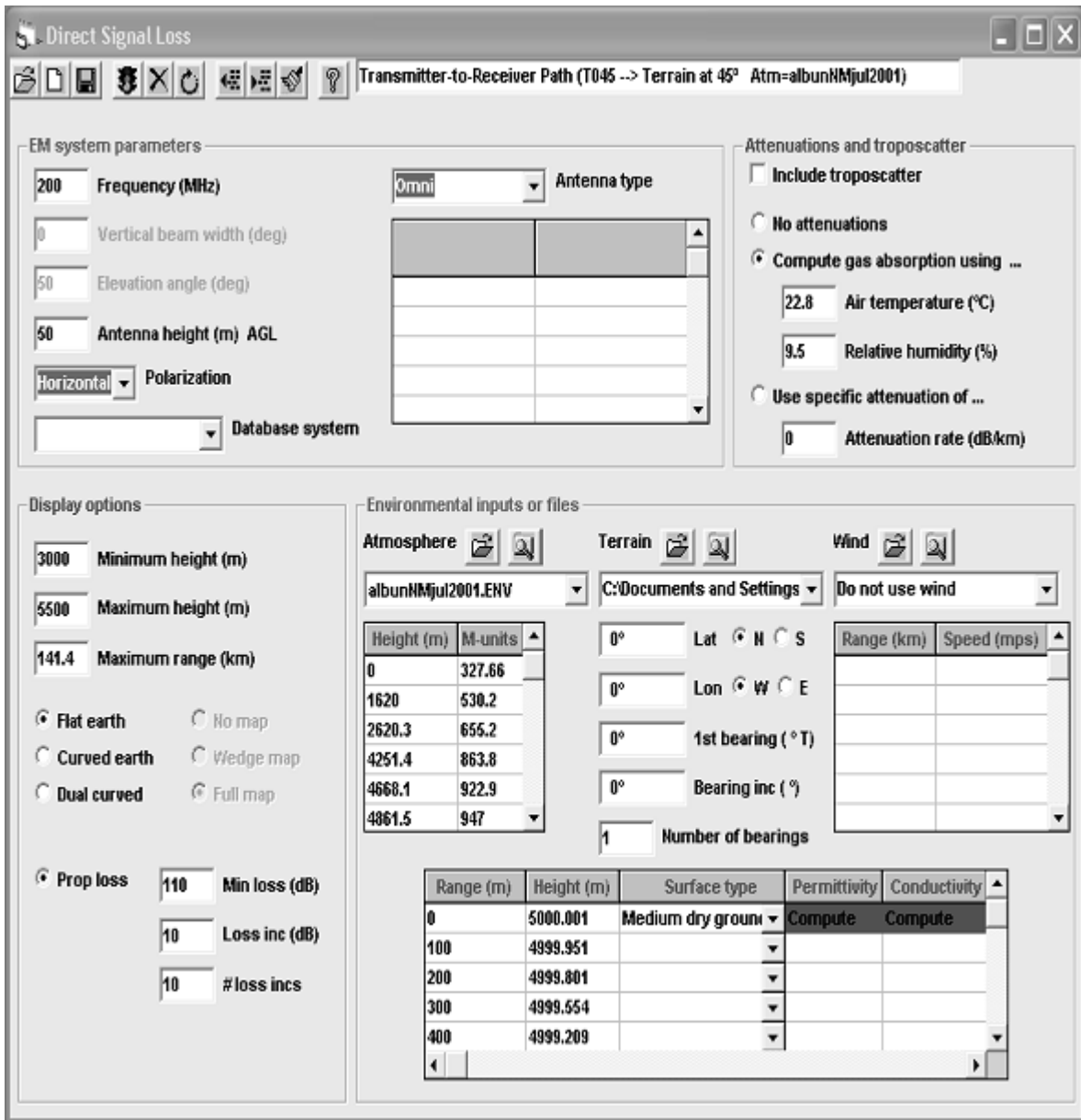
Figure 3.7 AREPS research window used to calculate the losses of the signal from the transmitter to every point in the terrain.
