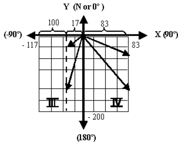
Figure 3.17 The new coordinate system, centered at the AOI, keeping the same terrain grid dimensions and the same values on the elevation matrix \mathbf{Z} . Also shown on the scheme is a representation of the vectors on the directions the new terrain files will be defined.
