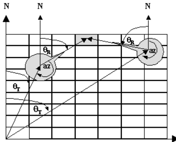
Figure 3.15 Geometry to calculate the angle of the antenna pattern (on gray), with respect to the maximum direction of gain, az , by calculating the angle of arrival of the direct signal to the antenna pattern and the antenna pointing angle of the direct signal, both with respect to the North reference axis.
