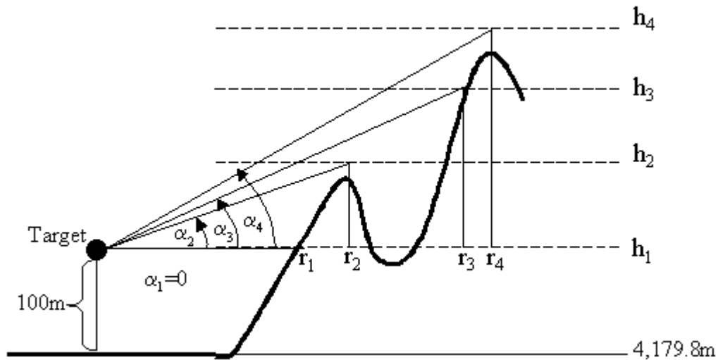
Figure 3.19 Calculating the Object-to-Receiver path at a particular bearing. By predefining a set of heights h_1, h_2, h_3, and h_4 is possible to calculate the ranges r_1, r_2, r_3, and r_4 and therefore the elevation angles \alpha_1, \alpha_2, \alpha_3, and \alpha_4
