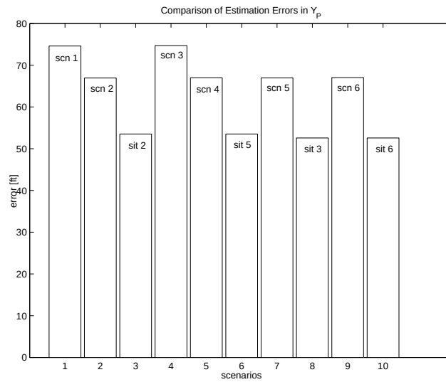
Figure 4.25 Y_P - Geo-location - Case 2: Comparison of Scenarios
