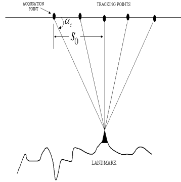
Figure A.1 Nominal tracking sequence.
