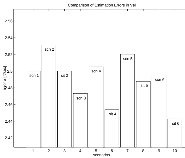
Figure 4.26 Velocity Estimation - Case 2: Comparison of Scenarios
