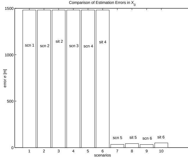
Figure 4.27 Own-ship X -Position Estimate - Case 3: Comparison of Scenarios
