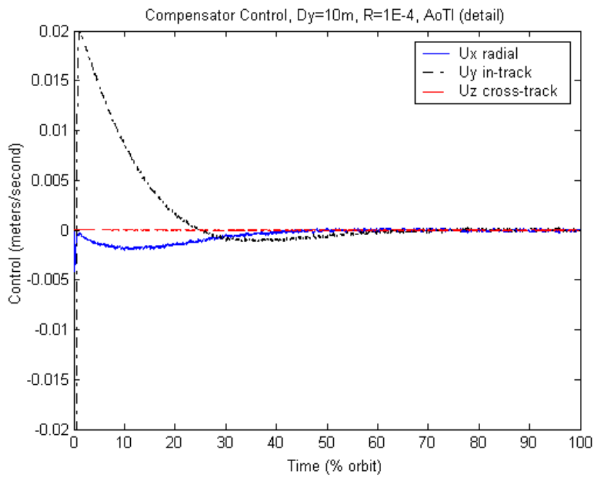
Figure 75. Compensator Control for R=1\text{E-}4 , D_y=10\text{m} , AoTI
