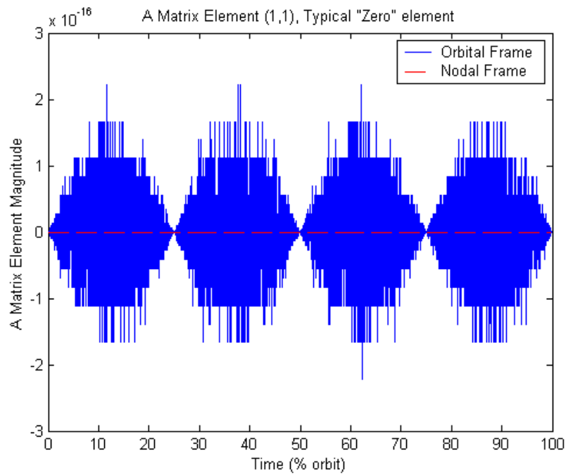
Figure 10. A Matrix Element (1,1) Comparisons, Typical “Zero” Element
