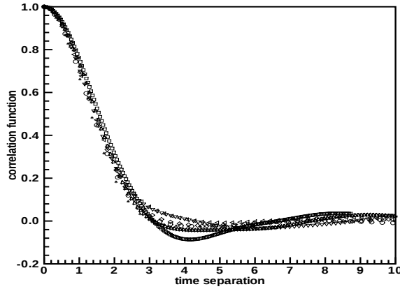
FIG. 1.1. Time correlation function at various wavenumbers plotted as functions of the similarity variable \xi = Vk\tau . The thick curve with the lowest minimum corresponds to a low wavenumber; increasing wavenumber corresponds to increasing \psi(\xi) at \xi = 4 .
