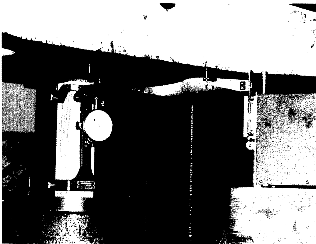
Figure 17. Axial compression test with deformation gauge.
