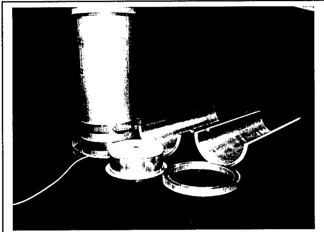
Figure 6. SBIR Analog Casting Tooling
