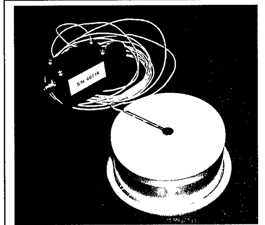
Figure 7. Sensor Installed in Insulation
