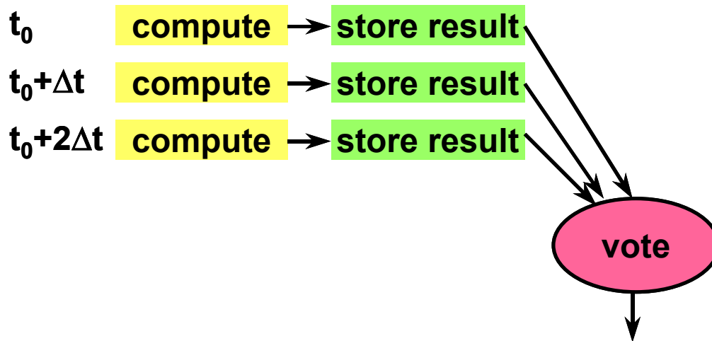
Figure 11. Time Redundancy [DEC99]
