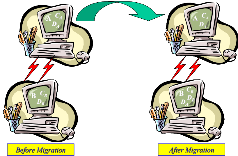
Figure 1. Client/Server Functionality
