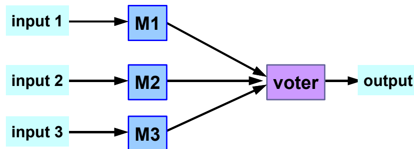
Figure 6. Triple Modular Redundancy before error detection [DEC99]
